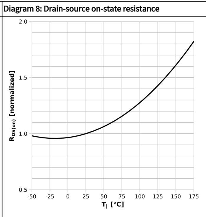
R_{DS(on)}=f(T_j); I_D=27.0 \text{ A}; V_{GS}=18 \text{ V}
