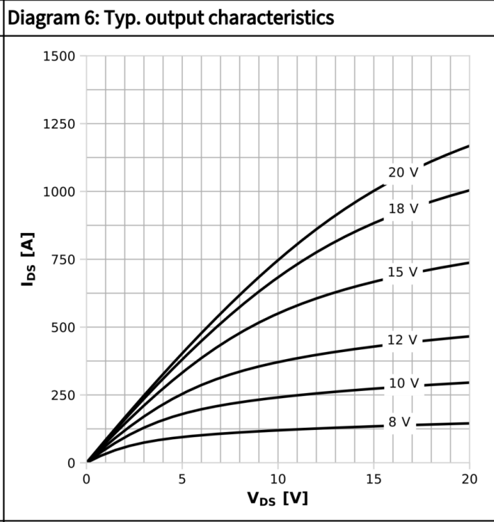
I_{DS}=f(V_{DS}); T_j=175^{\circ}\text{C}; \text{parameter: } V_{GS}
