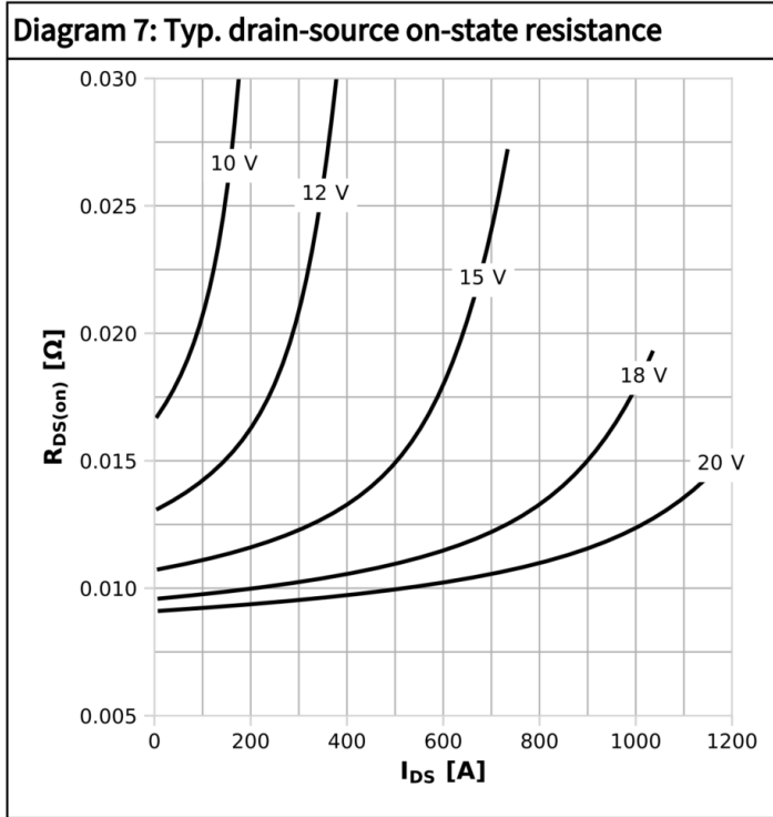
R_{DS(on)}=f(I_{DS}); T_j=125^{\circ}\text{C}; \text{parameter: } V_{GS}
