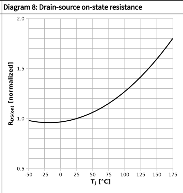
R_{DS(on)}=f(T_j); I_D=126.0 \text{ A}; V_{GS}=18 \text{ V}
