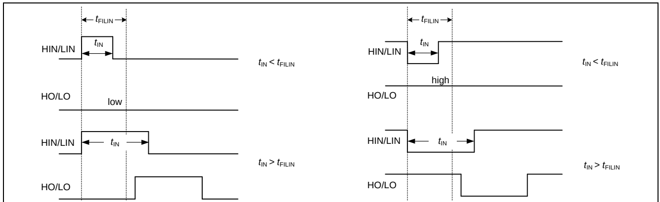
Figure 10 Timing of short pulse suppression (6EDL04I06PC, 6EDL04N06PC)
