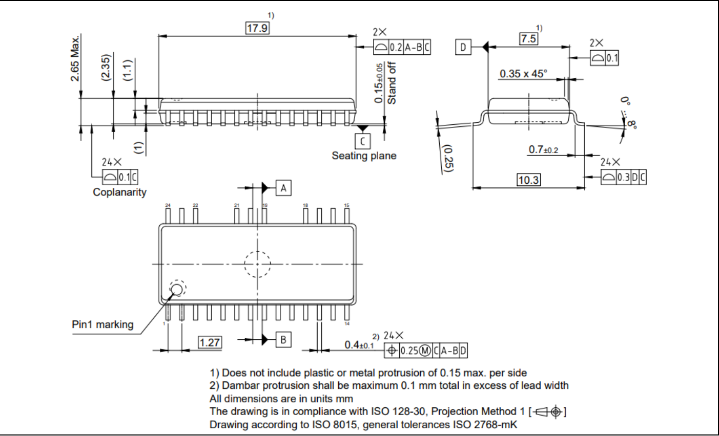
Figure 29 Package outline
