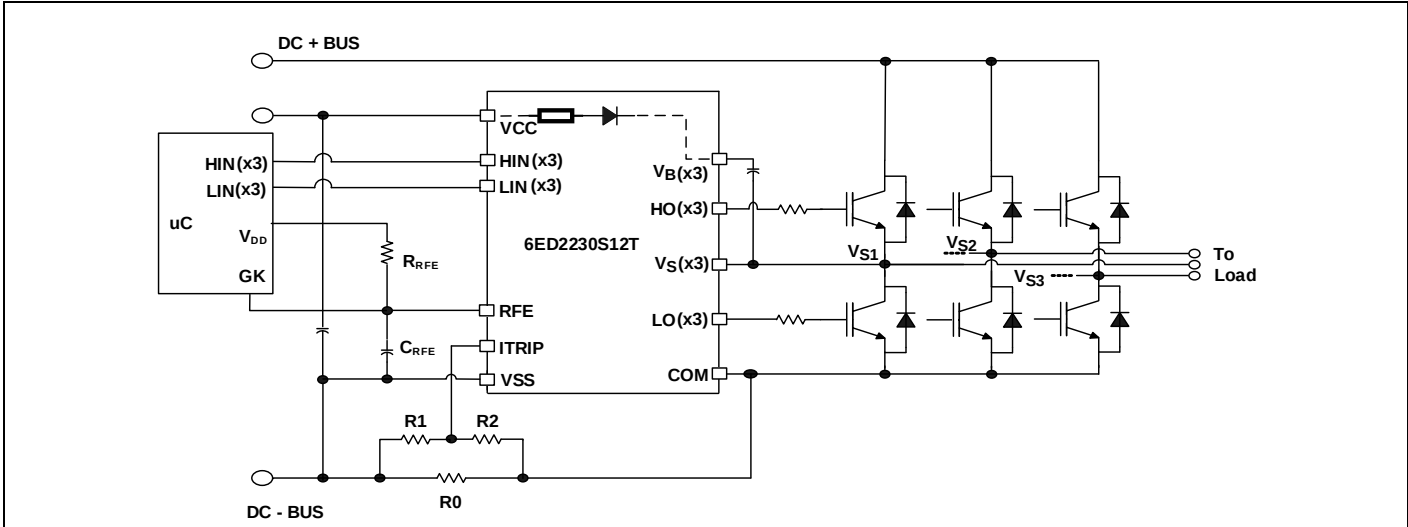
Figure 15 Programming the fault clear timer
