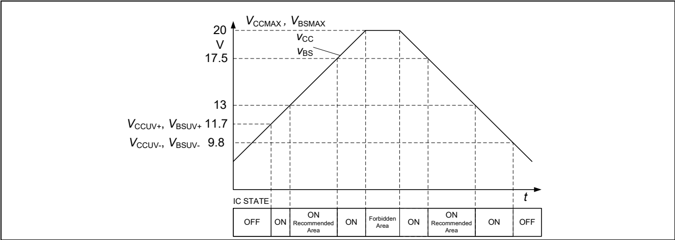
Figure 12 Operating areas
