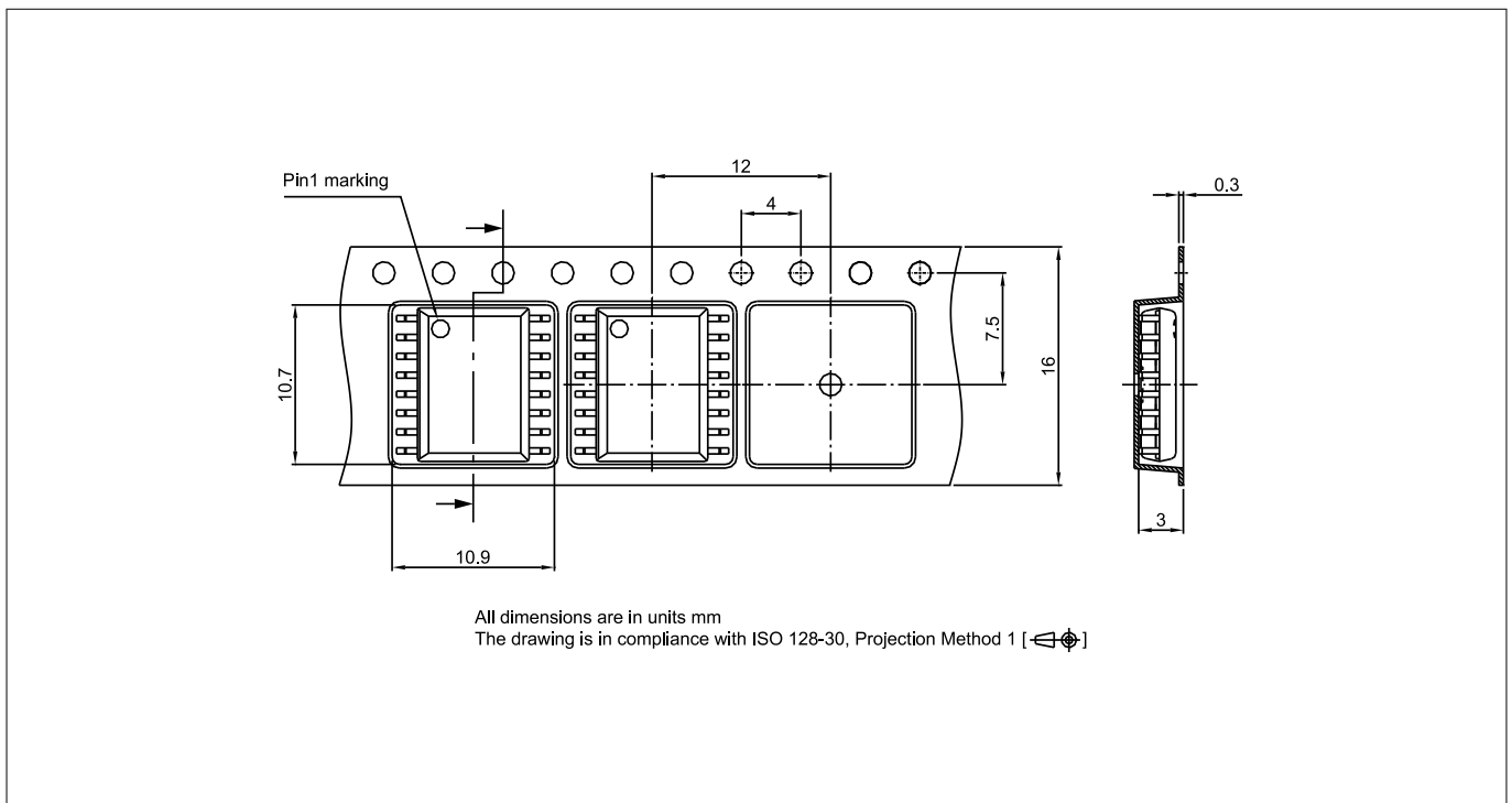
Figure 24 DSO16-300mil packing
