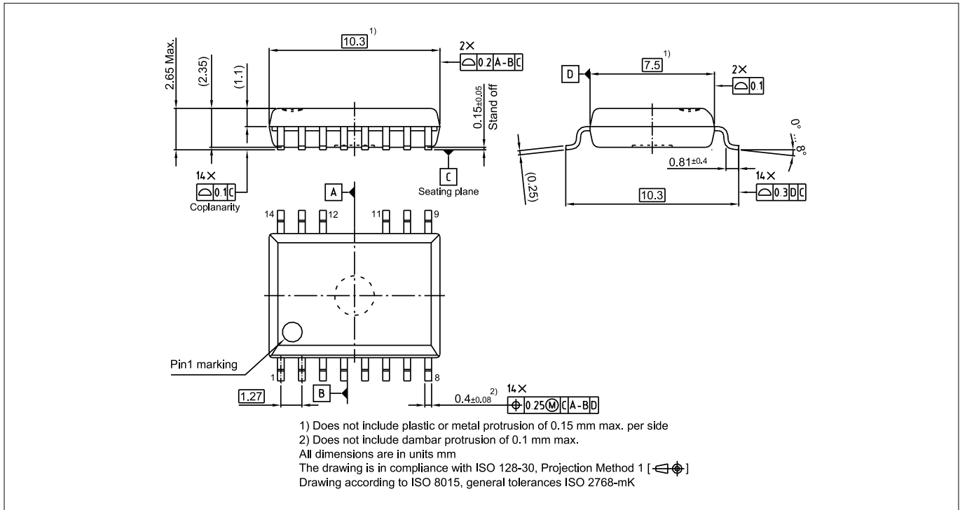
Figure 25 DSO14-300mil outline
