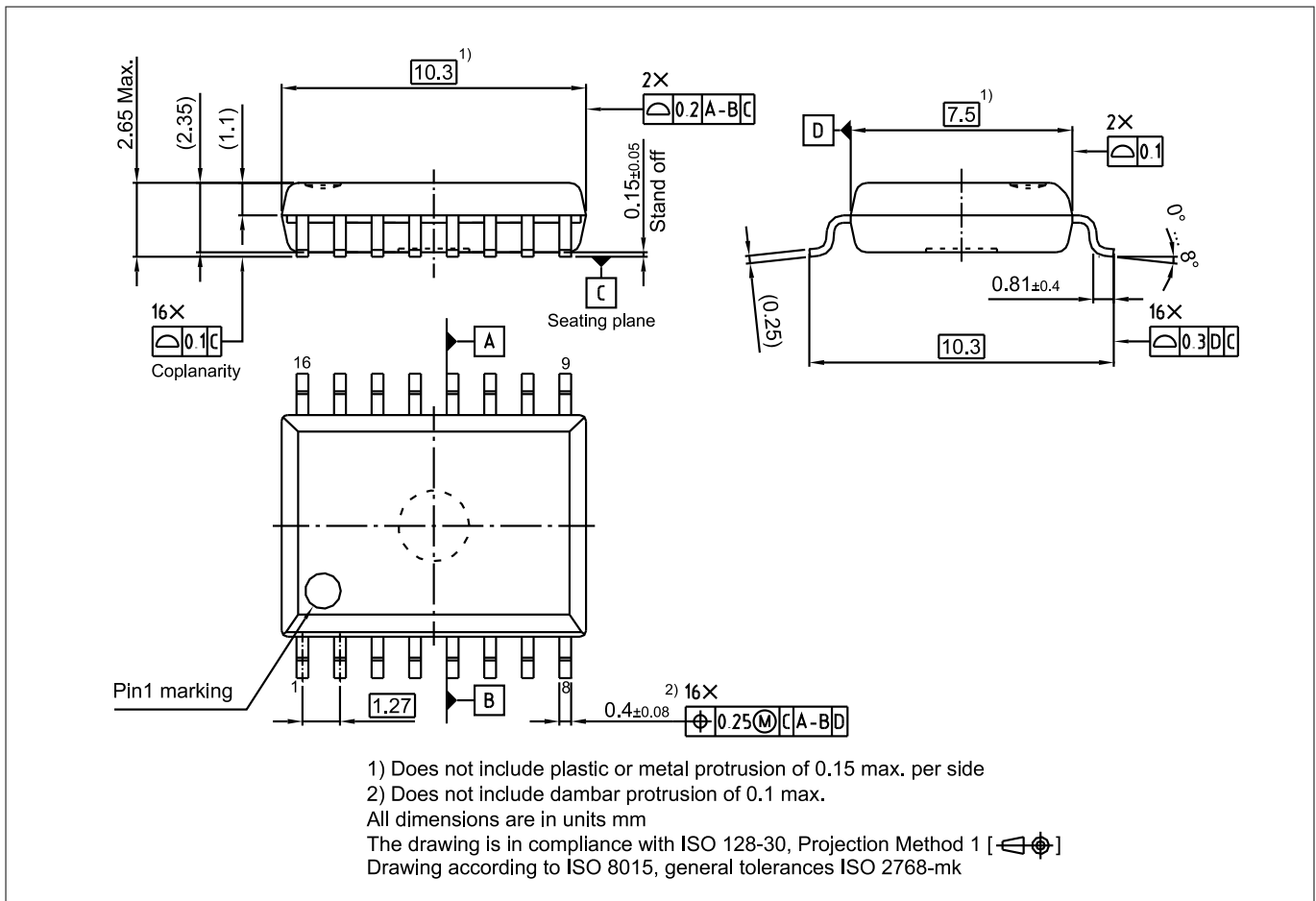
Figure 22 DSO16-300mil outline
