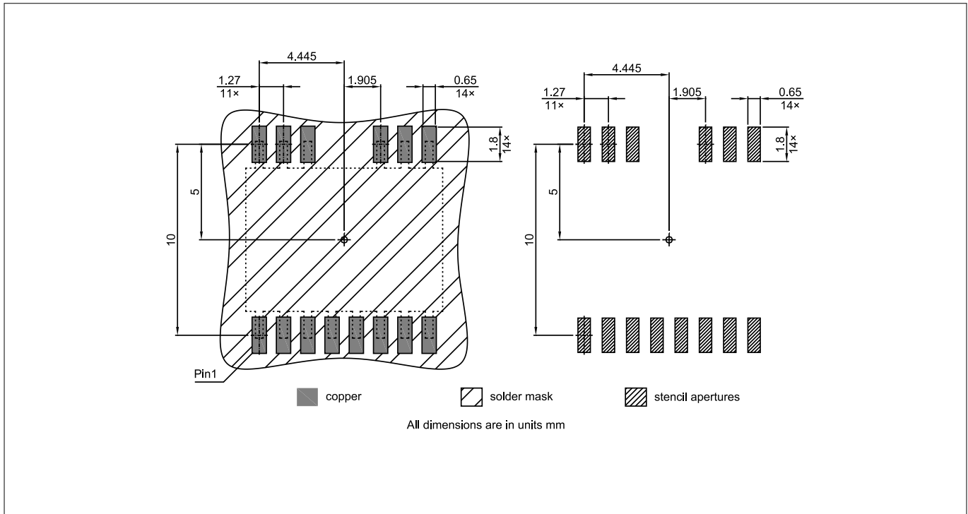
Figure 26 DSO14-300mil footprint
