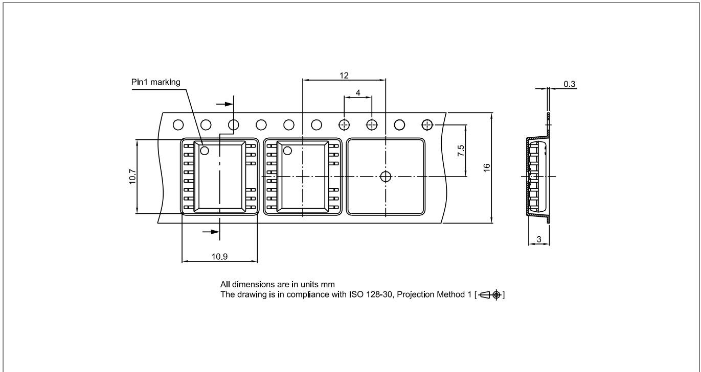
Figure 27 DSO14-300mil packing
