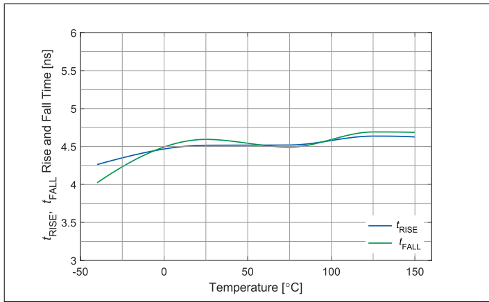
Figure 20 t_{\text{RISE}} & t_{\text{fall}} vs. temperature
