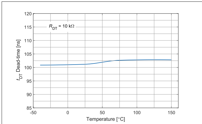
Figure 22 t_{\text{DT}} vs. temperature
