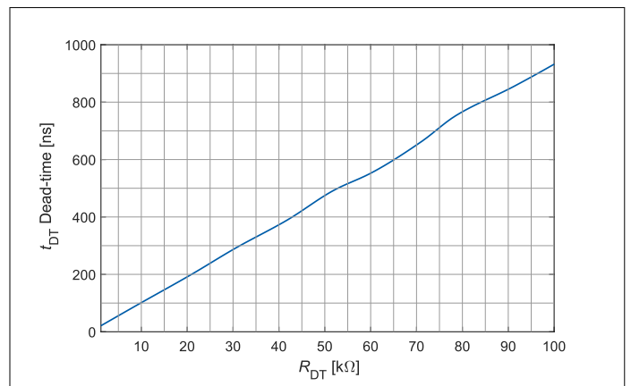
Figure 25 t_{\text{DT}} vs. R_{\text{DT}}
