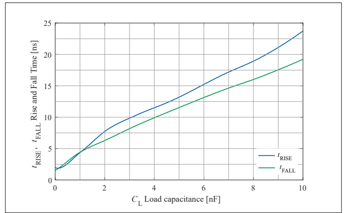
Figure 21 t_{\text{RISE}} & t_{\text{fall}} vs. C_{\text{LOAD}}
