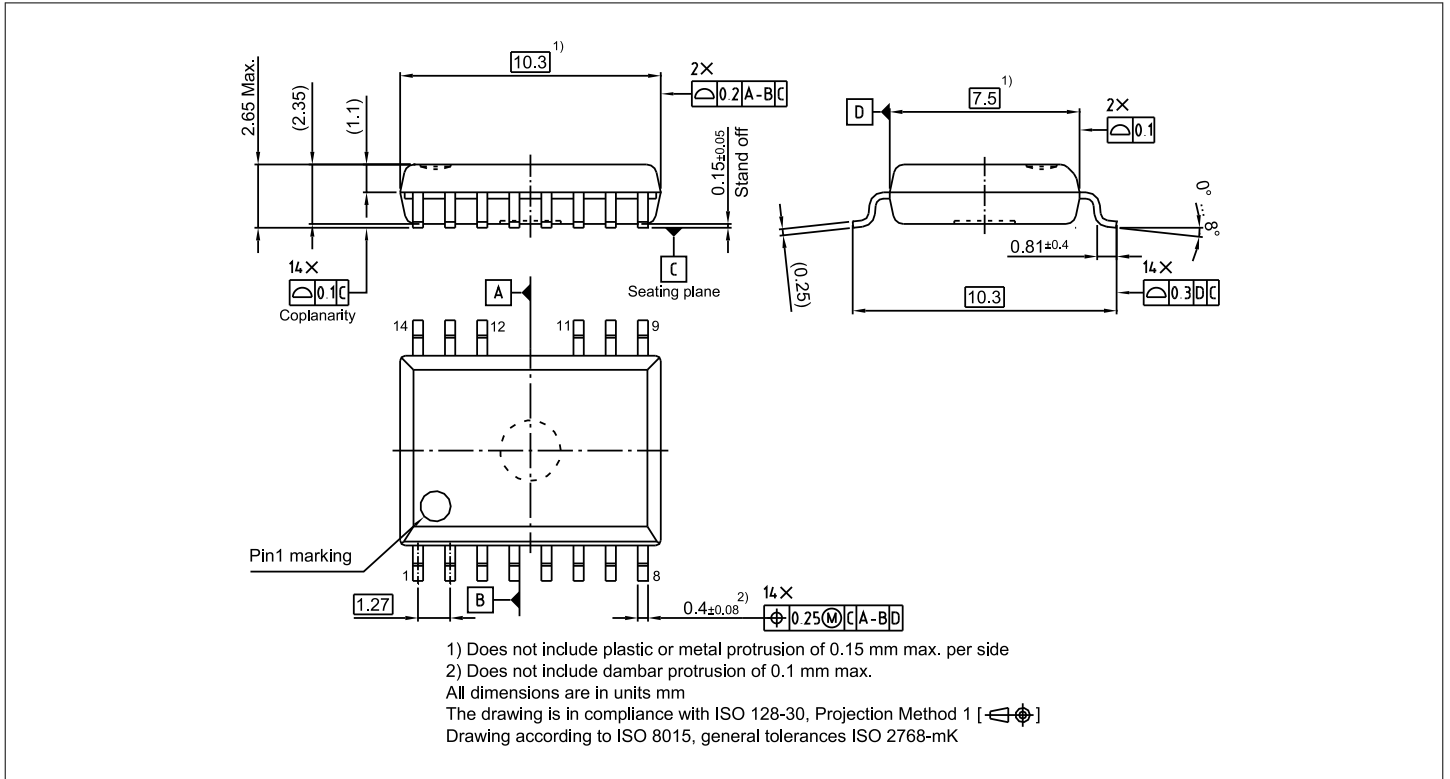
Figure 45 DSO-14-71 outline
