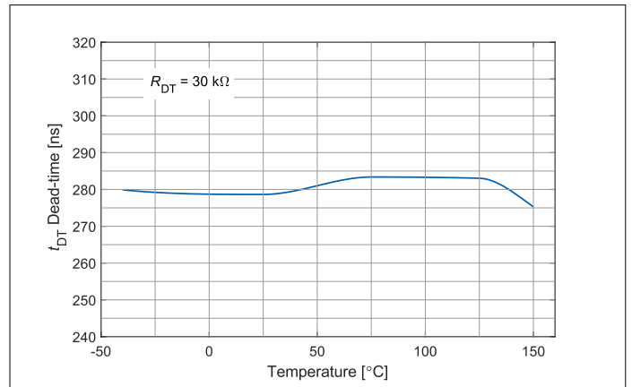
Figure 23 t_{\text{DT}} vs. temperature
