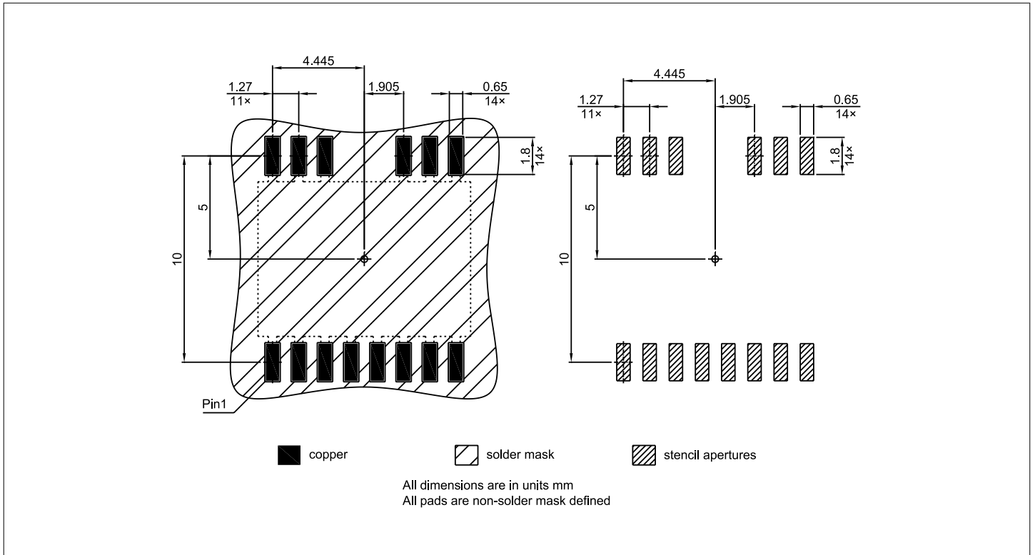
Figure 46 DSO-14-71 recommended footprint
