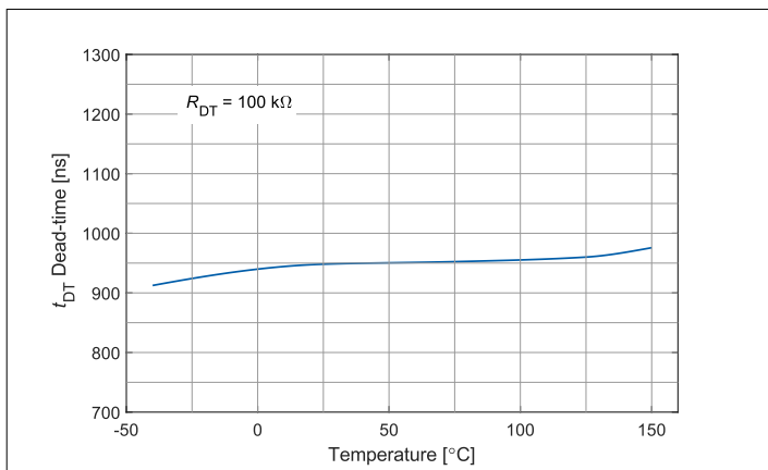
Figure 24 t_{\text{DT}} vs. temperature
