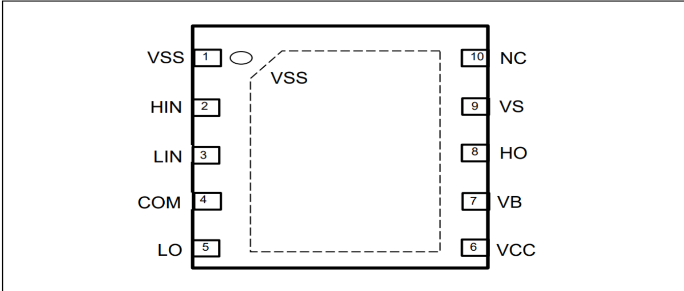
Figure 3 2ED2772S01G pin assignments (top view)
