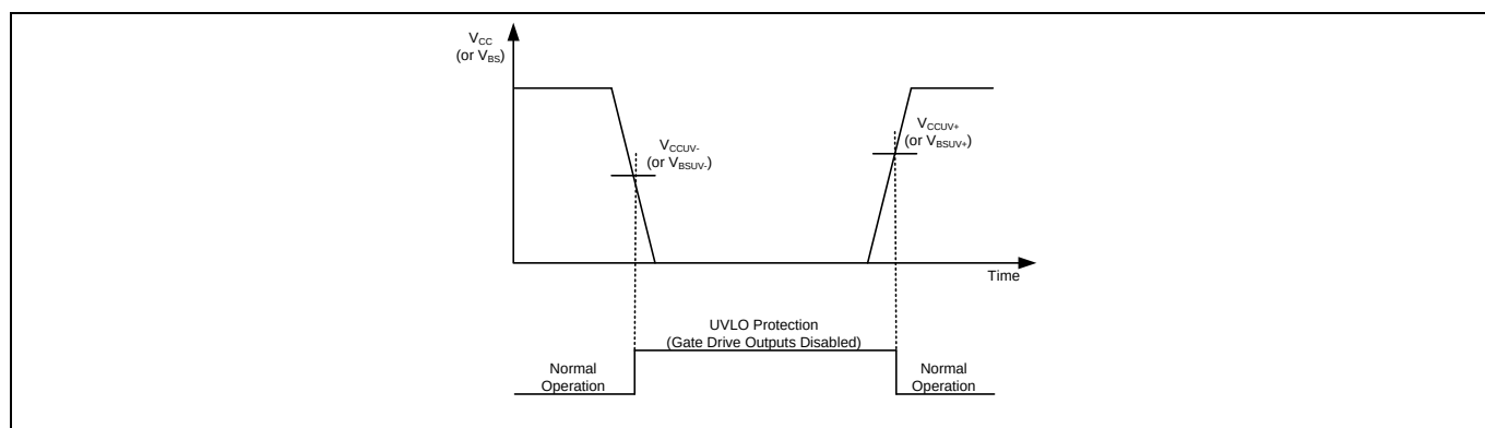
Figure 13 UVLO protection
