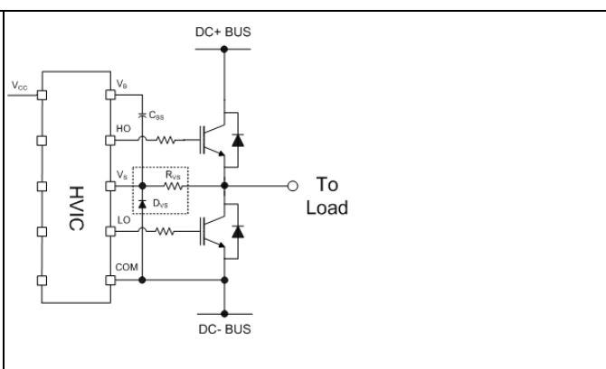
Figure 26 Clamping diode between COM and V_S
