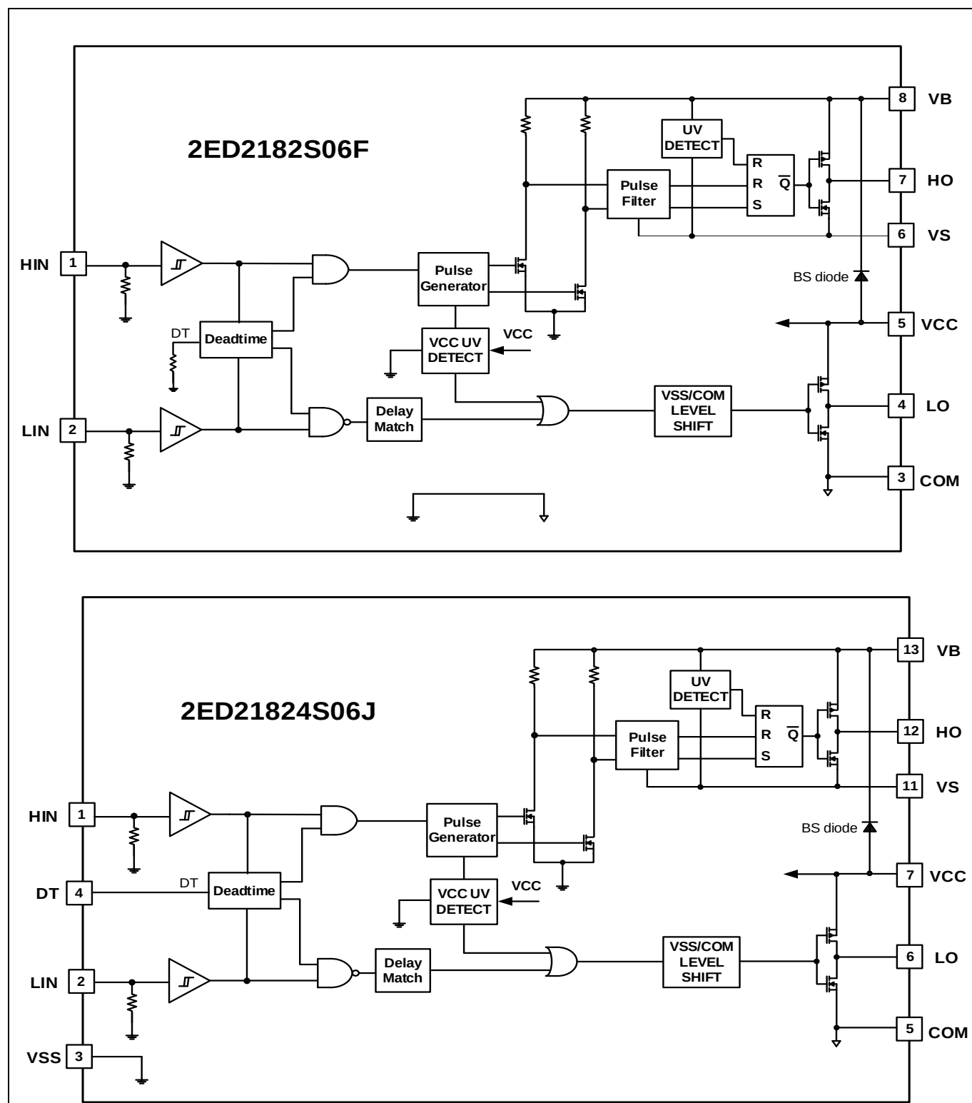
Figure 2 Block diagrams
