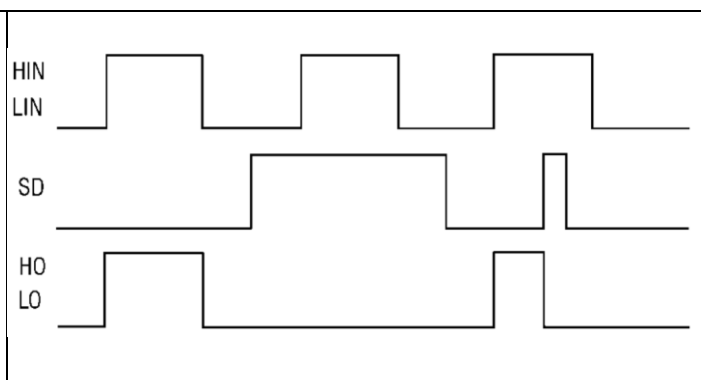
Figure 7 Input/output logic diagram
