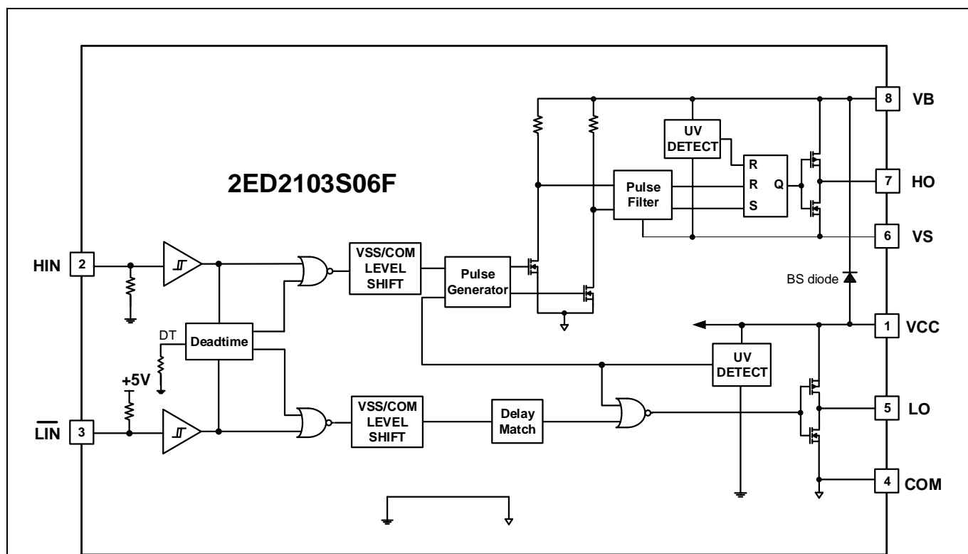
Figure 2 Block diagrams
