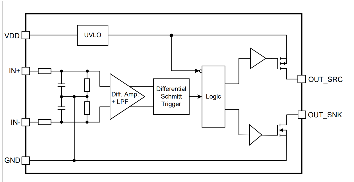
Figure 3 Simplified block diagram of EiceDRIVER™ 1EDNx550
