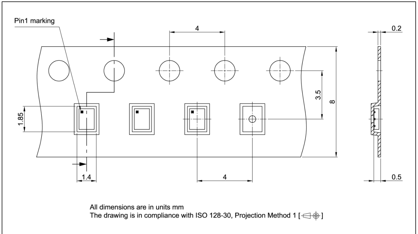
Figure 21 TSNP-6 packaging
