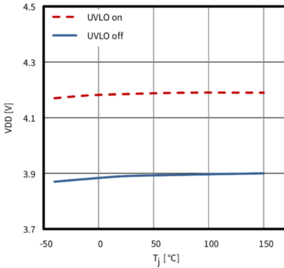
3. Undervoltage lockout threshold (1EDN6550) vs temperature
