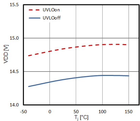
4. Undervoltage lockout threshold (1EDN9550) vs temperature
