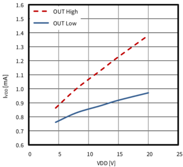
7. Typical quiescent current vs supply voltage
