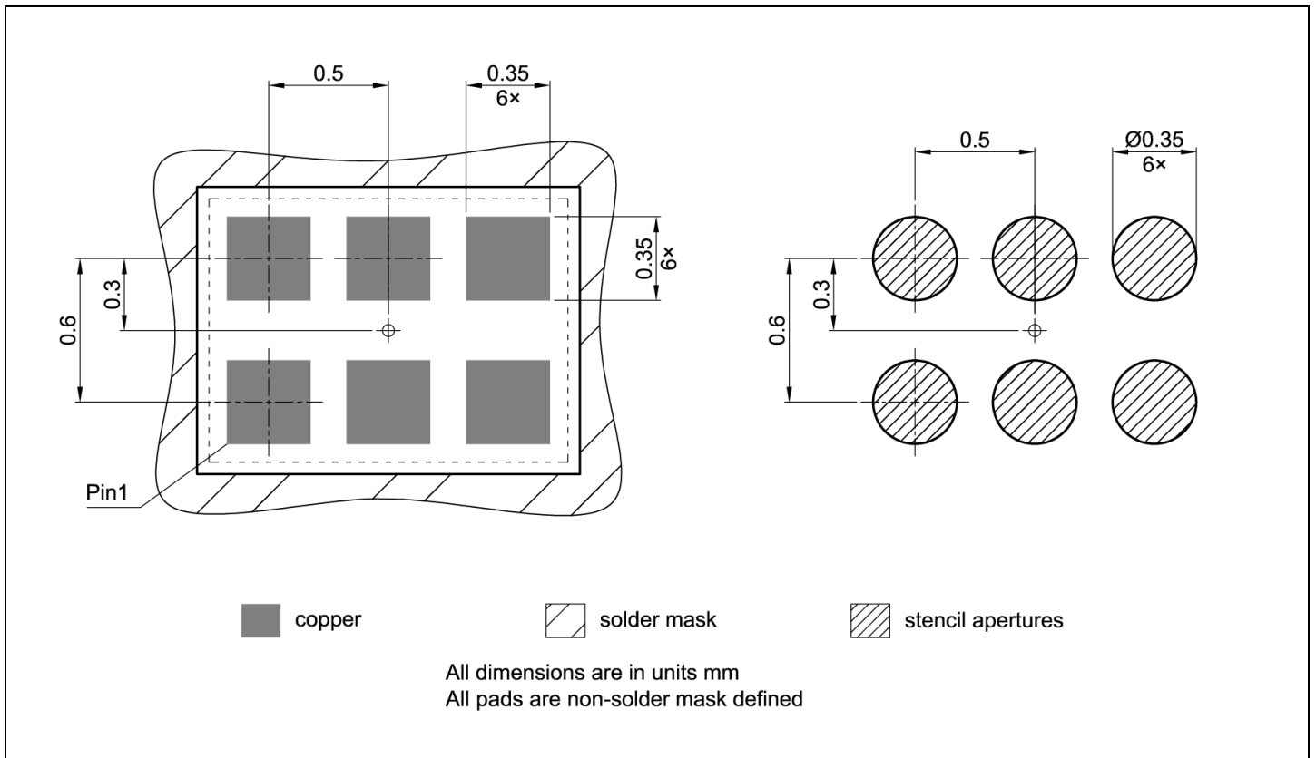
Figure 20 TSNP-6 footprint
