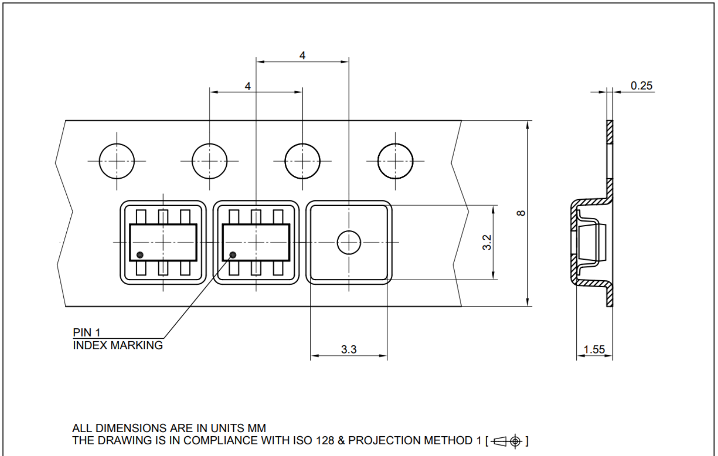
Figure 17 PG-SOT23-6 packaging
