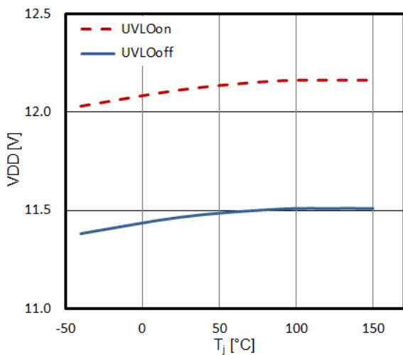
3. Undervoltage lockout threshold (1EDN6550) vs temperature
