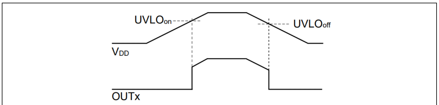
Figure 7 UVLO behavior (output state high)
