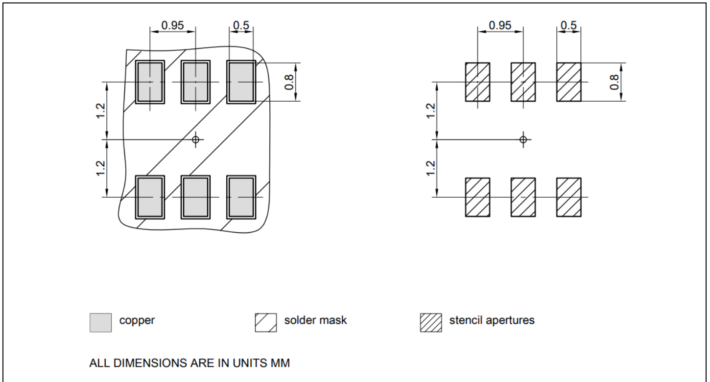
Figure 16 PG-SOT23-6 footprint
