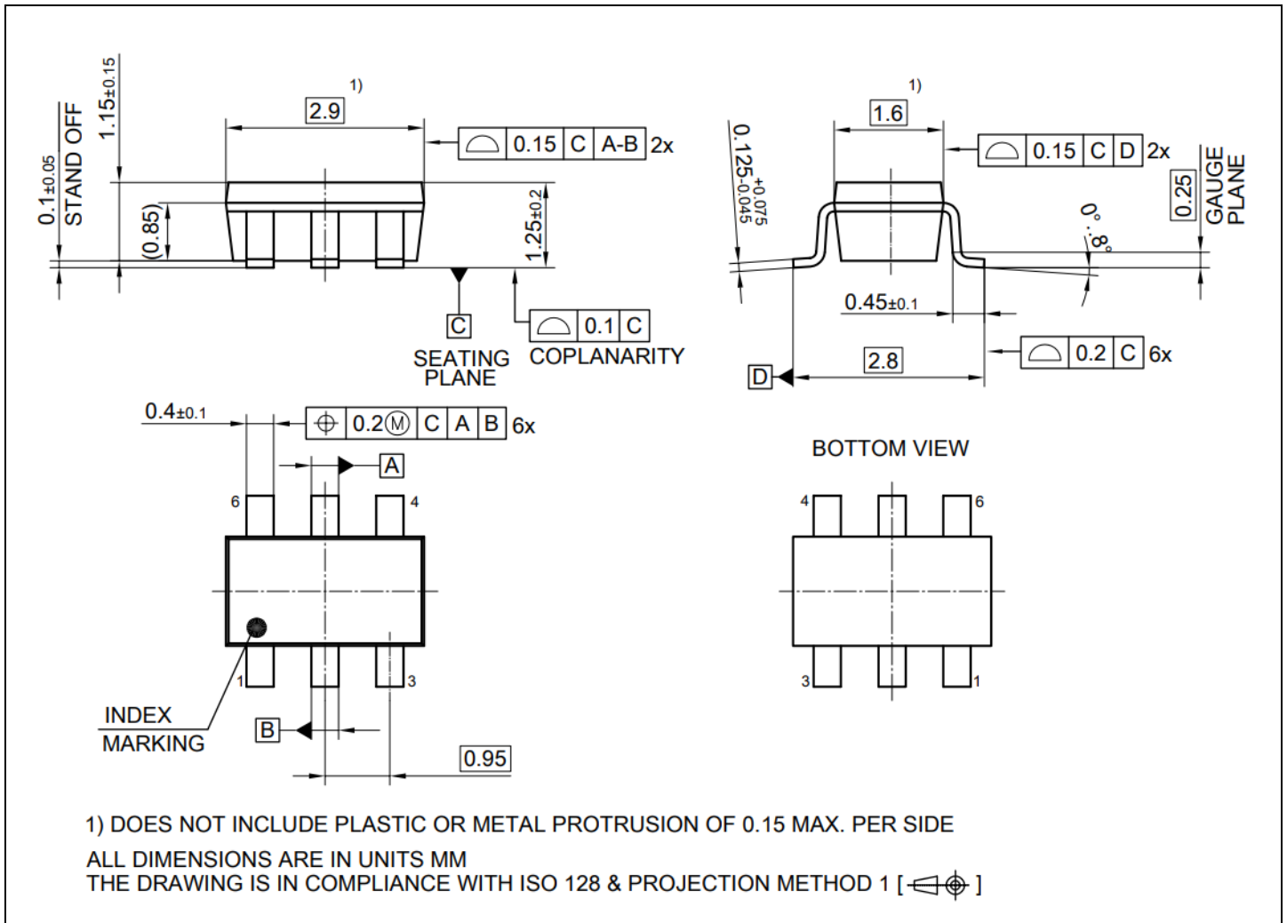
Figure 15 PG-SOT23-6 outline
