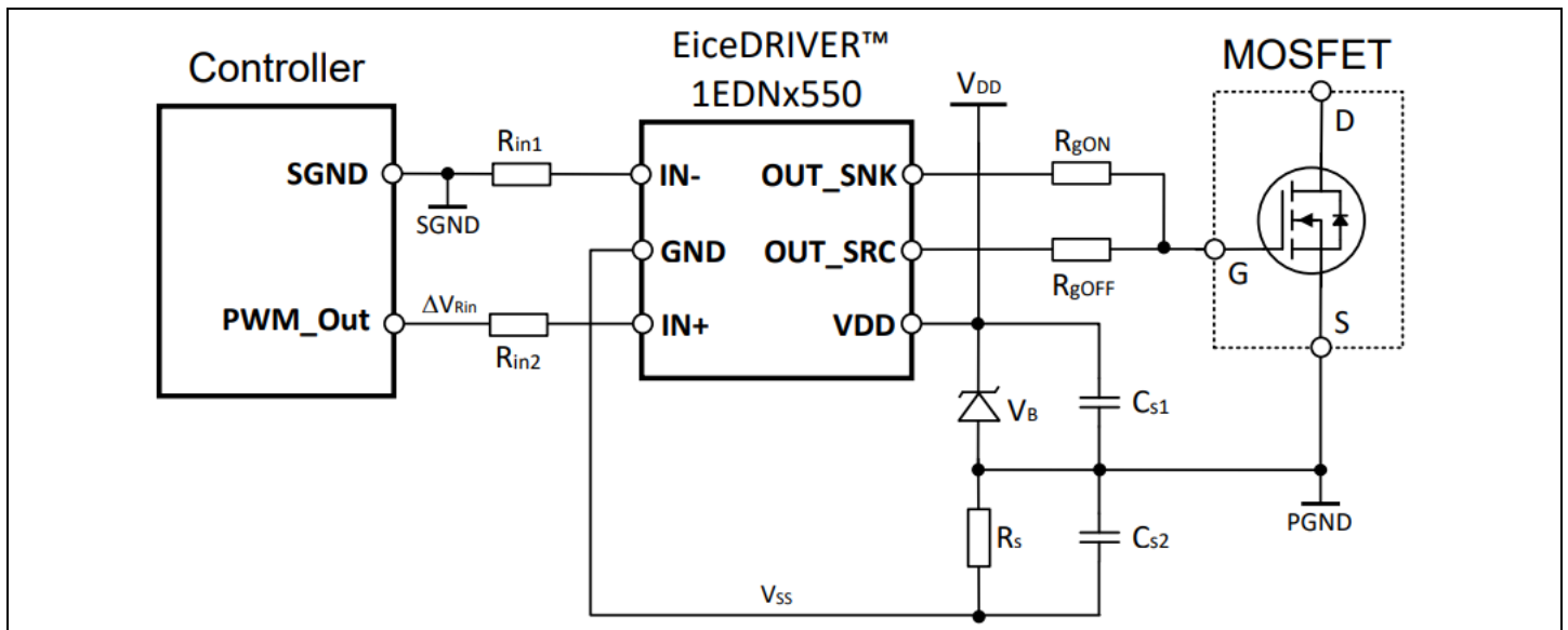
Figure 11 Bipolar gate drive for 3-pin MOSFET
