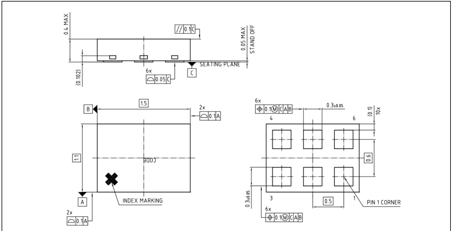
Figure 19 TSNP-6 outline
