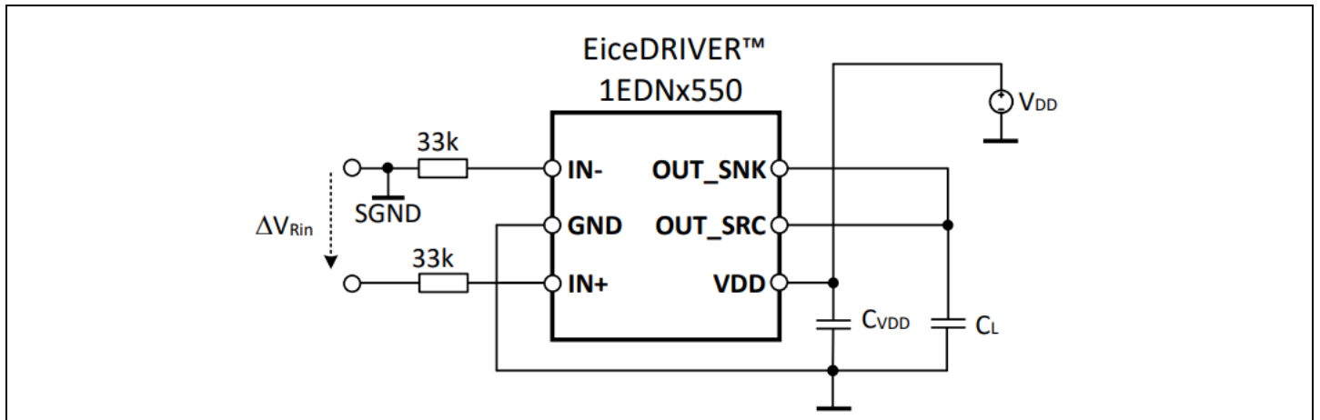
Figure 5 Test circuit
