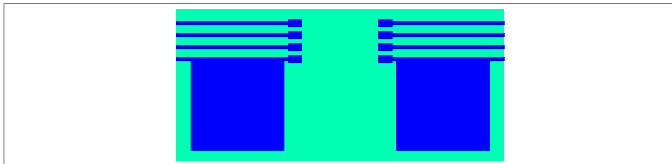
Figure 11 Reference layout for thermal data (Copper thickness 35 µm)
