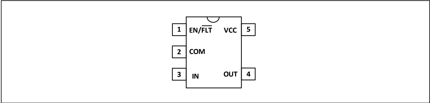
Figure 3 PG-SOT23-5-1 (top view)
