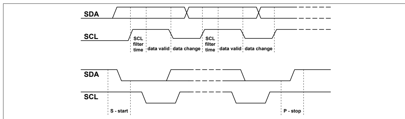
Figure 6 Start, stop and data conditions
