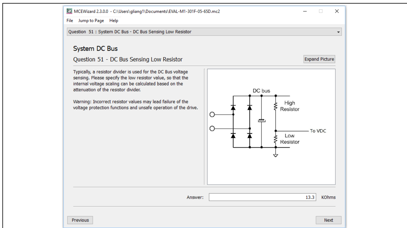
Figure 18 DC bus-sensing configuration in MCEWizard
