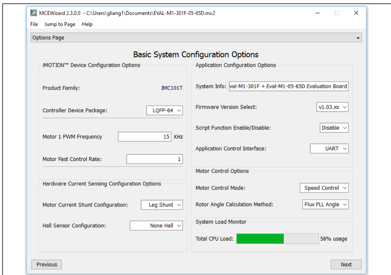
Figure 12 Shunt configuration
