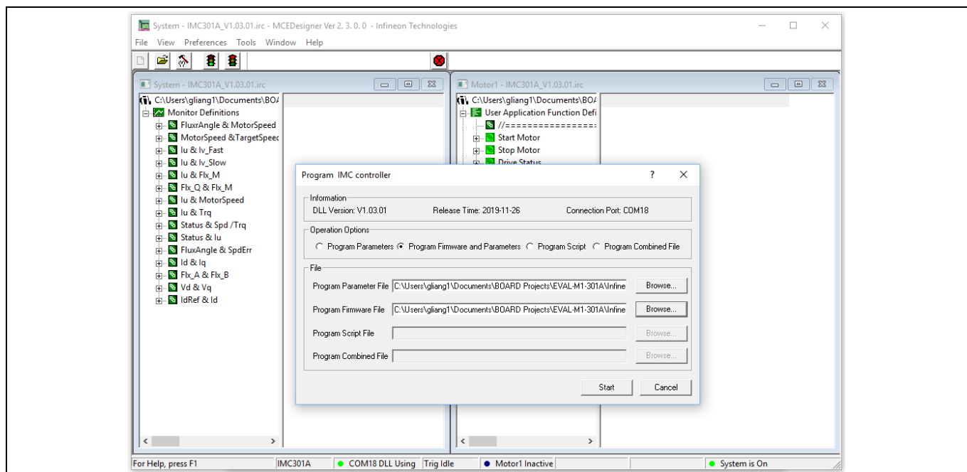
Figure 10 Program firmware and parameters in “Program IMC Controller” pop-up window
