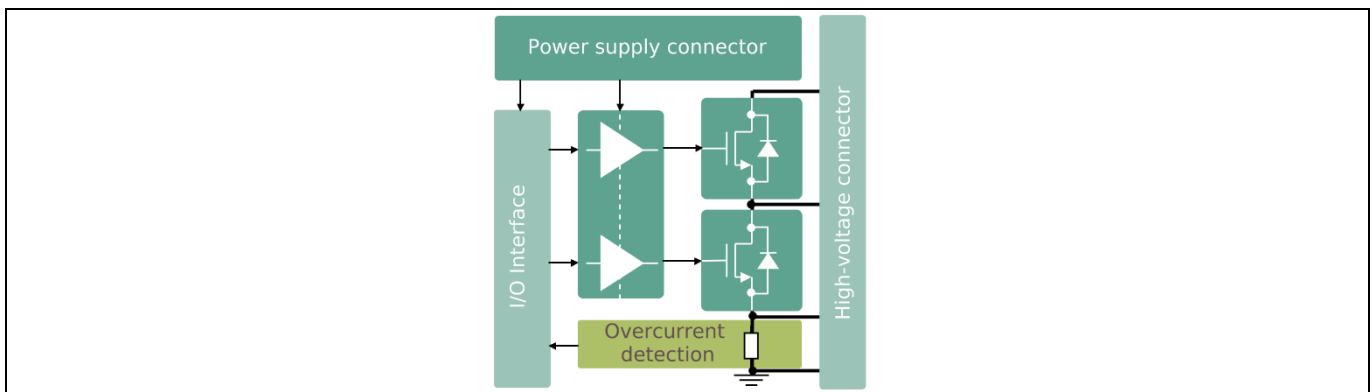
Figure 2 Eval-1ED3142MU12F-SiC evaluation board block diagram
