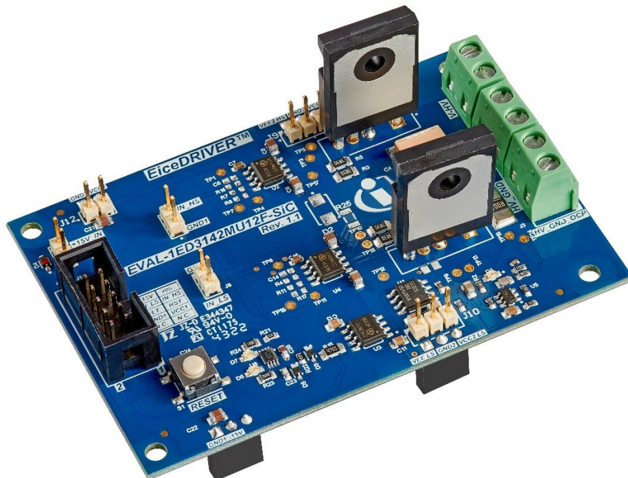
Figure 1 Eval-1ED3142MU12F-SiC evaluation board
