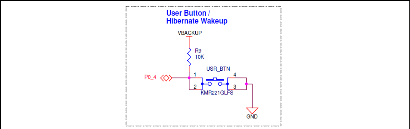
Figure 40 User button
