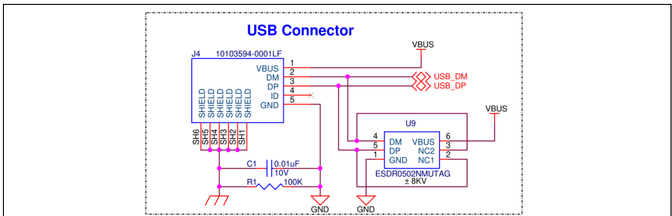
Figure 34 USB connector
