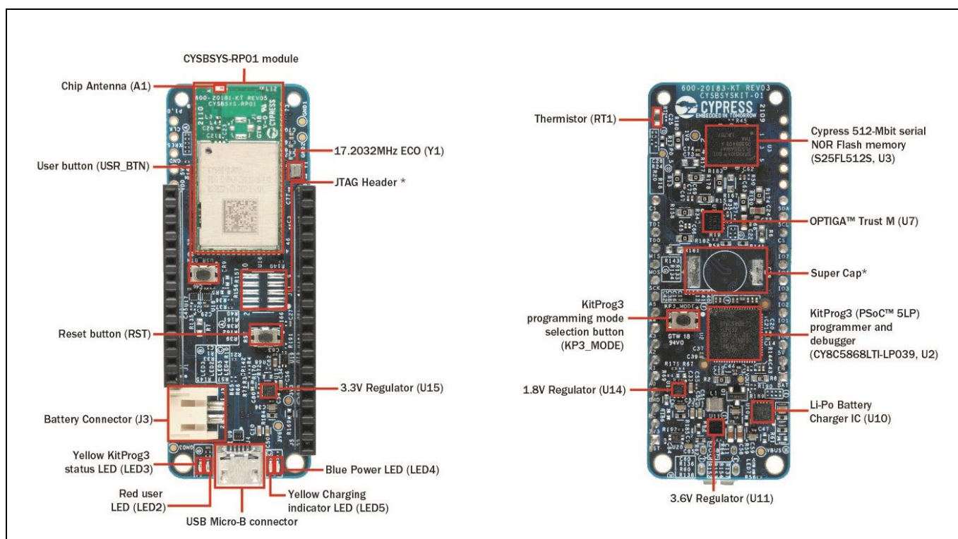
Figure 4 CYSBSYSKIT-DEV-01
