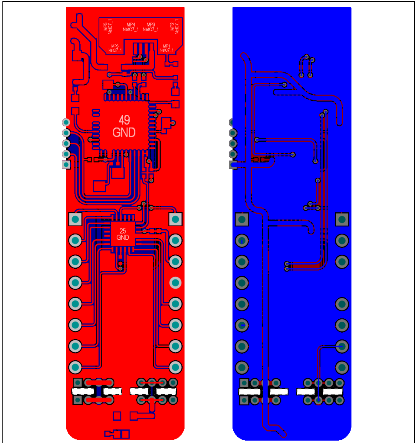
Figure 4 TLI55950 2Go evaluation kit PCB layout – Top (left), bottom (right)
