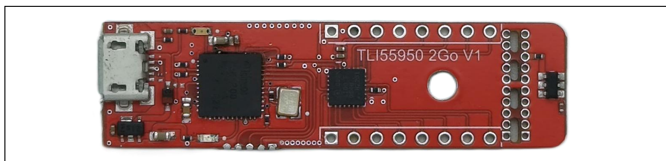
Figure 1 TLI55950 2Go evaluation kit
