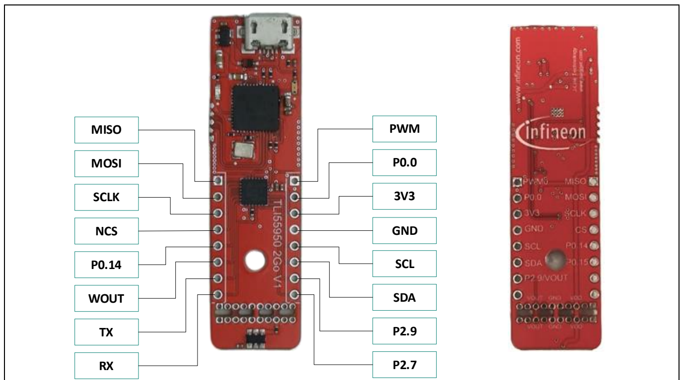
Figure 2 TLI55950 2Go evaluation kit auxiliary connector pinouts
