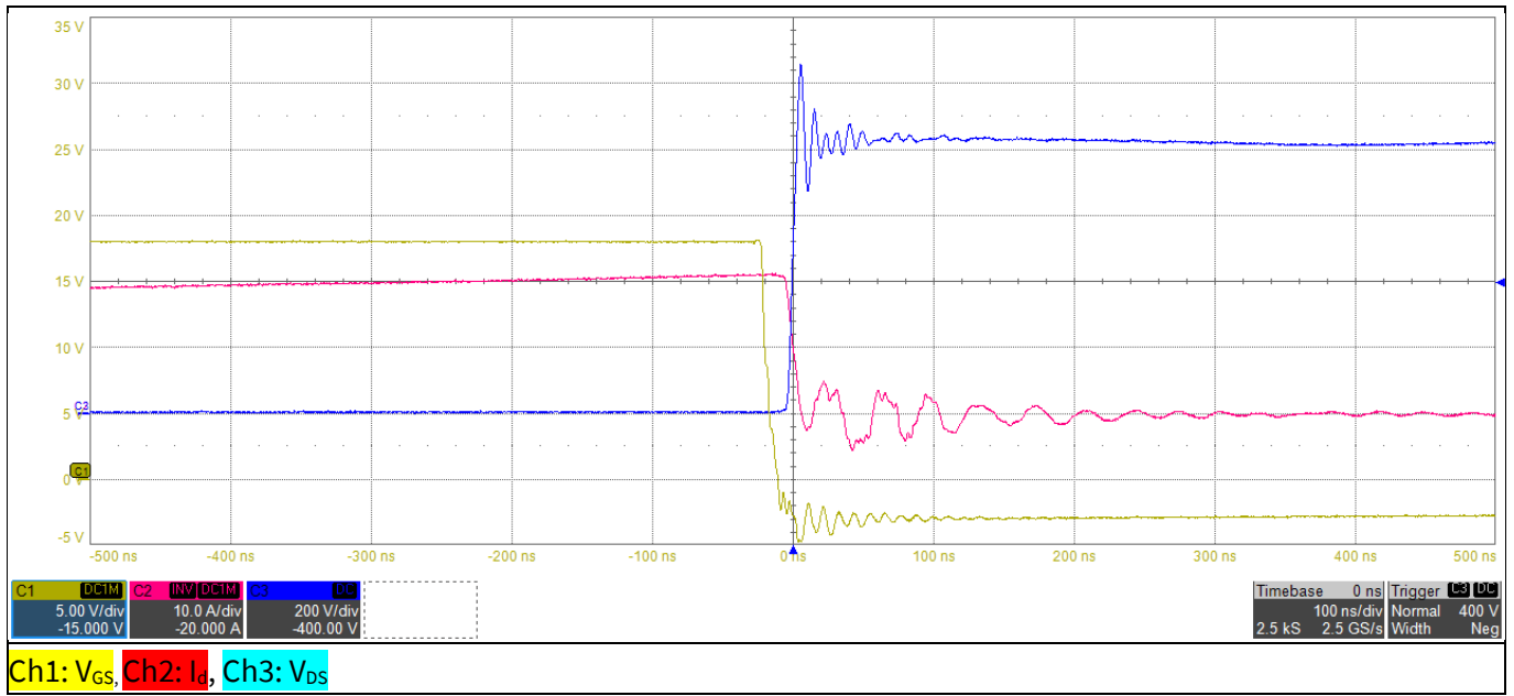
Figure 6 Eval-1EDR3146HQE-SiC – First turn-off of the low-side CoolSiC™ MOSFET
