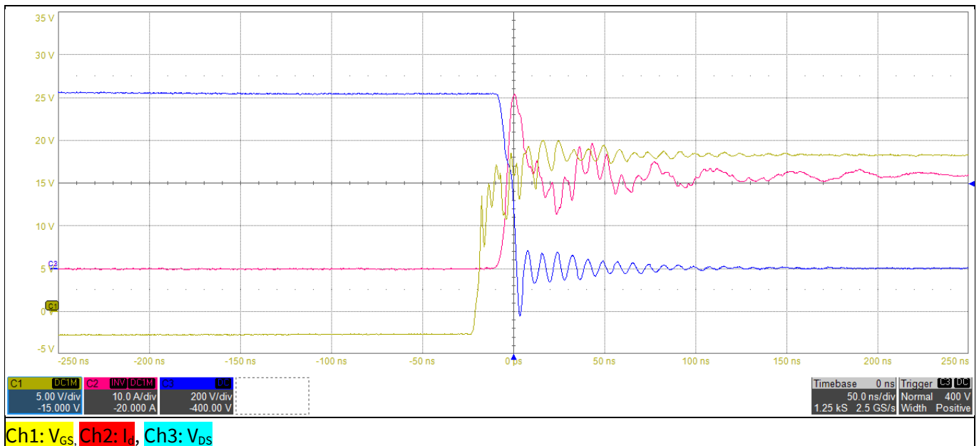
Figure 5 Eval-1EDR3146HQE-SiC – Second turn-on of the low-side CoolSiC™ MOSFET
