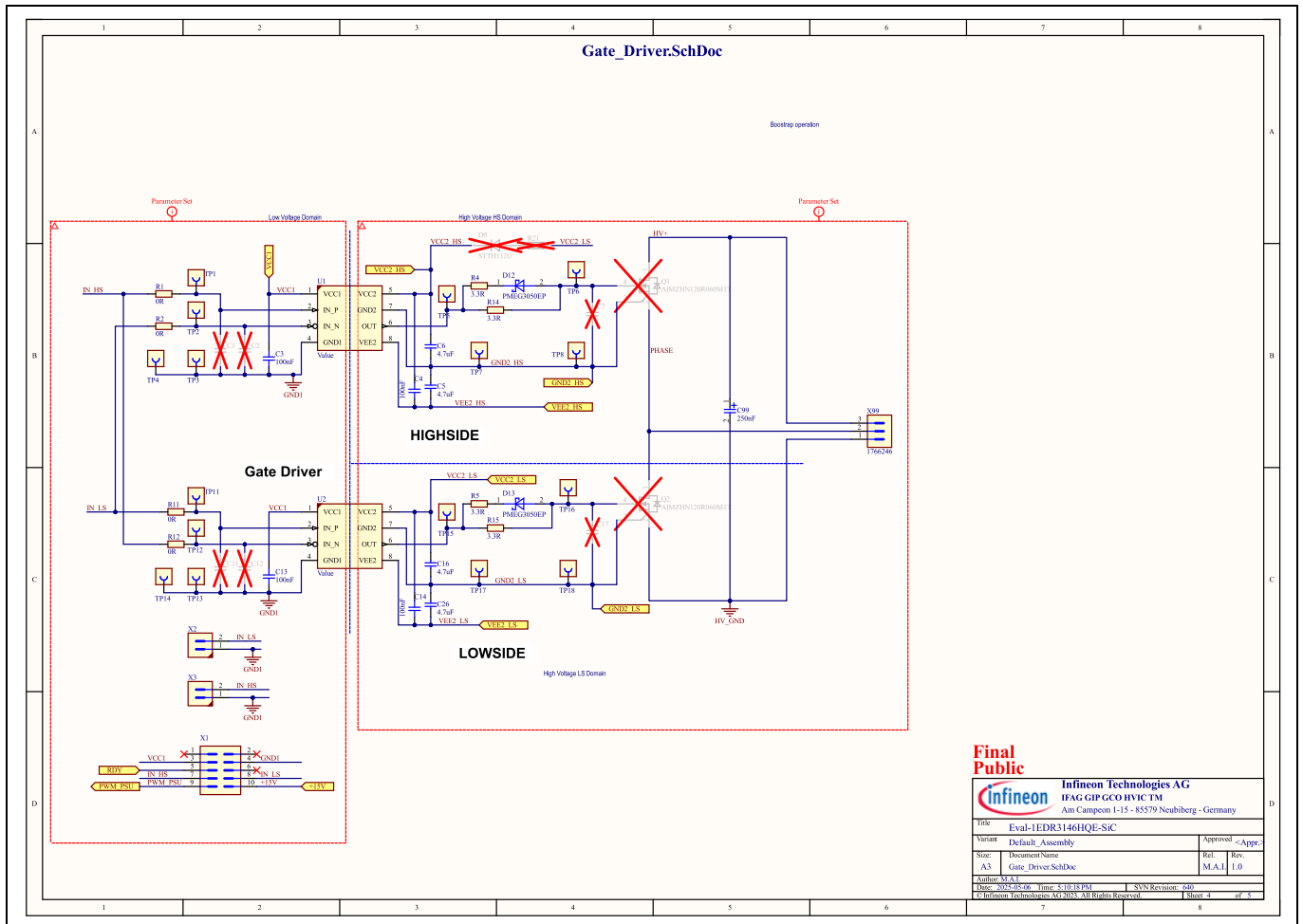
Figure 8 Gate driver circuit schematic
