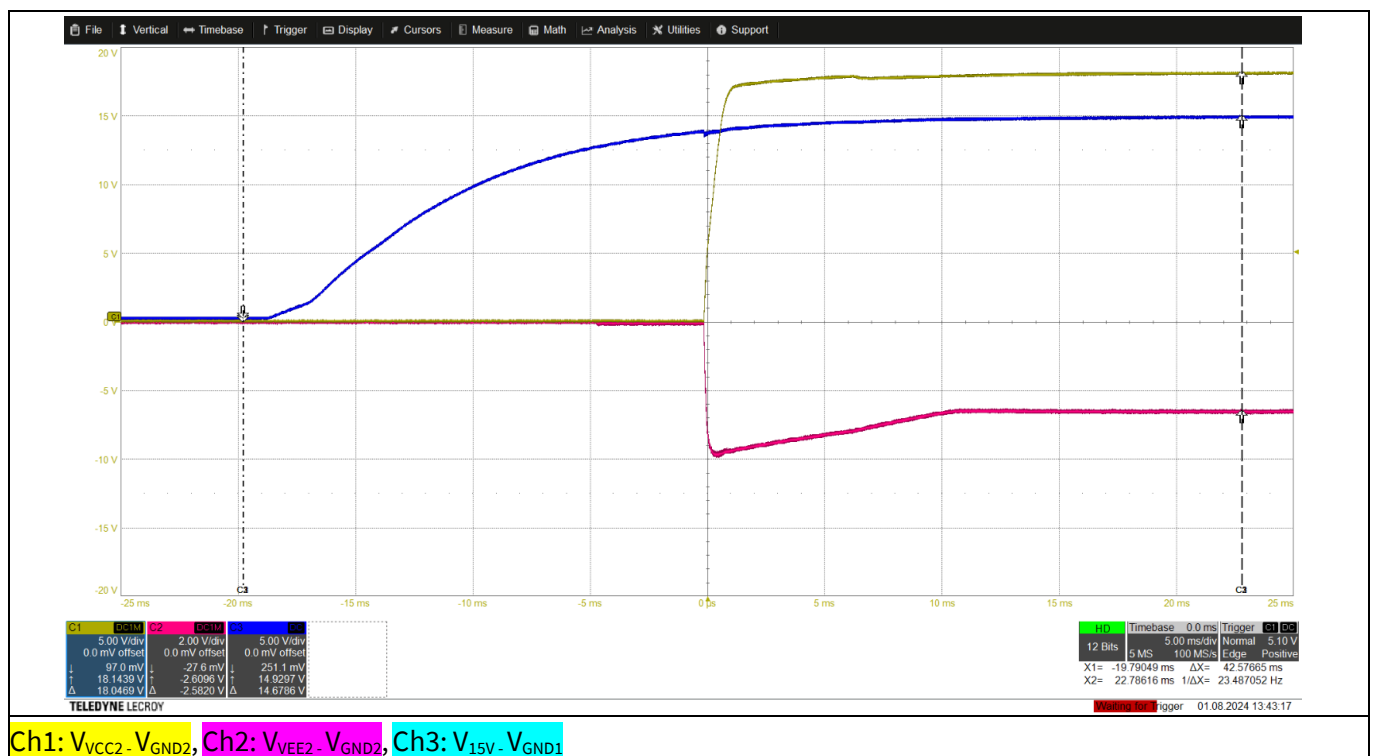
Figure 3 Eval-1EDR3146HQE-SiC – Power supply voltages startup
