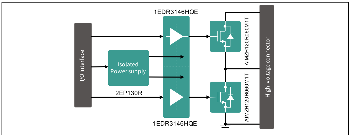
Figure 2 Eval-1EDR3146HQE-SiC evaluation board block diagram
