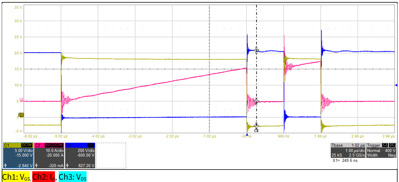
Figure 4 Eval-1EDR3146HQE-SiC – Double-pulse test of the low-side CoolSiC™ MOSFET
