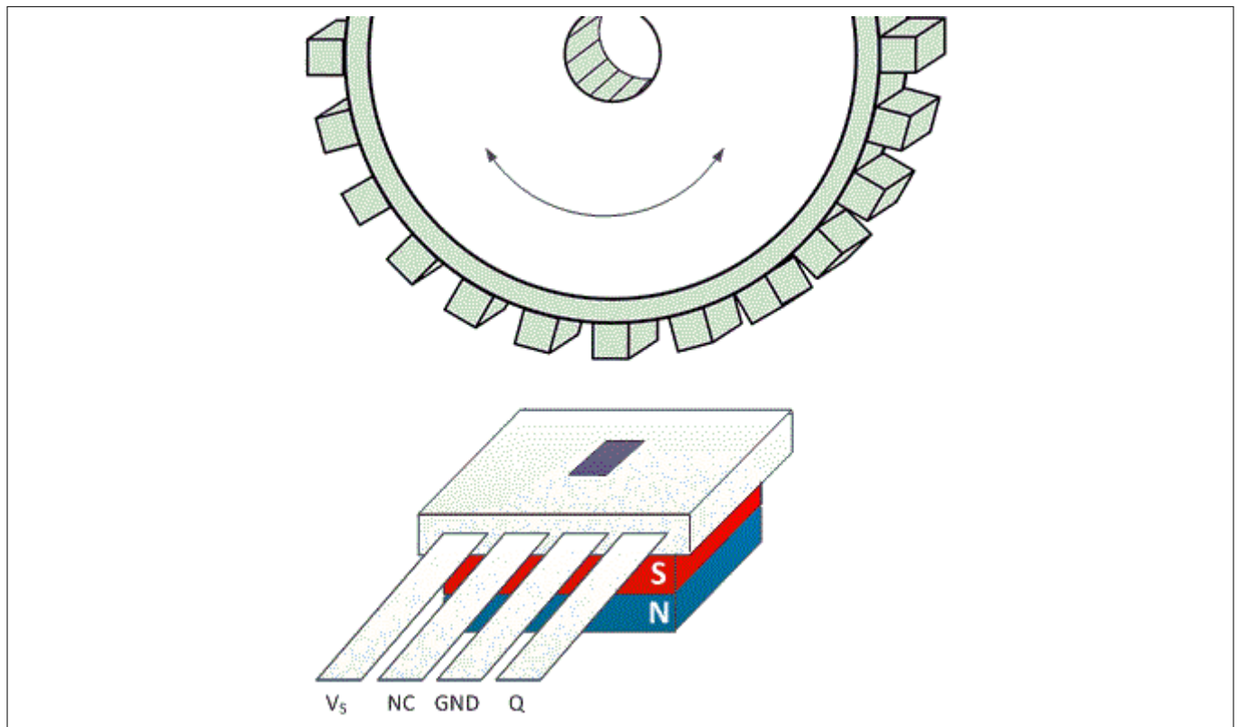
Figure 15 Schematic components of the magnetic circuit
