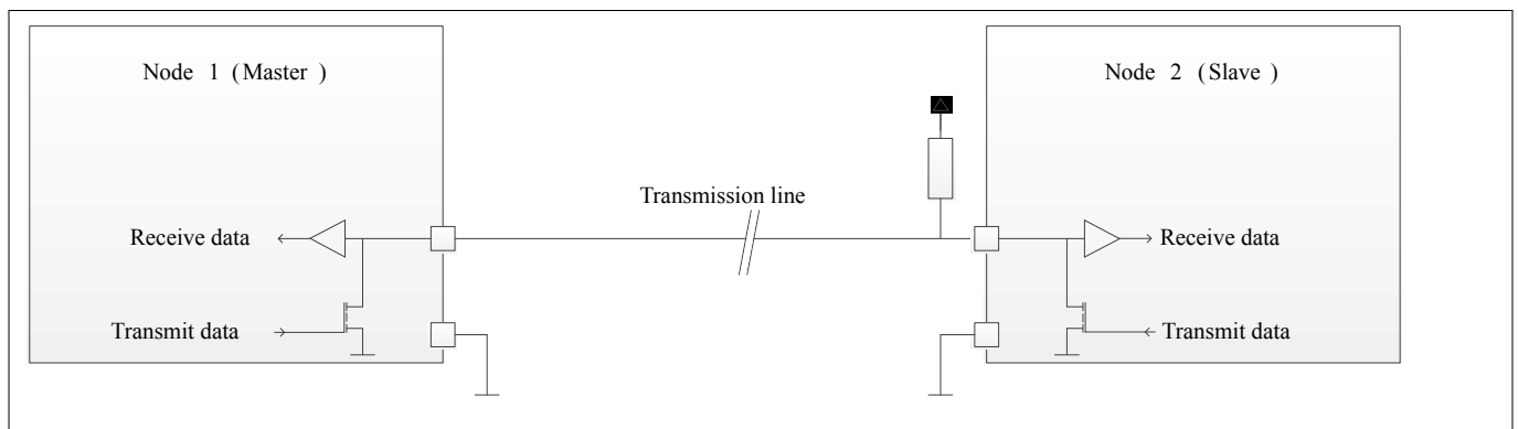
Figure 23 Physical layer of SICI
