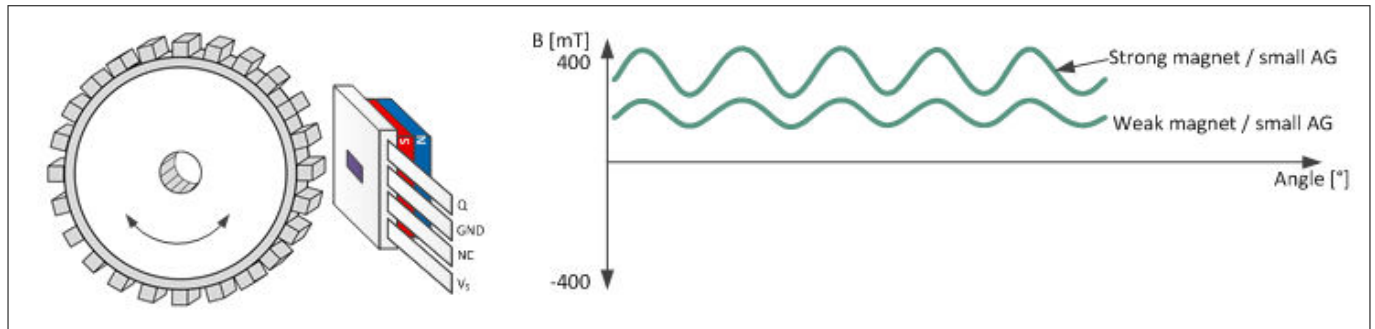
Figure 19 Magnetic signals with a strong and a weak back bias magnet
