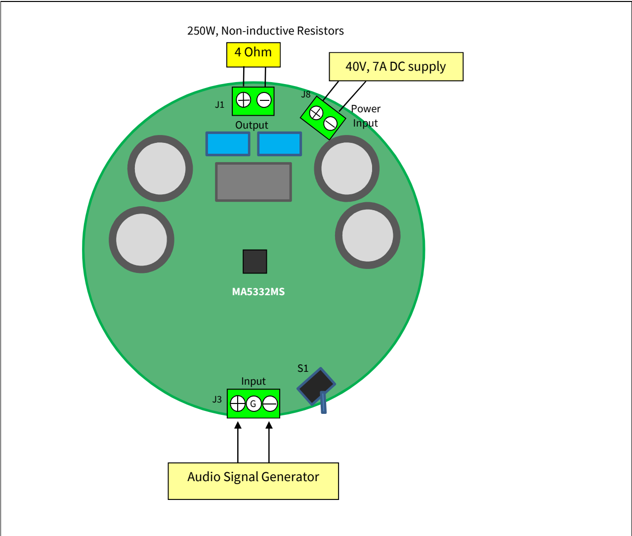
Figure 2 Typical connection connector description
