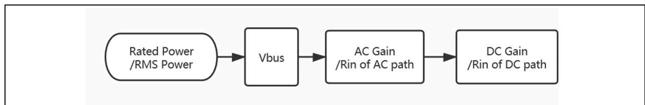
Figure 13 Gain design flow
