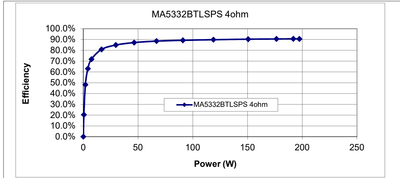
Figure 8 REF_MA5332BTLSPS 4 \Omega load stereo, V_{bus} = 40\text{ V}
