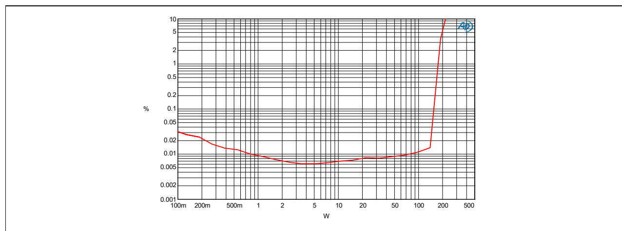
Figure 4 Power vs. THD+N 4\ \Omega load
