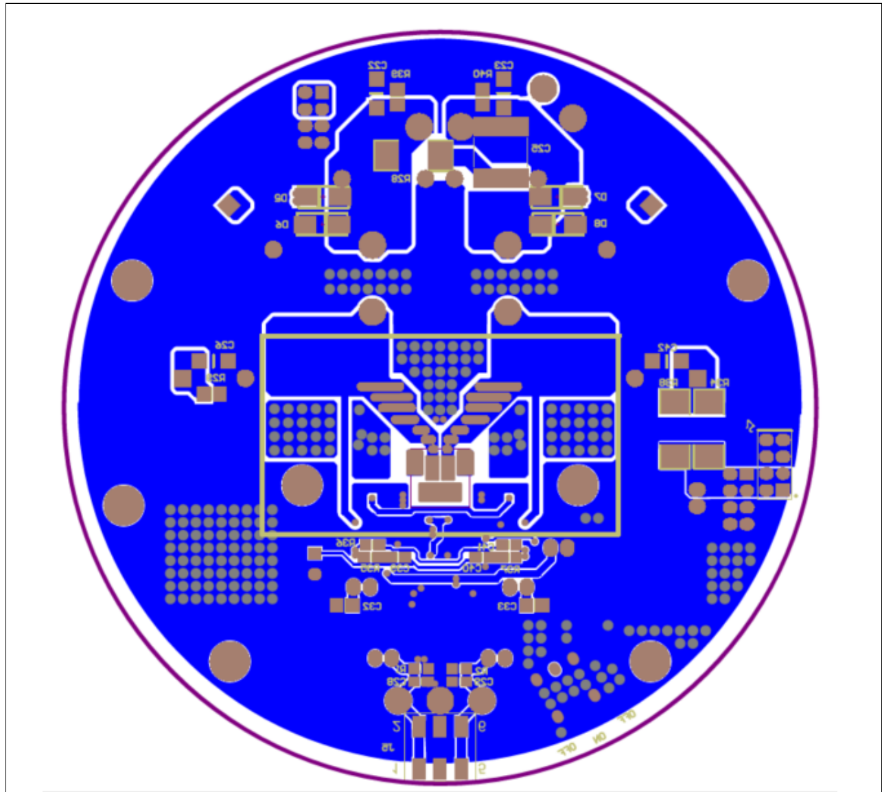
Figure 16 Board bottom view
