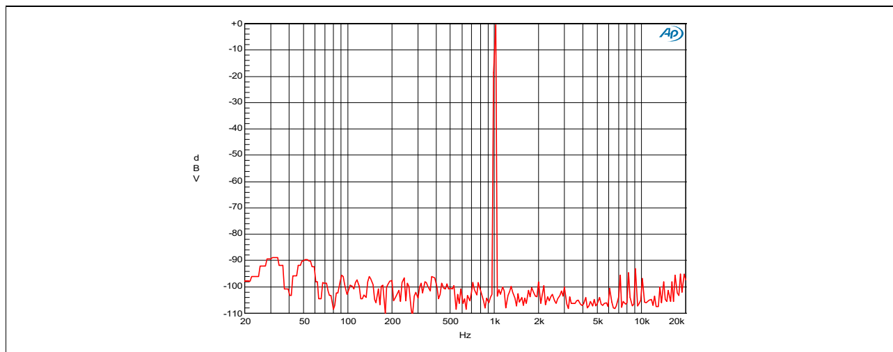
Figure 7 Noise floor with 1 V RMS output 4 \Omega load
