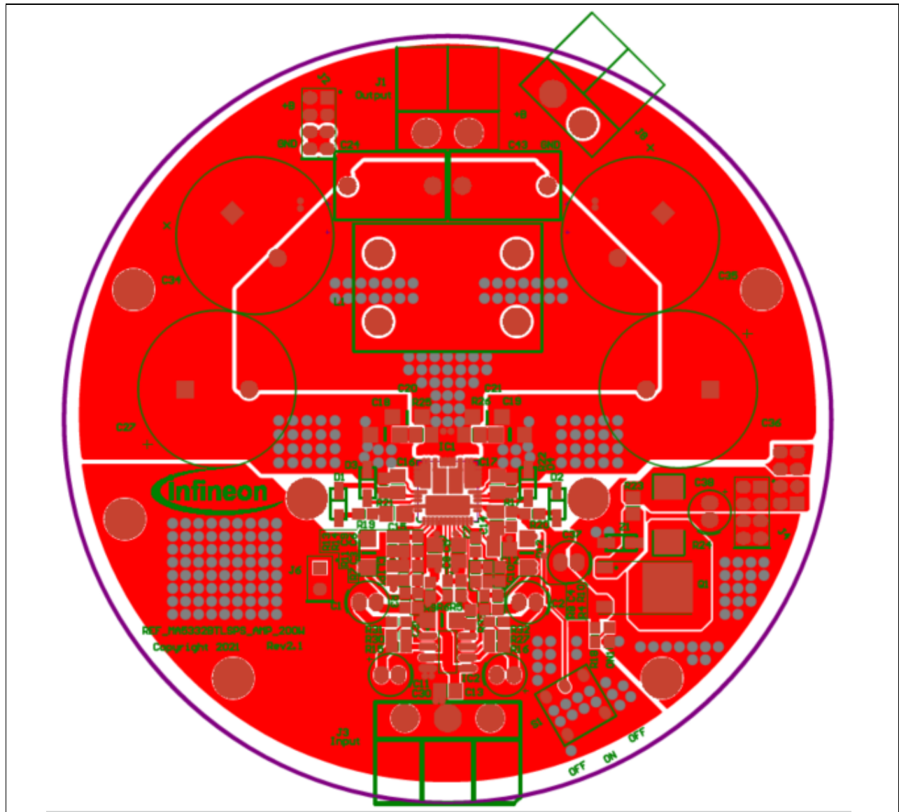
Figure 15 Board top view
