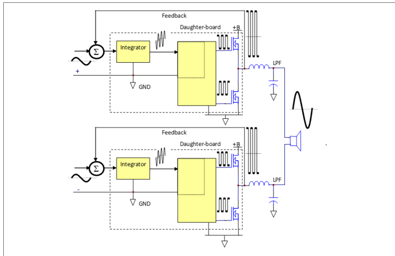
Figure 1 Simplified block diagram of class D amplifier
