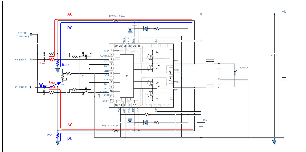
Figure 12 AC and DC path
