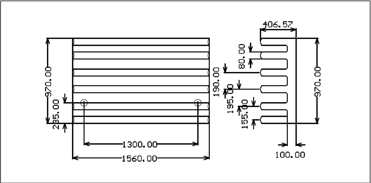
Figure 11 Heatsink dimension
