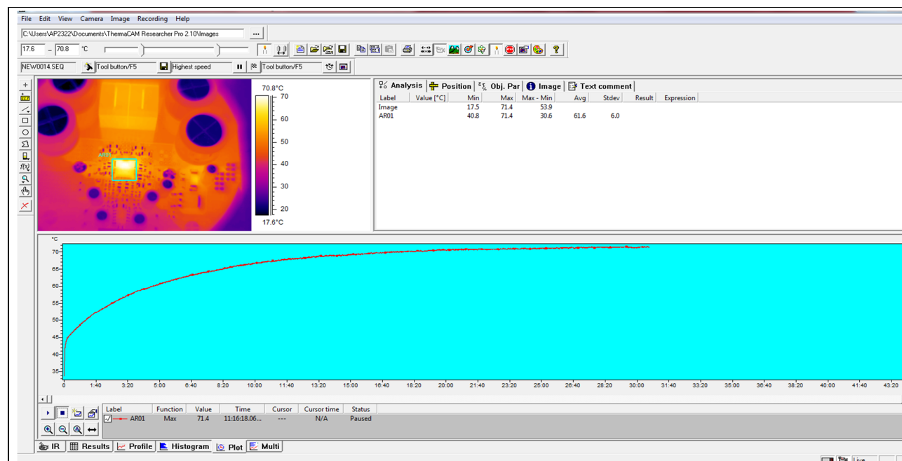
Figure 9 1/8Po power P_{out} = 18.75 \text{ W} with 4 \Omega load 40 V with heatsink
