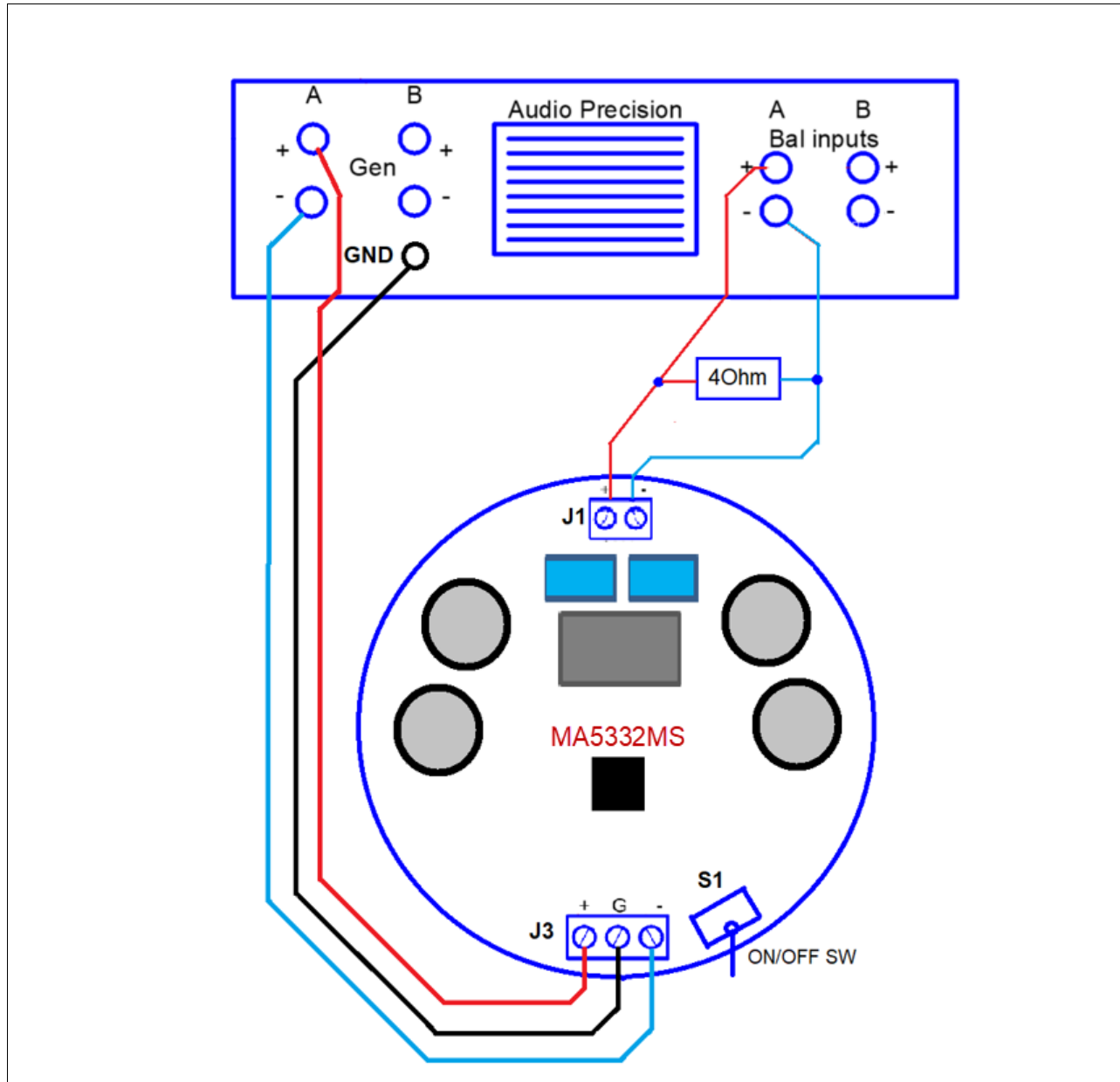
Figure 3 Audio analyzer connection
