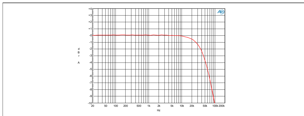
Figure 5 Frequency response 4\ \Omega load
