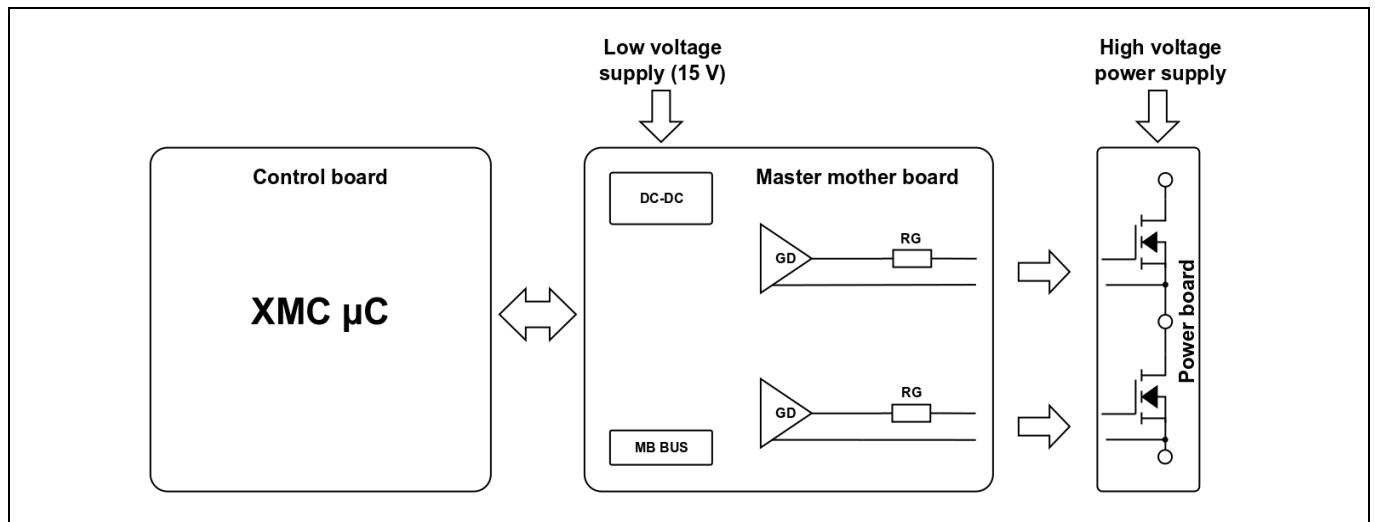
Figure 14 Block diagram
