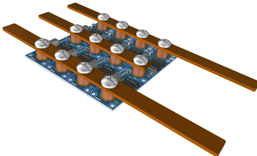
Figure 18 Four power boards connected in parallel via copper bars
