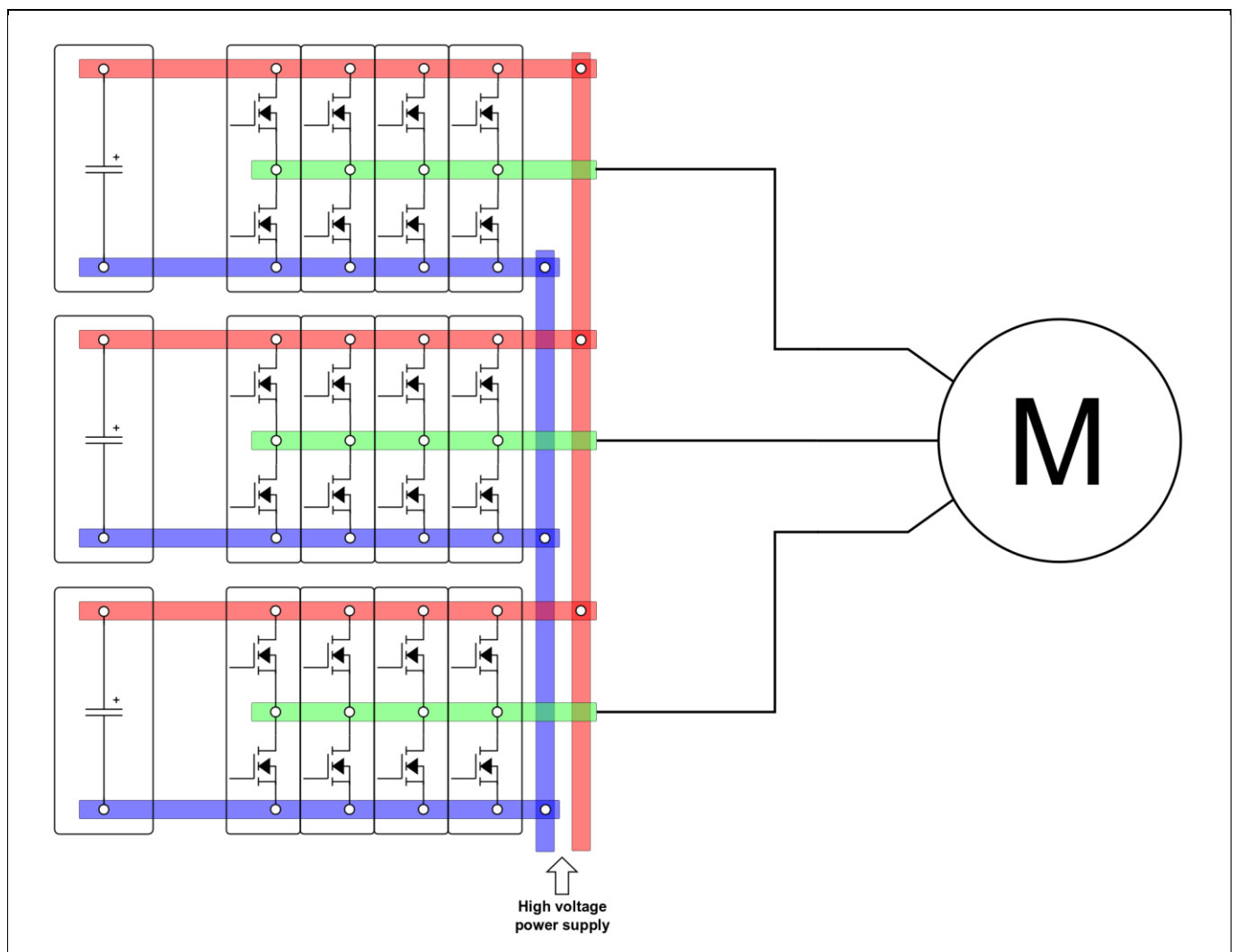
Figure 28 Power connections
