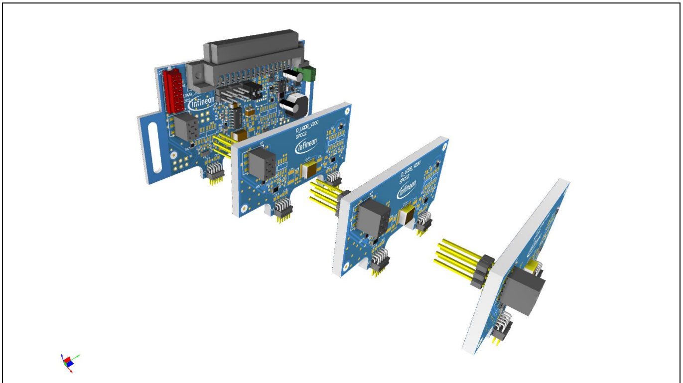
Figure 19 Master mother board and daughter boards
