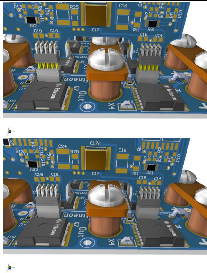
Figure 22 After alignment, push all the headers all the way into the receptacles
