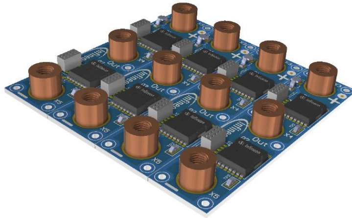
Figure 17 Four power boards – unconnected
