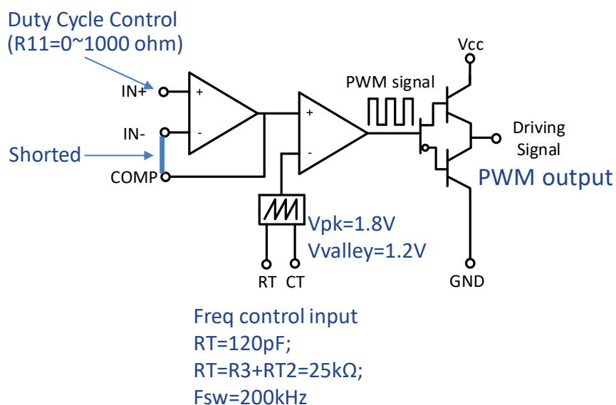
Figure 4 • GS65011-EVBZ PWM signal adjustment diagram
