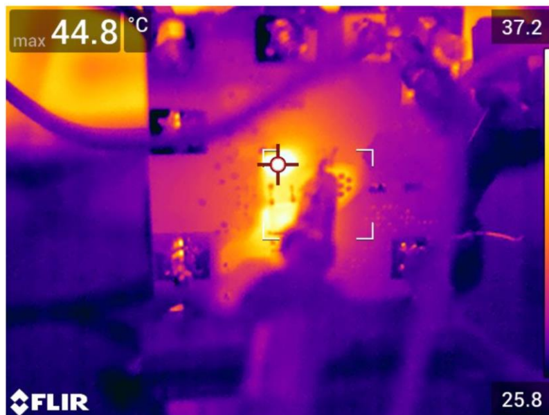
Figure 11 • Thermal imaging with an external fan ( T_{MAX} = 44.8^{\circ}C )
