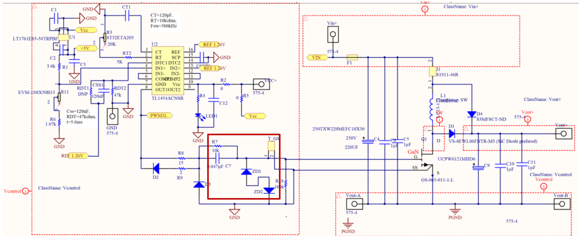
Figure 3 • GS65011-EVBEZ Schematic
