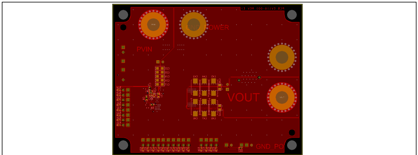
Figure 3 Bottom layer
