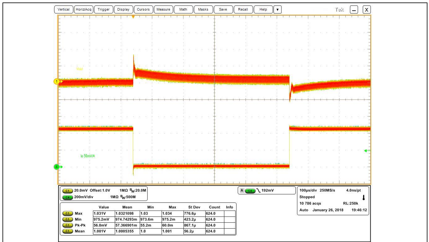
Figure 18 Transient response at 9 A step-load current at 30 A/µs slew rate: I out = 0 A to 9 A, (Ch 1 : V out , Ch 4 : I out ) pk-pk: 60 mV, fsw = 800 kHz
