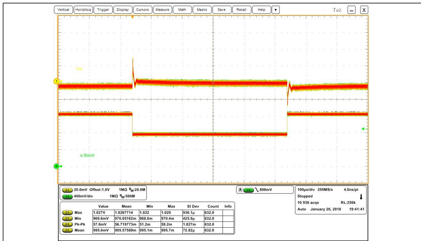
Figure 22 Transient response at 9 A step-load current at 30 A/μs slew rate: I_{out} = 16 \text{ A} to 25 A, (Ch1: V_{out} , Ch4: I_{out} ), pk-pk: 59.2 mV, fsw = 1000 kHz
