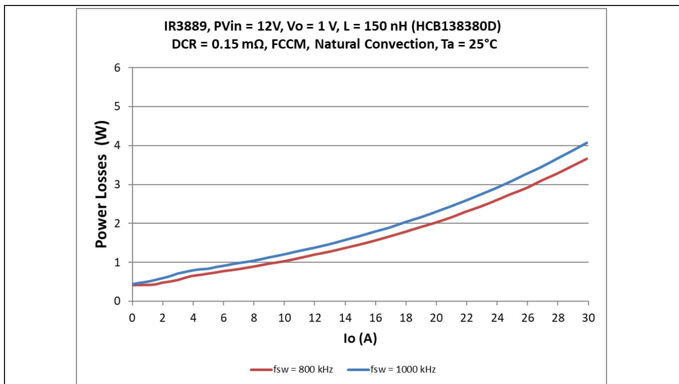
Figure 24 Power loss with natural convection ( 12\text{ V}_{in} , 1\text{ V}_{out} , 150\text{ nH} , 800\text{ kHz}/1000\text{ kHz} , T_a = 25^\circ\text{C} )
