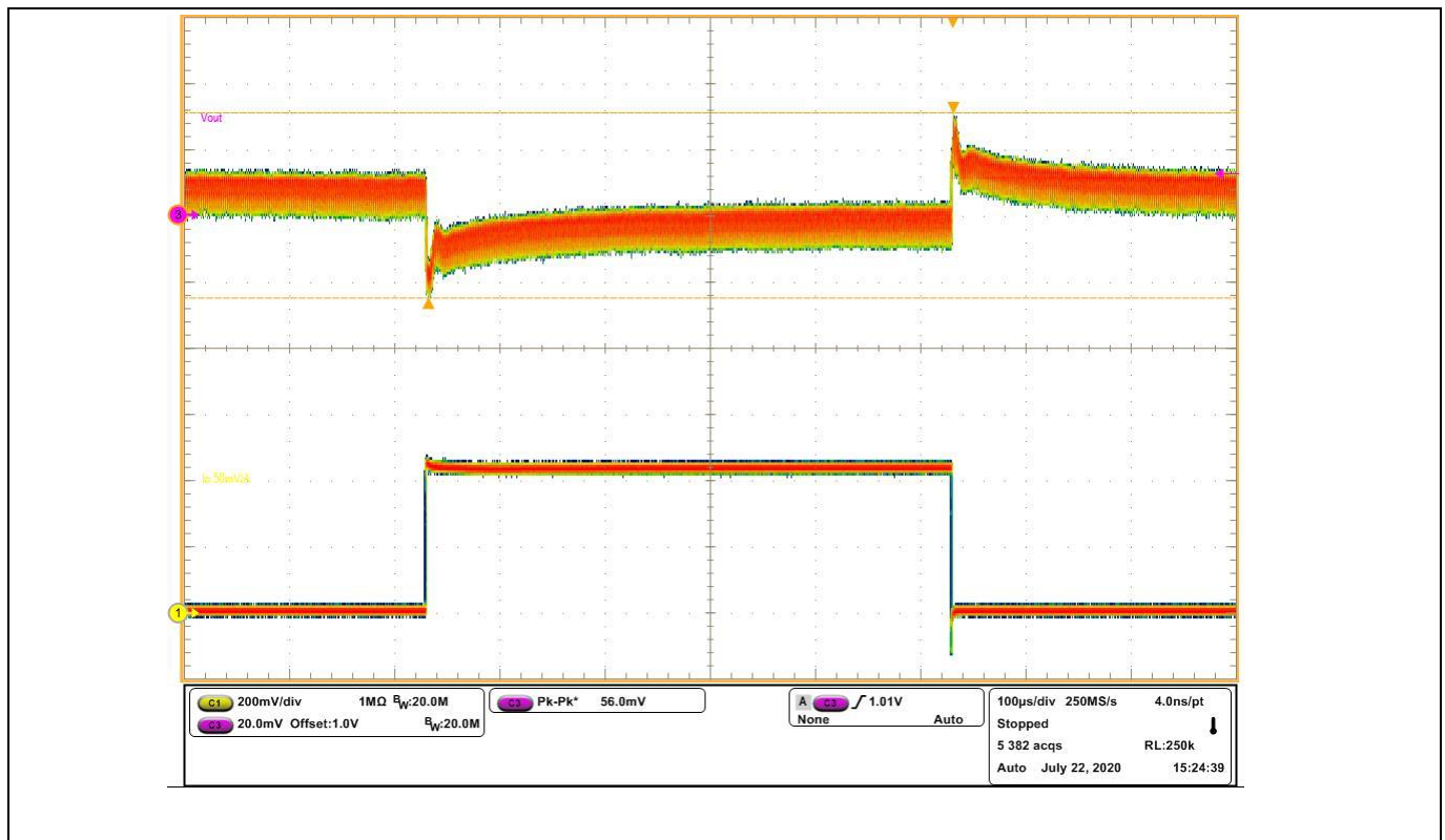
Figure 19 Transient response at 9 A step-load current at 30 A/μs slew rate: I_{out} = 0 A to 9 A (Ch 3 : V out , Ch 1 : I out ) pk-pk: 56 mV, f_{sw} = 600 kHz
