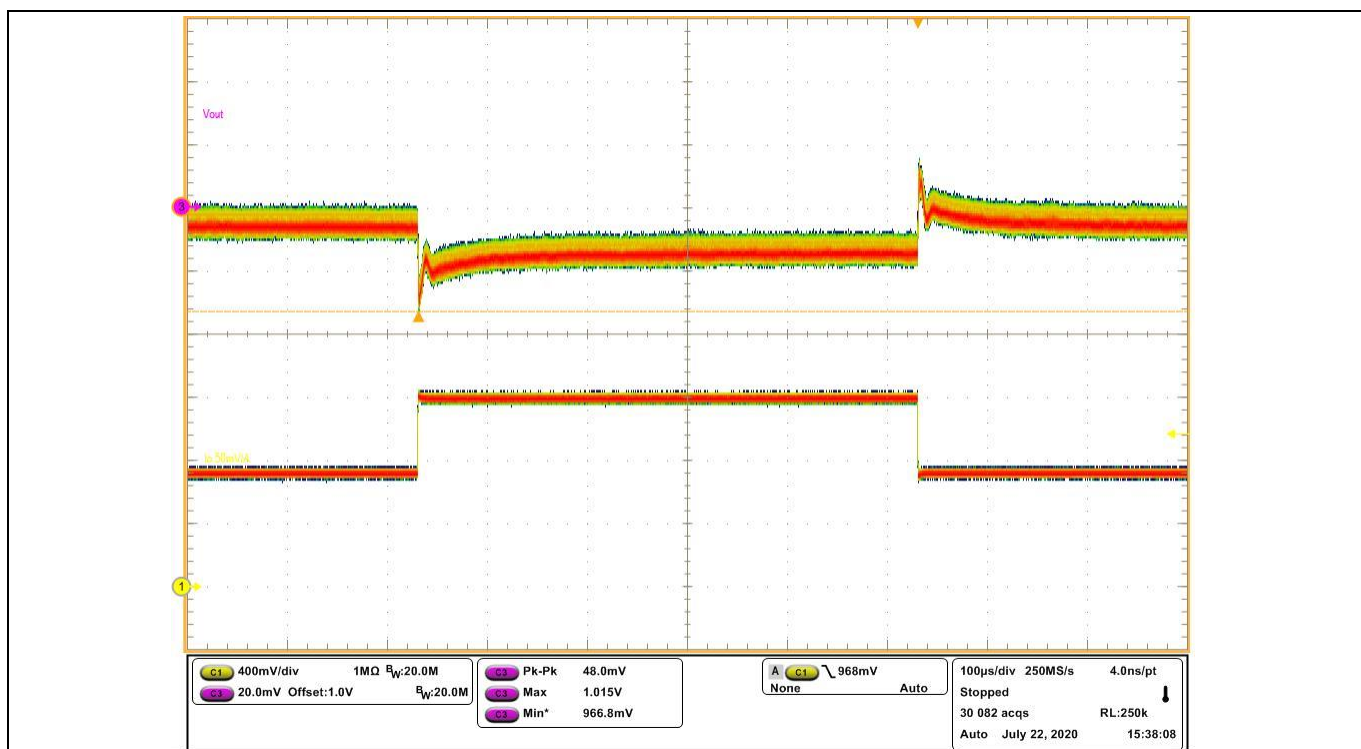
Figure 24 Transient response at 9 A step-load current at 30 A/μs slew rate: I_{out} = 16 \text{ A to } 25 \text{ A} (Ch 3 : V out , Ch 1 : I out ) pk-pk: 48 mV, f_{sw} = 1000 \text{ kHz}
