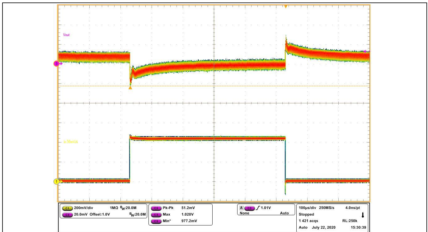
Figure 20 Transient response at 9 A step-load current at 30 A/μs slew rate: I_{out} = 0 A to 9 A (Ch 3 : V out , Ch 1 : I out ), pk-pk: 51.2 mV, f_{sw} = 800 kHz
