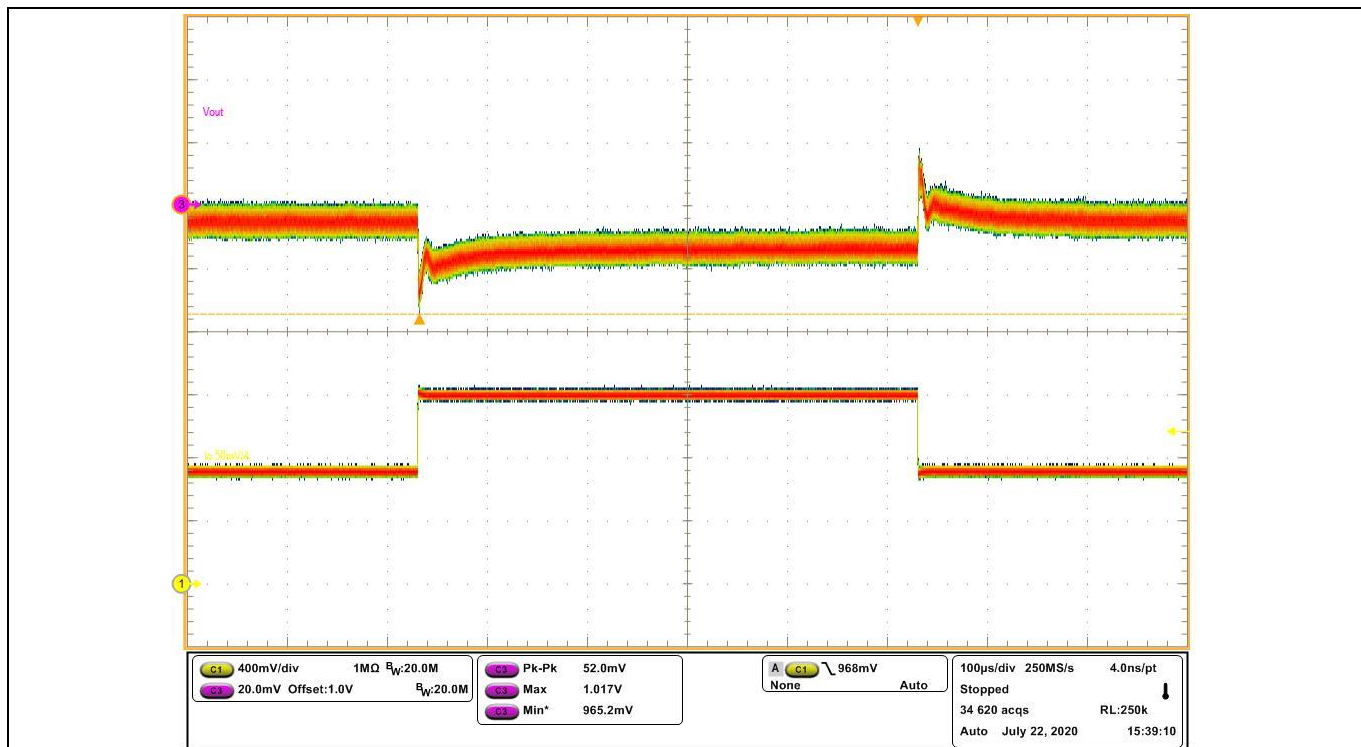
Figure 23 Transient response at 9 A step-load current at 30 A/μs slew rate: I_{out} = 16 \text{ A to } 25 \text{ A} (Ch 3 : V out , Ch 1 : I out ) pk-pk: 52 mV, f_{sw} = 800 \text{ kHz}
