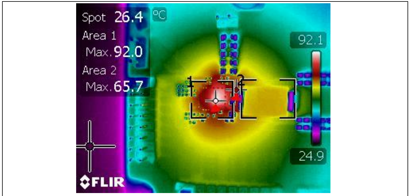
Figure 30 Thermal image of the board at 25 A load TDA38827 = 92°C, L = 65.7°C, f_{sw} = 800 kHz, T_a = room temperature, natural convection
