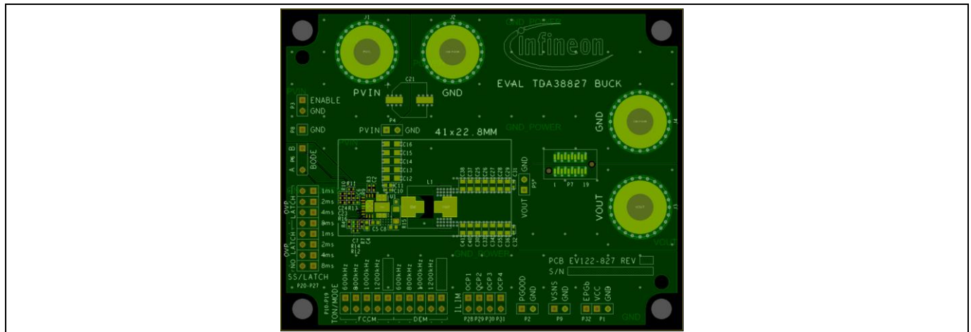
Figure 2 Top layer
