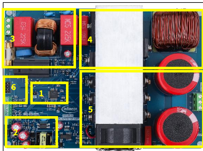
Figure 1 Functional groups of the EVAL-IKA15N65ET6 evaluation board, top side
