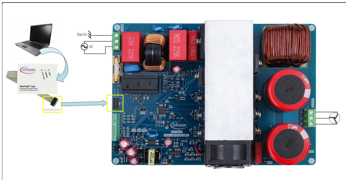
Figure 4 System connections using EVAL-IKA15N65ET6
