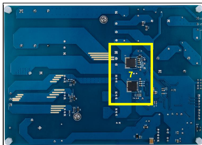
Figure 2 Functional groups of the EVAL-IKA15N65ET6 evaluation board, bottom side
