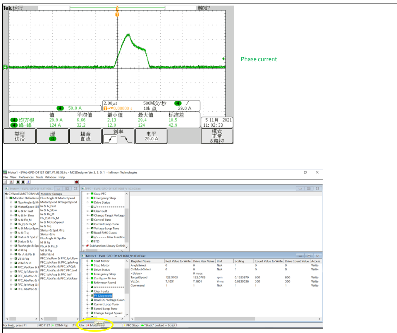
Figure 27 Inverter short-circuit protection
