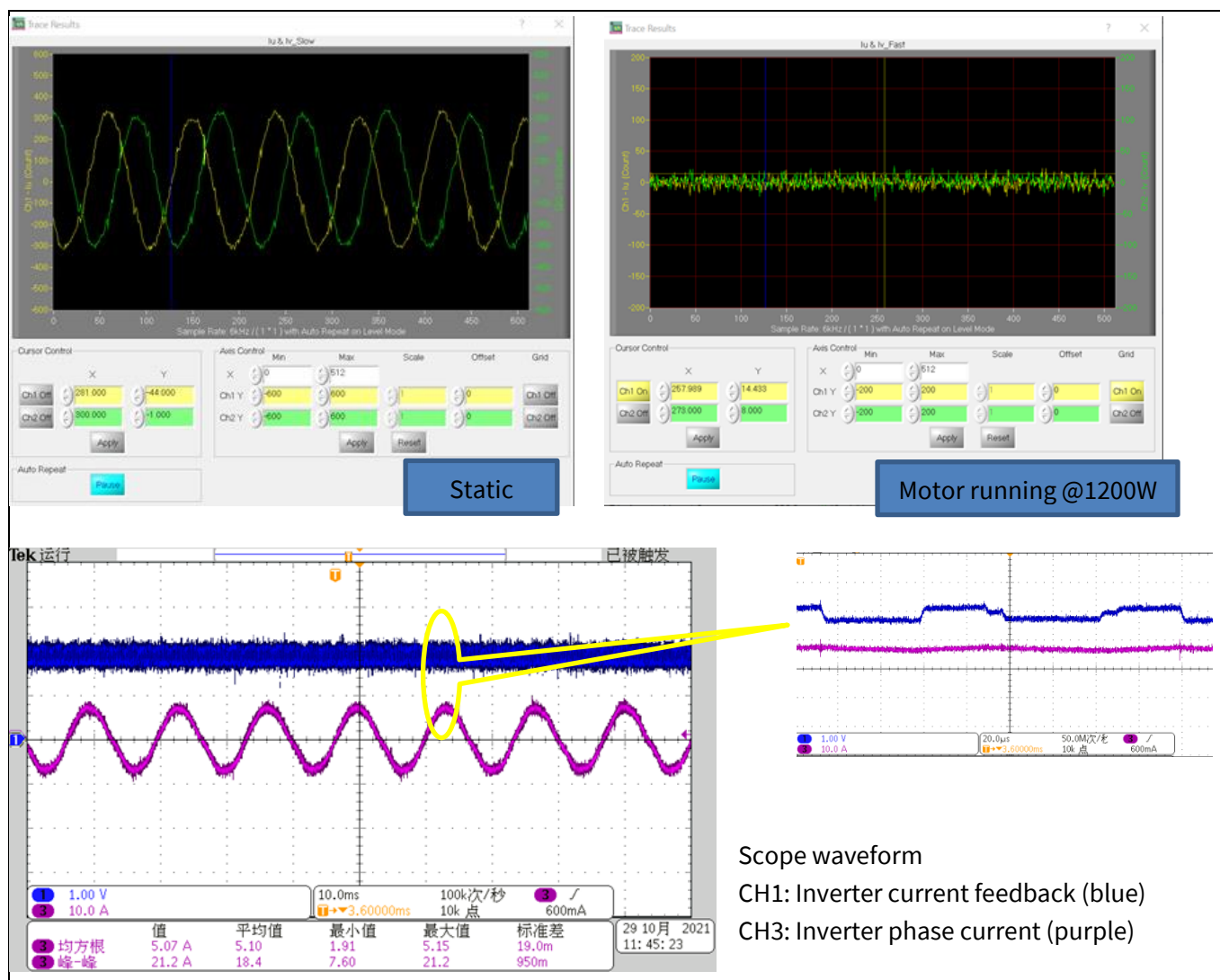
Figure 24 Inverter current waveforms
