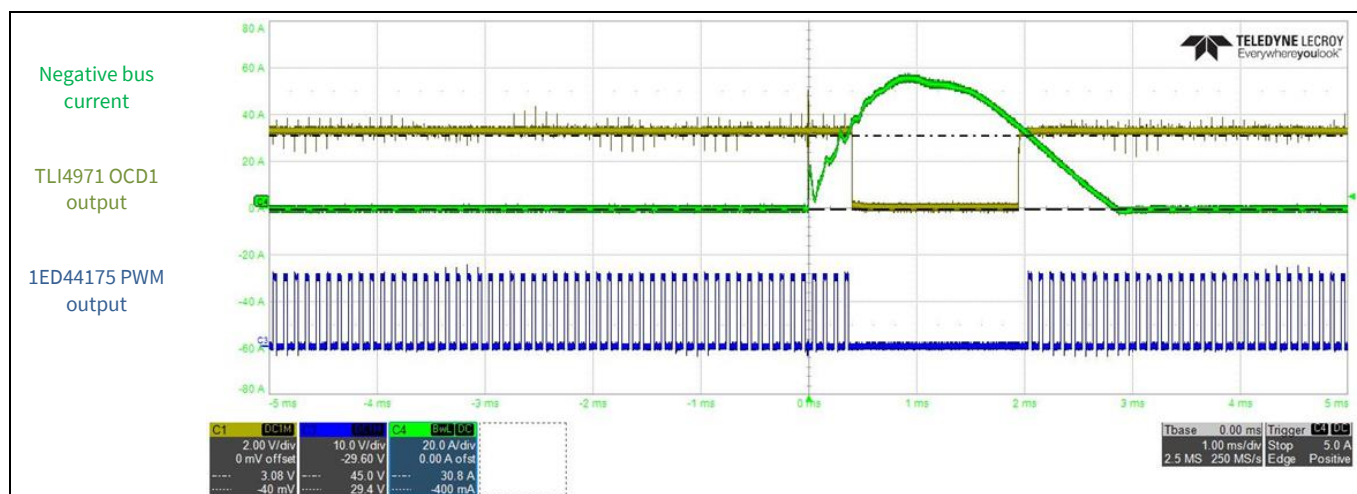
Figure 28 PFC overcurrent protection test
