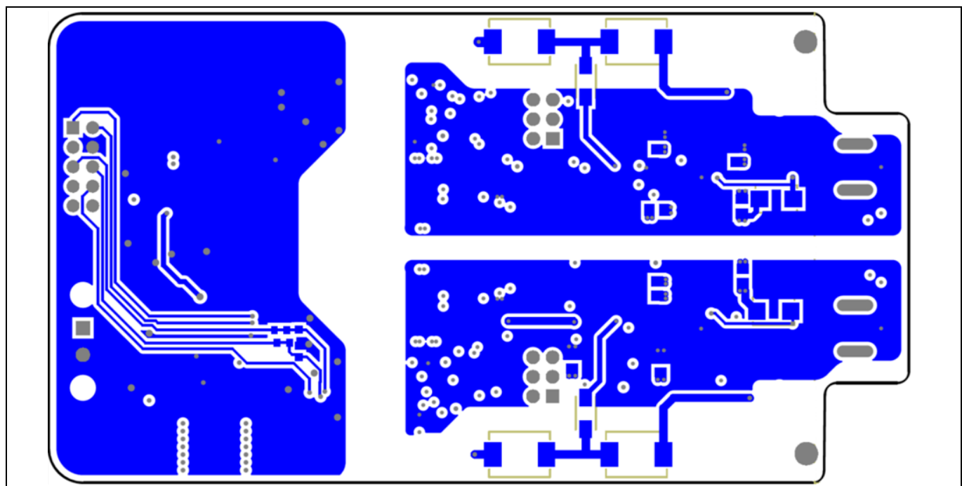
Figure 13 FFXMR20KM1DR with the bottom layer highlighted
