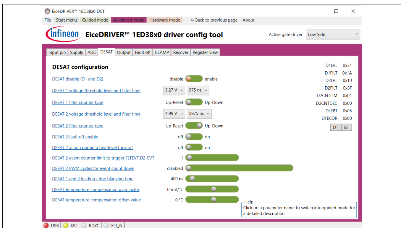
Figure 10 Example: DESAT configuration table of the advanced mode
