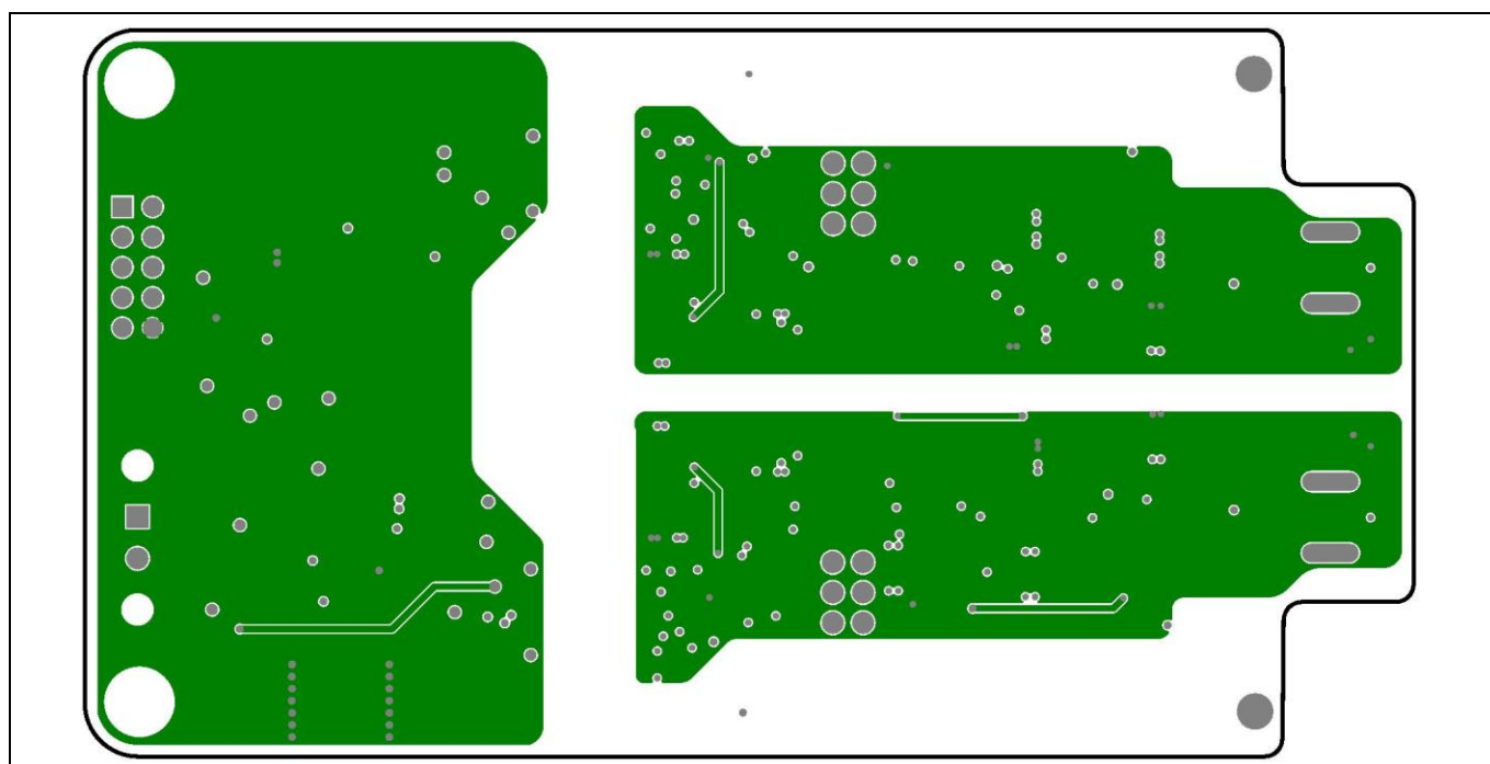
Figure 15 FFXMR20KM1DR with the internal layer 2 highlighted
