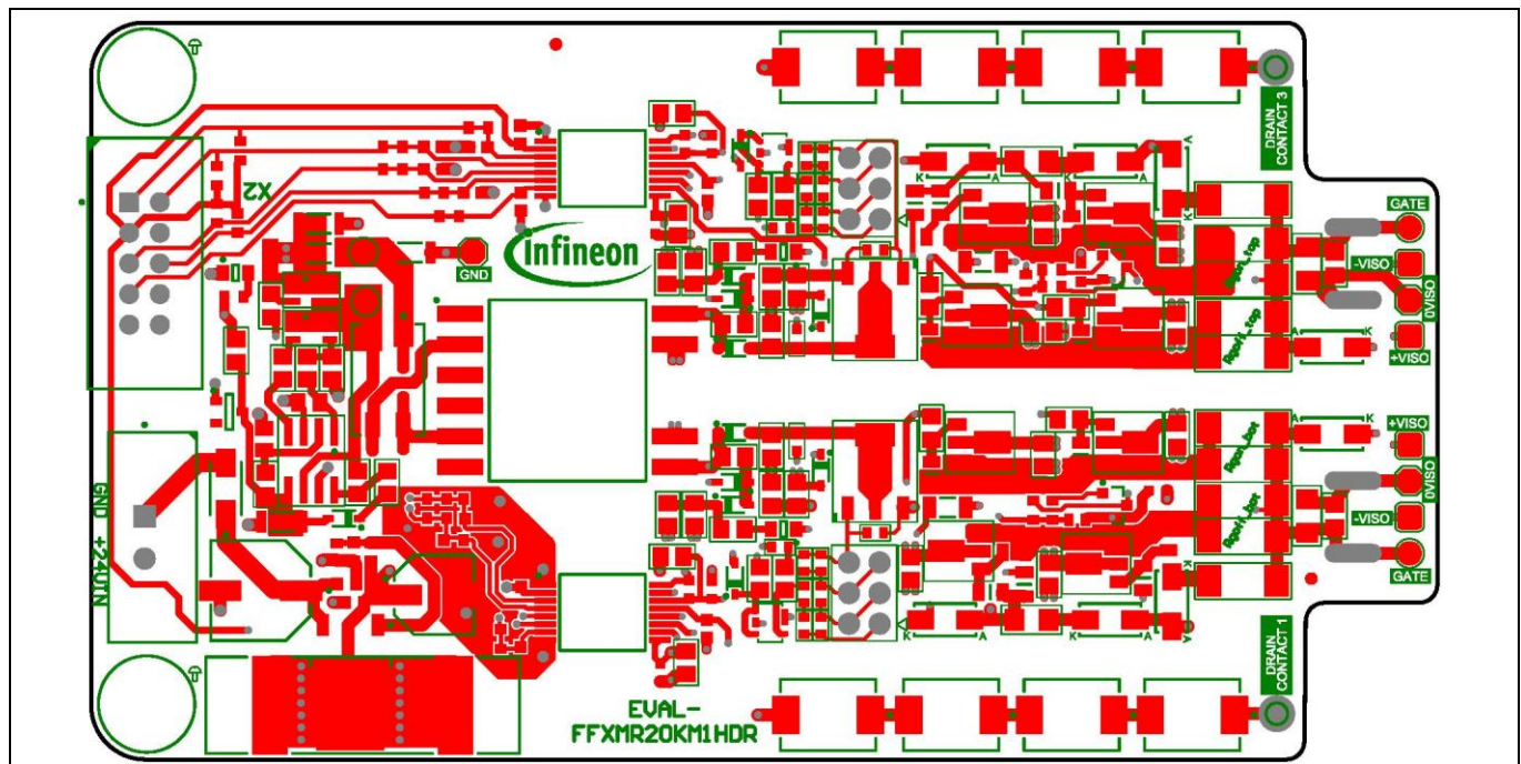
Figure 12 FFXMR20KM1DR with the top layer highlighted
