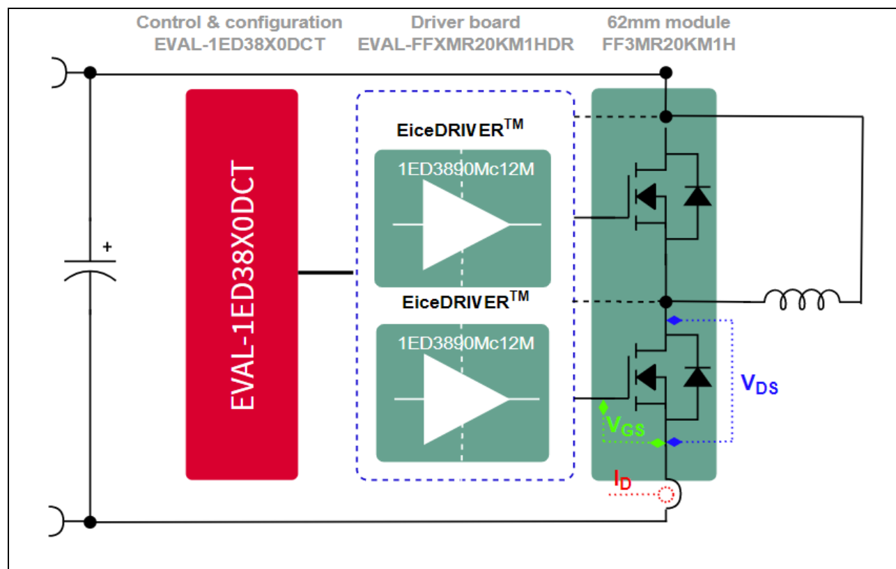
Figure 16 Test setup and voltage measurement techniques
