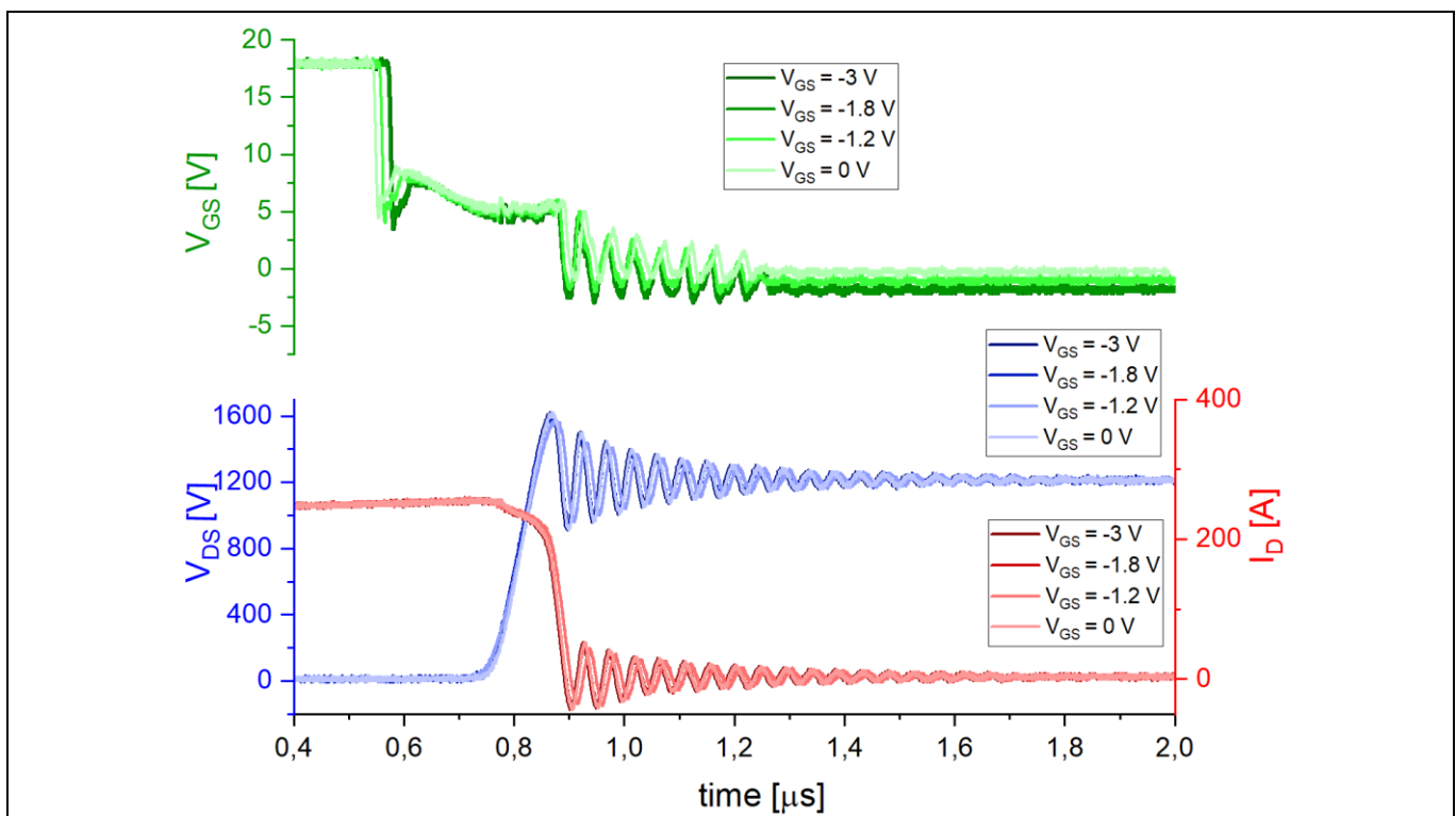
Figure 19 Turn-off waveforms with different ( V_{GS} = -3... 0 V / +18 V)
