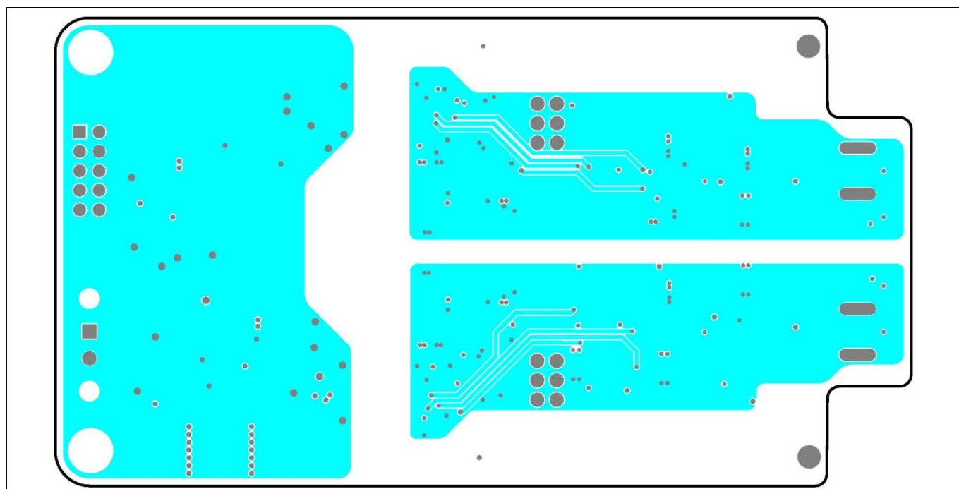
Figure 14 FFXMR20KM1DR with the internal layer 1 highlighted
