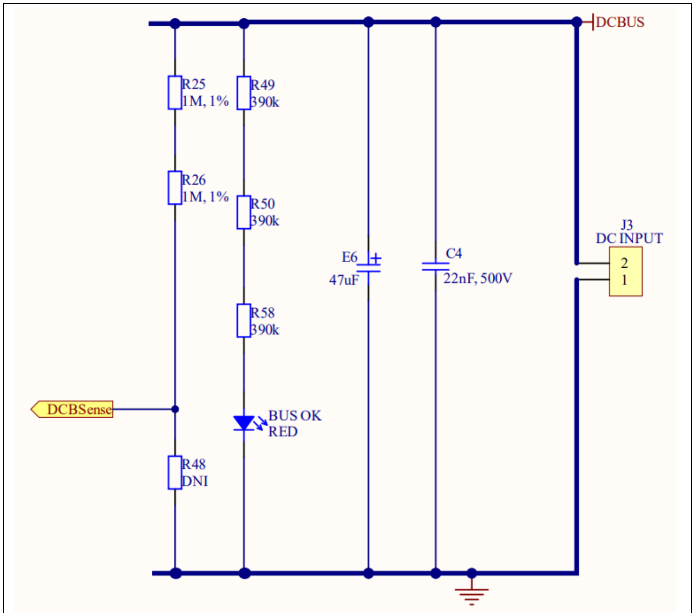
Figure 13 DC-Link schematic
