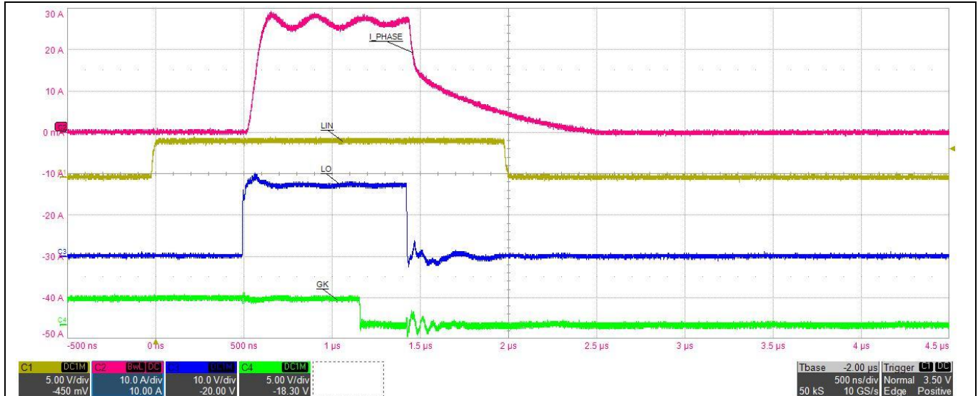
Figure 18 Short-circuit protection at V_{IN}=300V
