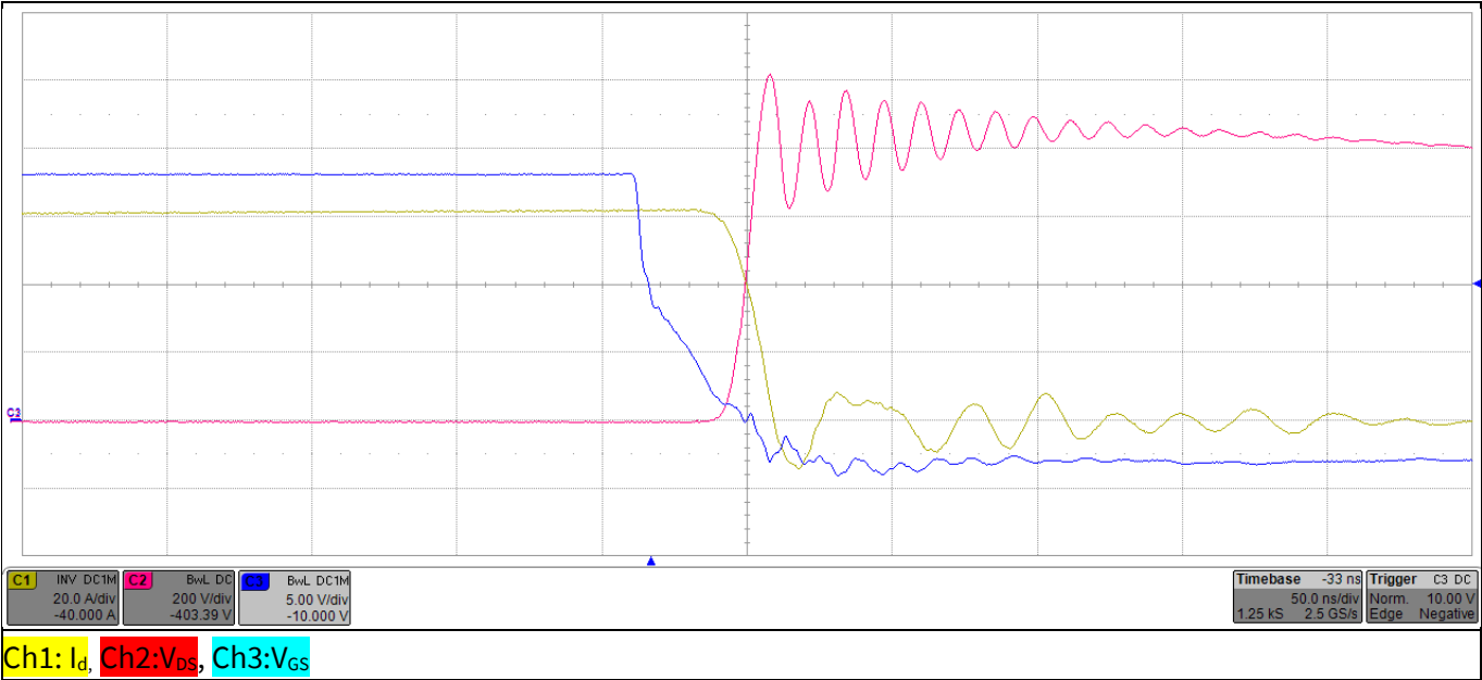
Figure 6 Eval-2ED3146MC12L-SiC – Turn-off of the low-side CoolSiC™ MOSFET
