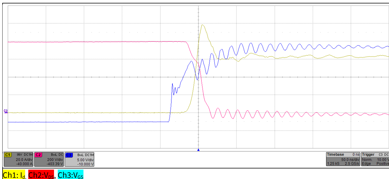
Figure 5 Eval-2ED3146MC12L-SiC – Turn-on of the low-side CoolSiC™ MOSFET
