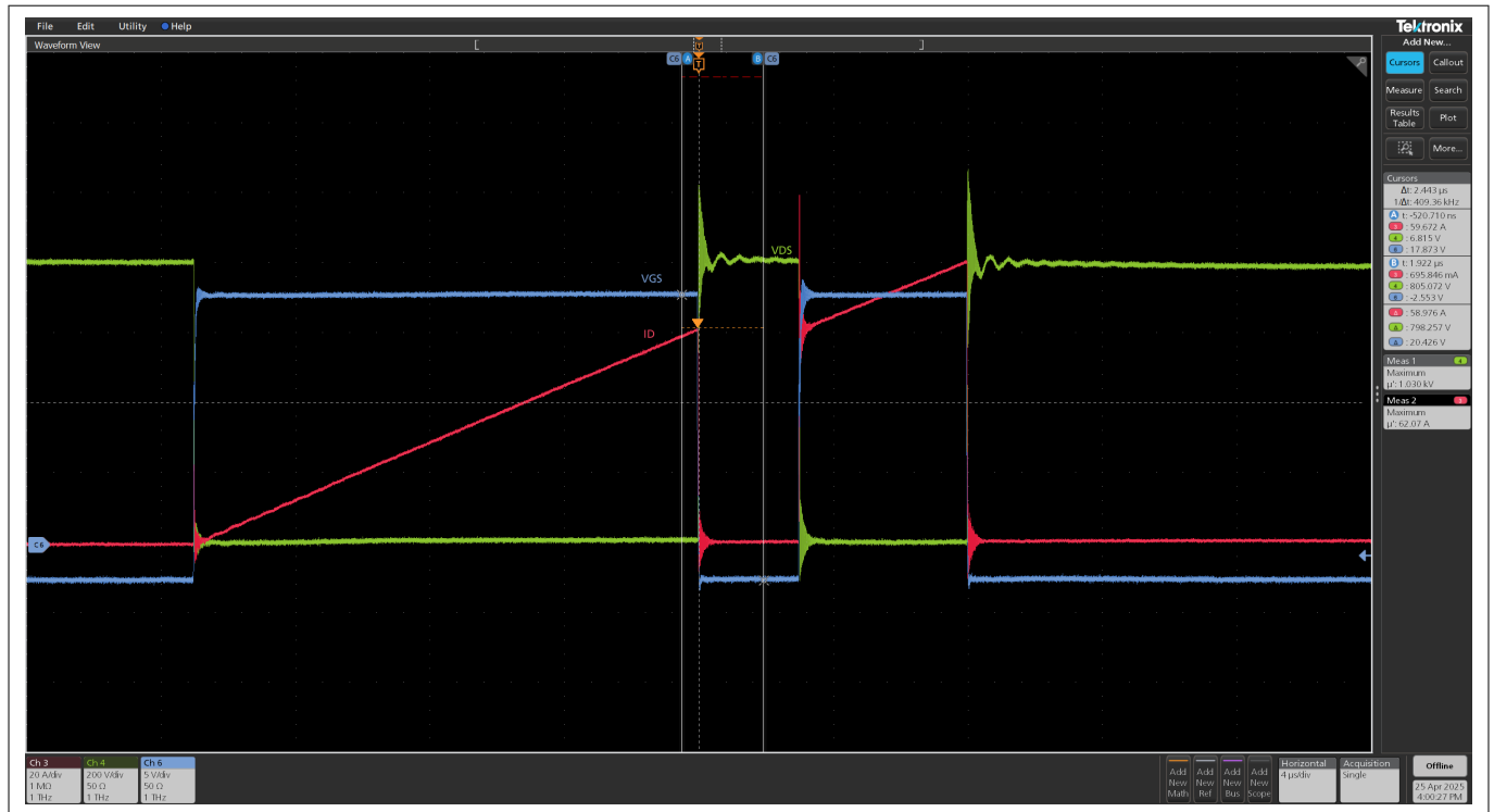
Figure 5 Eval-1ED3145MC12H-SiC– Double-pulse test of the low-side CoolSiC™ MOSFET
