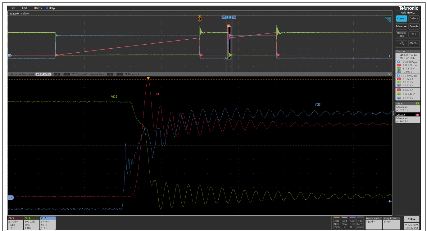
Figure 6 Eval-1ED3145MC12H-SiC– Turn-on of the low-side CoolSiC™ MOSFET
