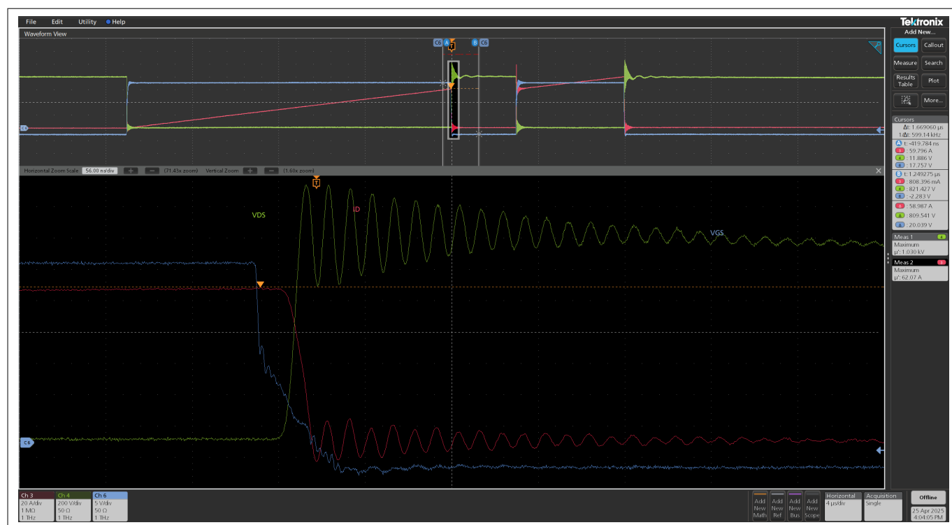
Figure 7 Eval-1ED3145MC12H-SiC– Turn-off of the low-side CoolSiC™ MOSFET
