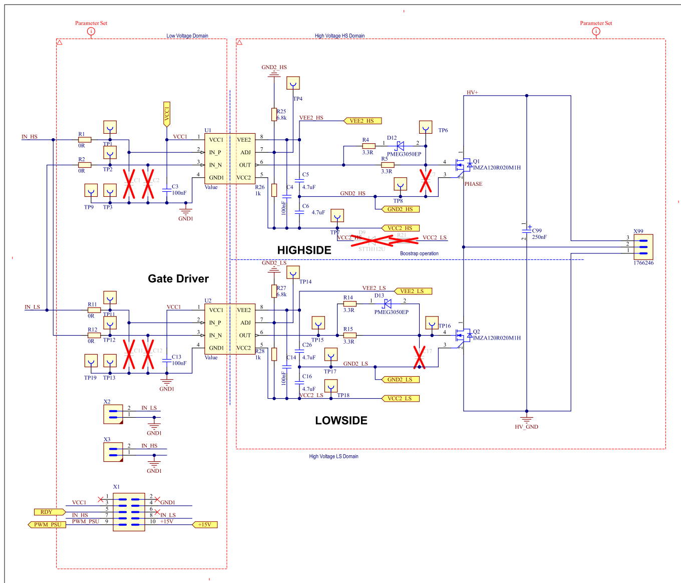
Figure 9 Gate driver circuit schematic
