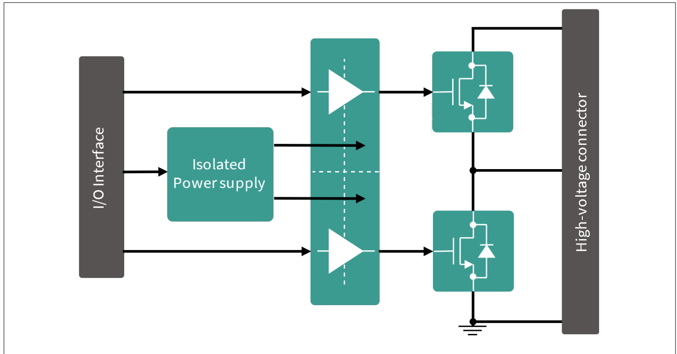
Figure 2 Eval-1ED3145MC12H-SiC evaluation board block diagram
