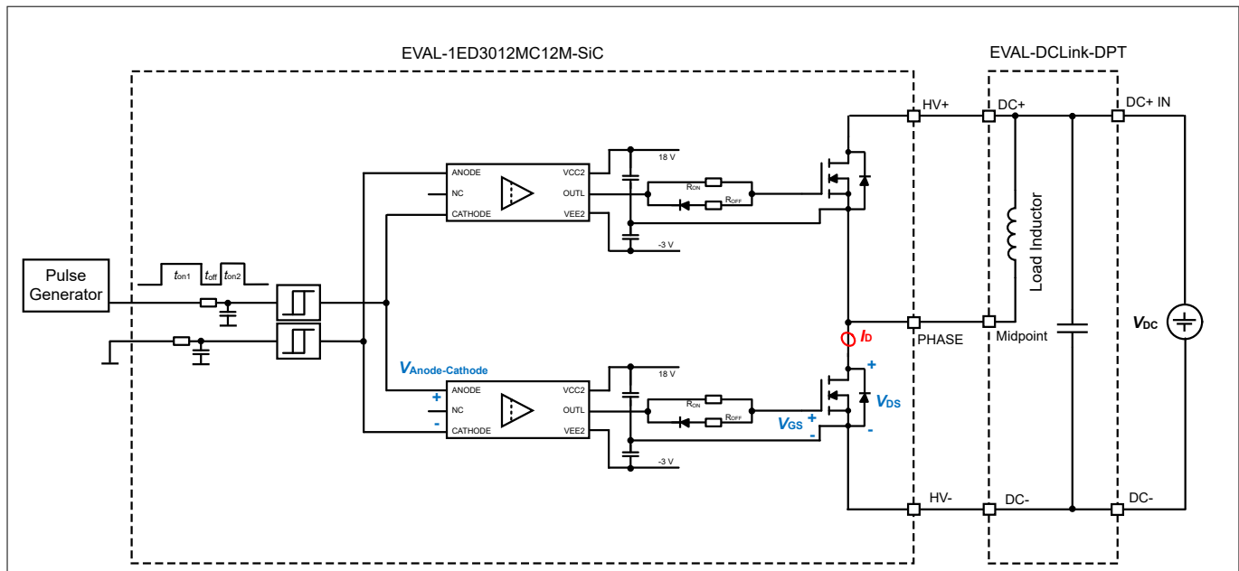
Figure 5 Measurement setup for the double-pulse test
