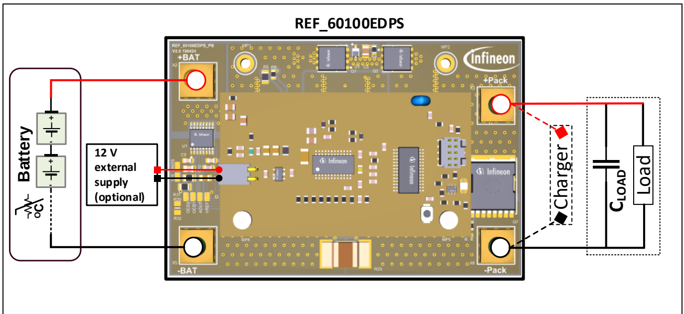
Figure 5 REF_EDPS setup in the application
