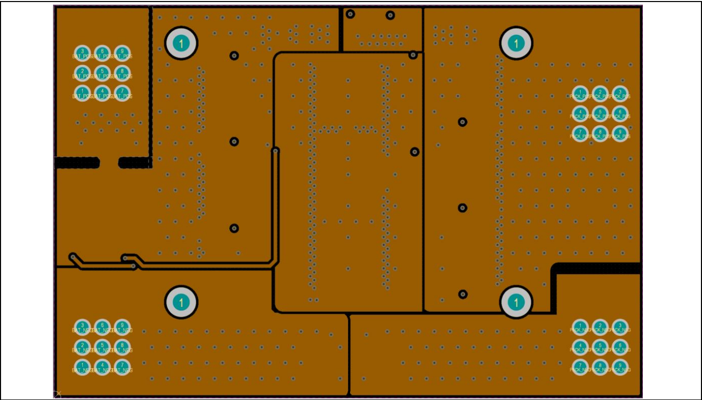
Figure 15 REF_60100EDPS_PB layer 2
