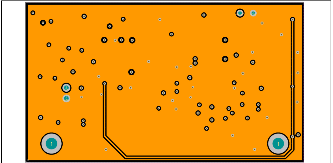
Figure 19 REF_60100EDPS_CB layer 2
