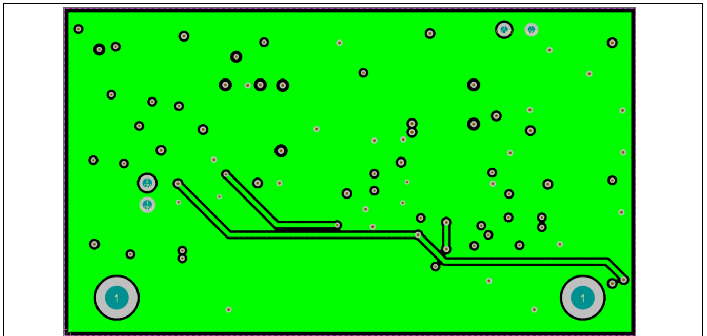
Figure 20 REF_60100EDPS_CB layer 3
