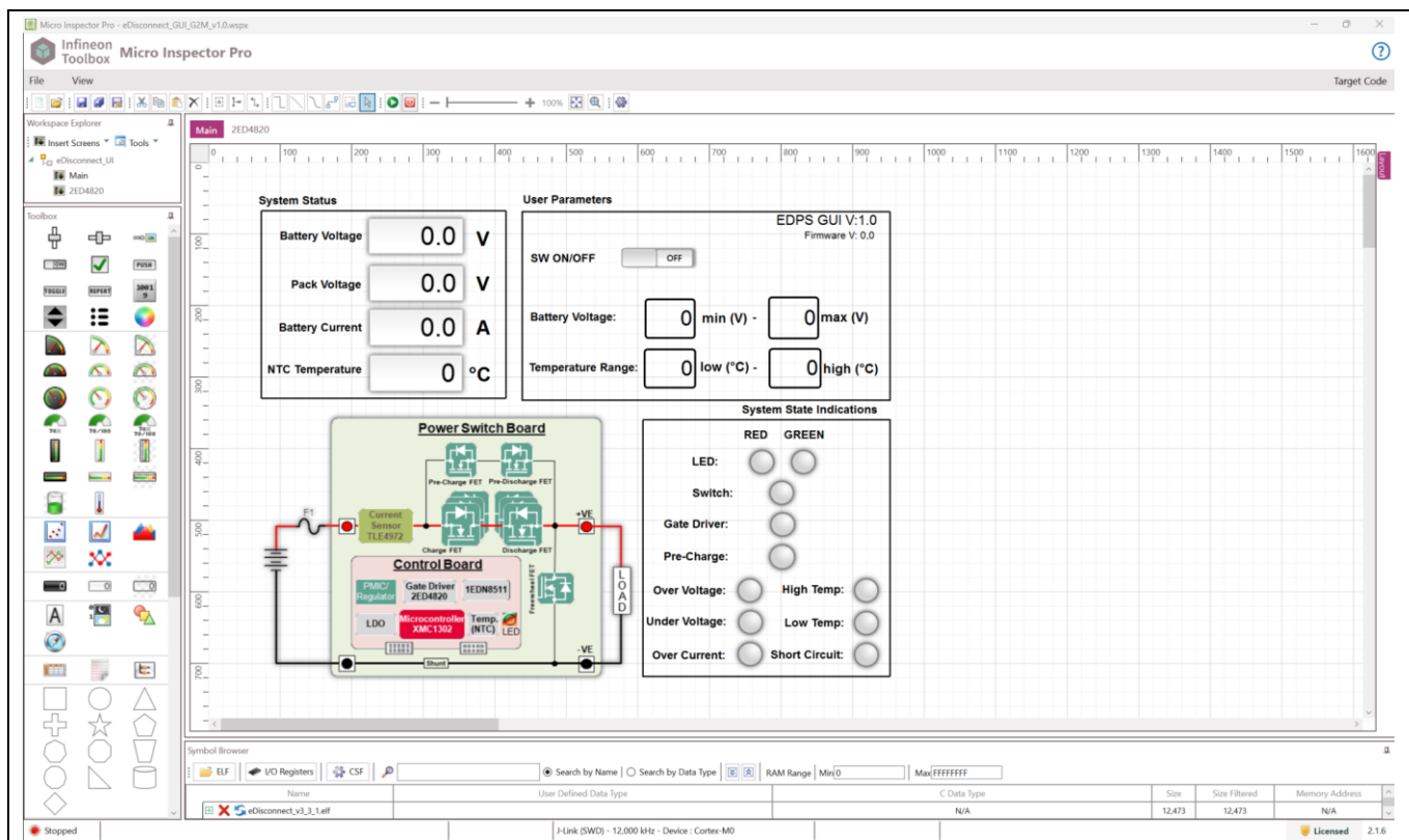
Figure 23 User interface control design in Micro Inspector Pro
