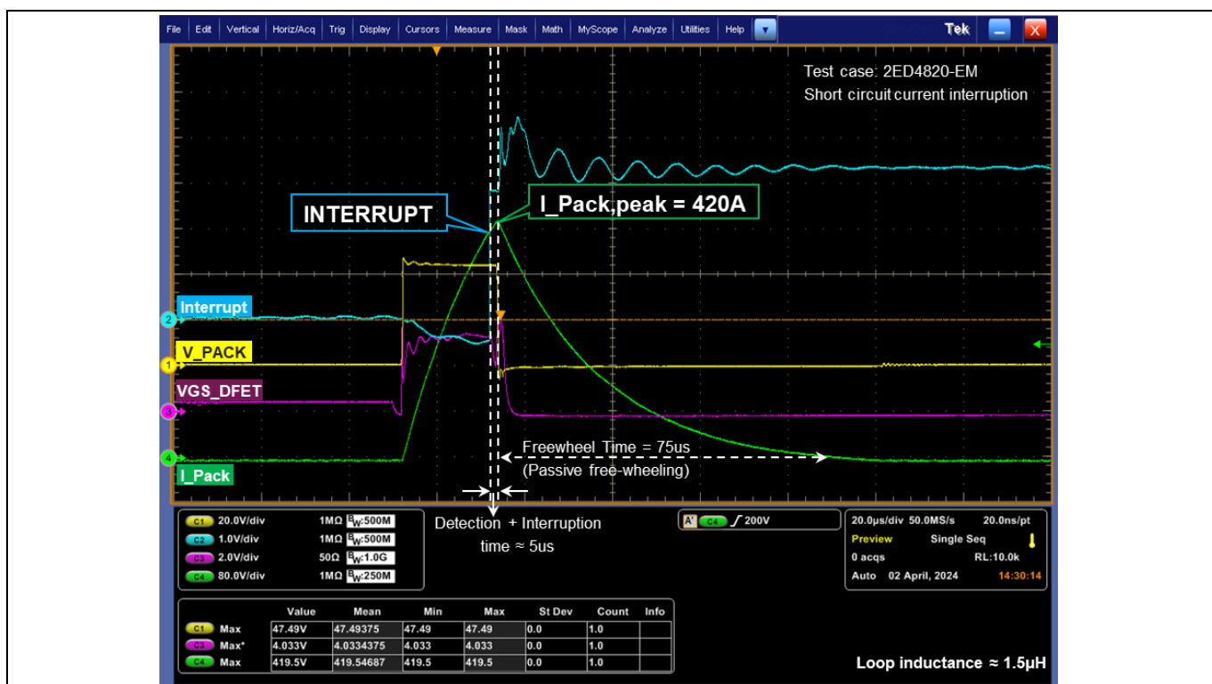
Figure 31 Short-circuit current interruption by 2ED4820-EM
