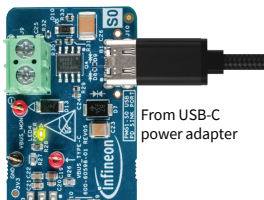
Powering the CY7110 board
