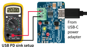
USB PD sink setup
