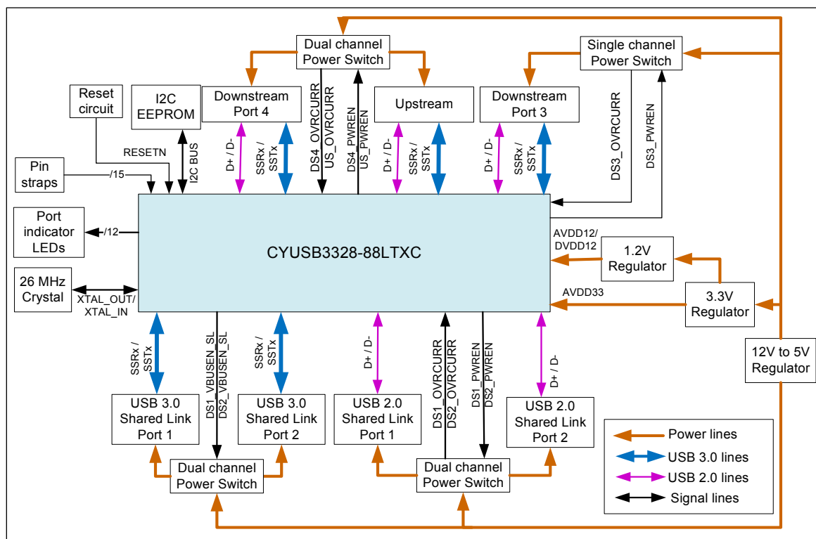
Figure 5-14. CY4613 Hardware Block Diagram
