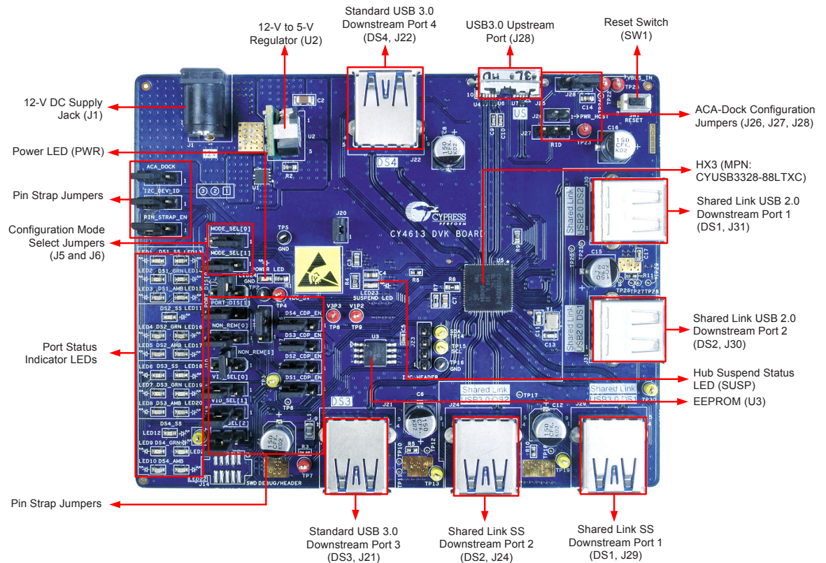
Figure 3-7. CY4613 Board (Top Side)
