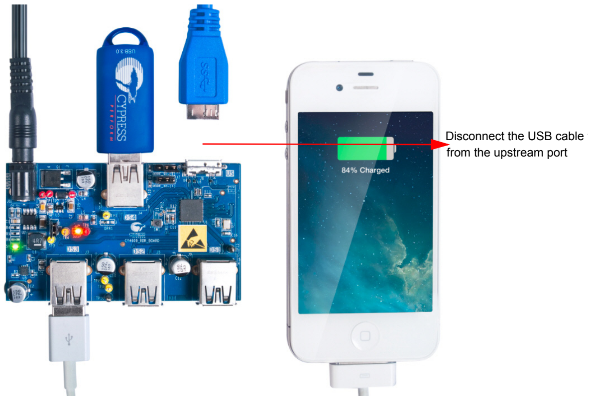
Figure 3-21. Ghost Charging
