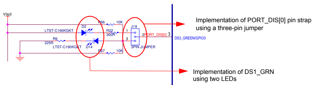
Figure 3-18. Port Status Indicator LEDs Using Shared GPIOs
