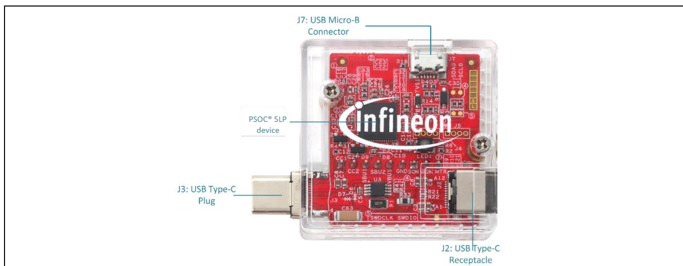
Figure 2 CY4500-EPR EZ-PD™ Protocol Analyzer board (front view)
