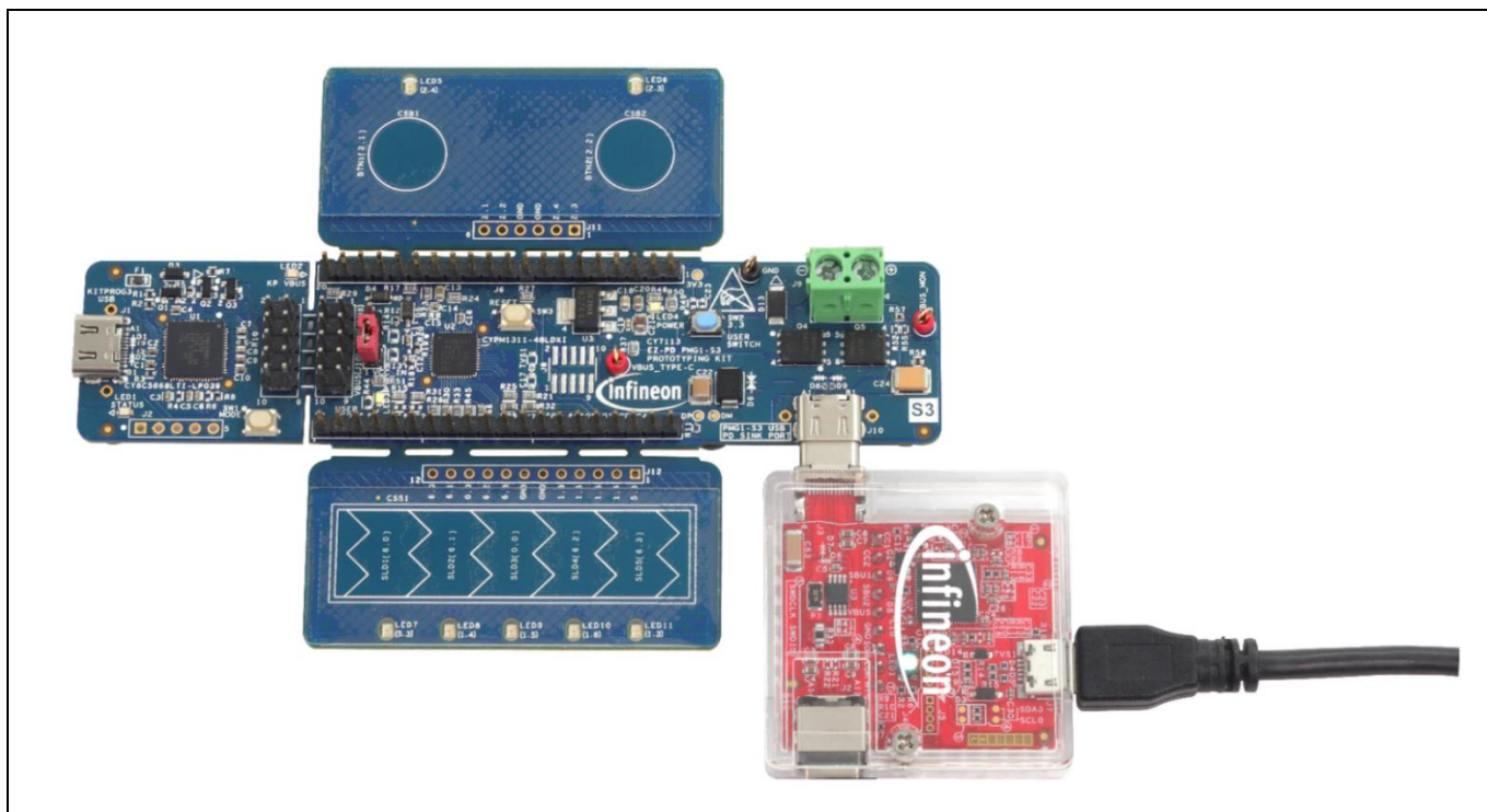
Figure 11 Setup for operating CY4500-EPR EZ-PD™ Protocol Analyzer
