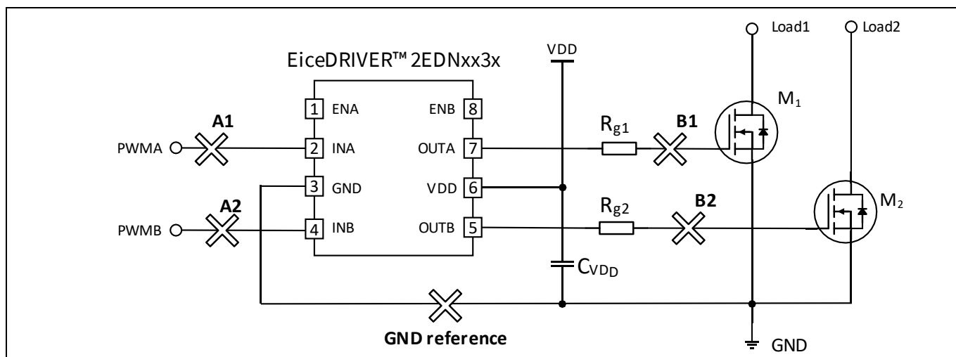
Figure 5 Probing points to verify the driving behavior of A1, A2, B1 and B2
