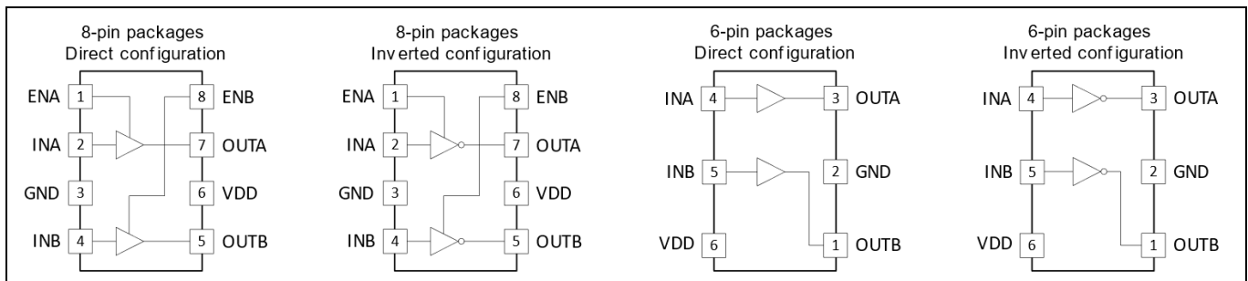
Figure 4 Input configurations
