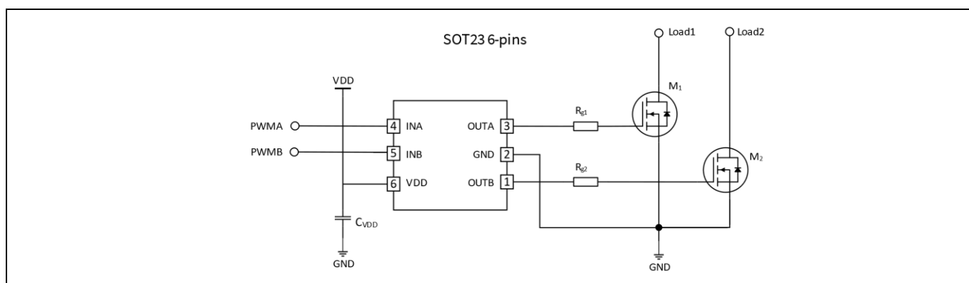
Figure 2 Application example: SOT-23-6 package
