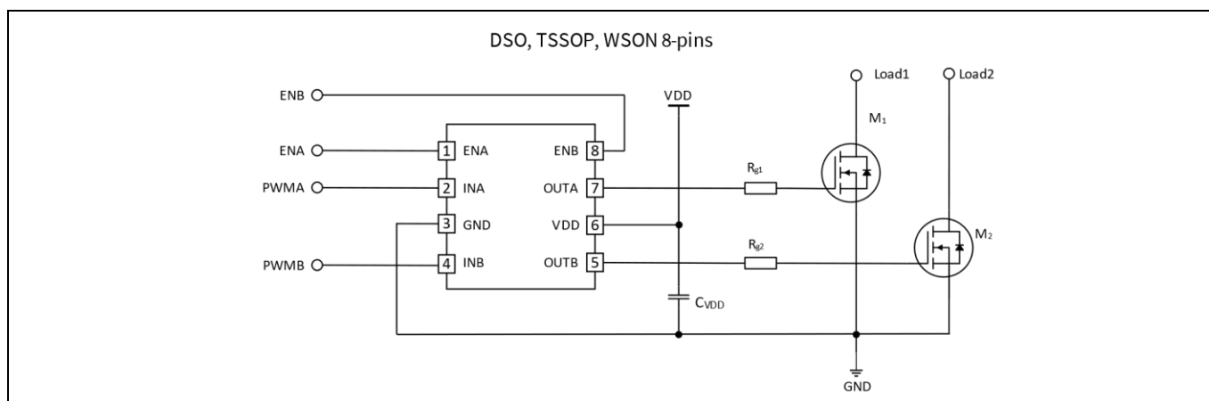
Figure 1 Application example: DSO-8, TSSOP-8 and WSON-8 packages
