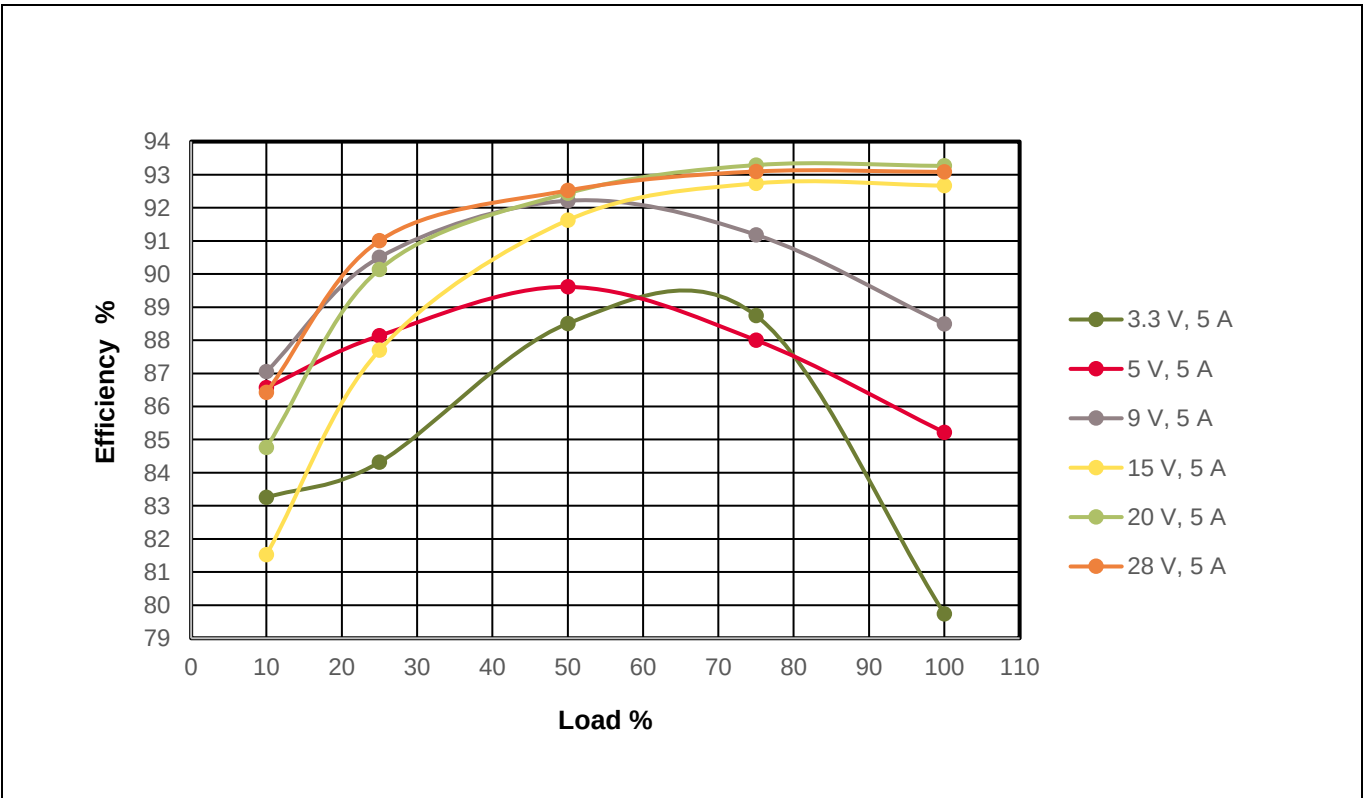
Figure 5 Efficiency at 115 V ac /60 Hz
