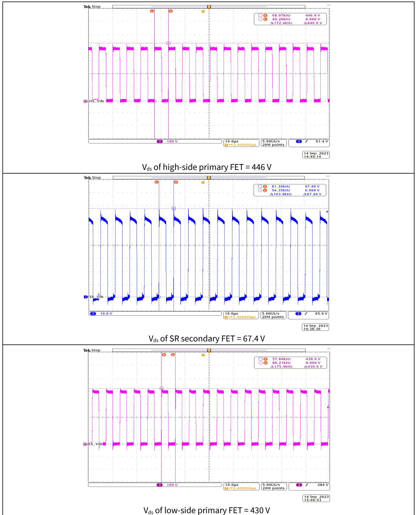
Figure 35 Drain-source voltage stress of different FETs at V_{in} = 265 V_{ac}/63 \text{ Hz} , V_{out} = 28 \text{ V} , I_{out} = 5 \text{ A}
