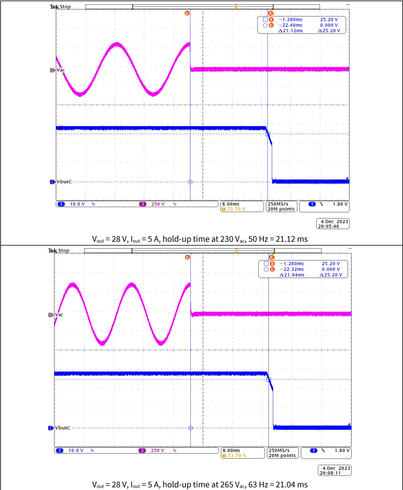
Figure 33 Hold-up time at various AC inputs (CH1: V bus_C , CH3: V in_AC )
