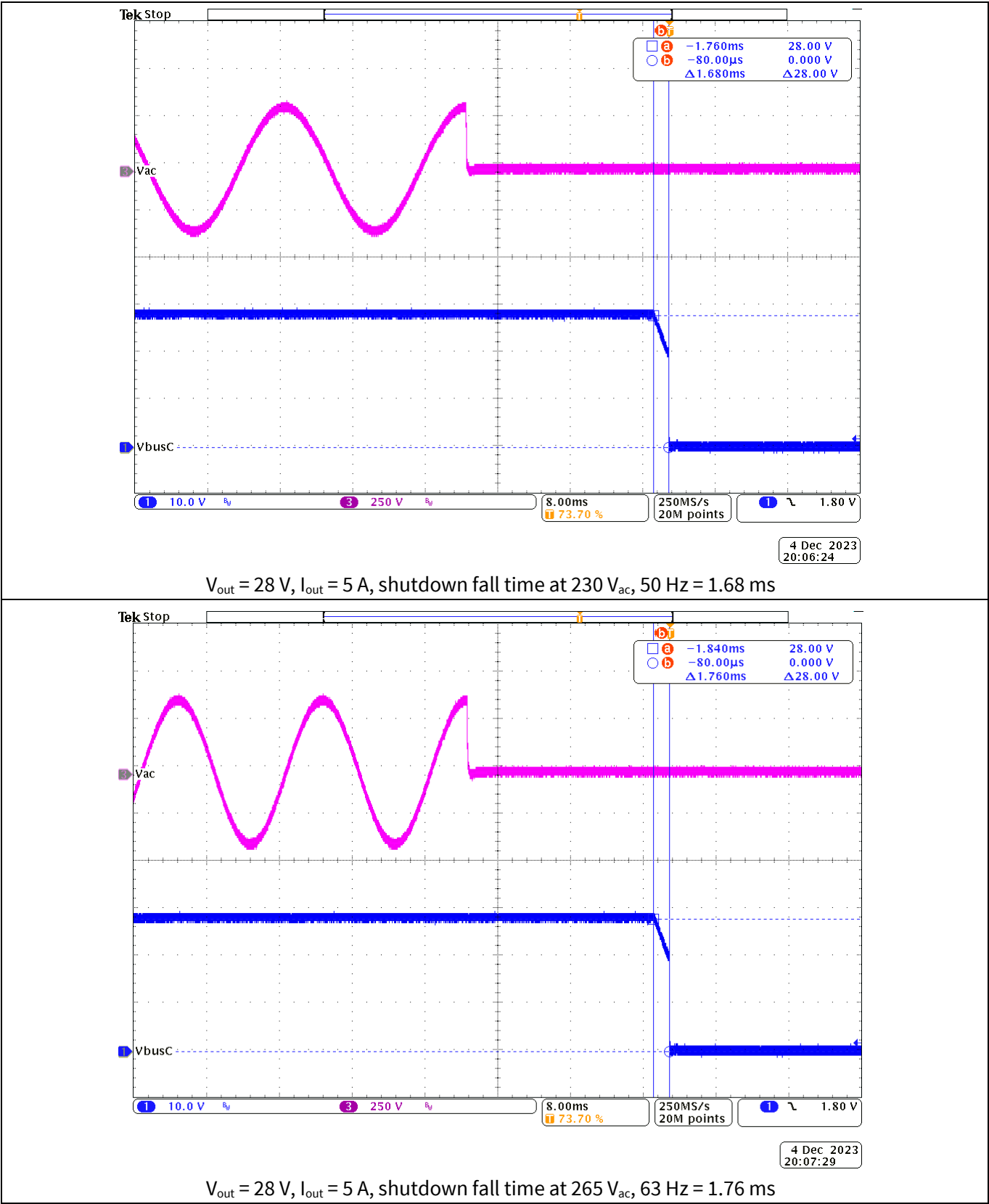
Figure 34 Shutdown fall time at various AC inputs (CH1: V bus_C , CH3: V in_AC )
