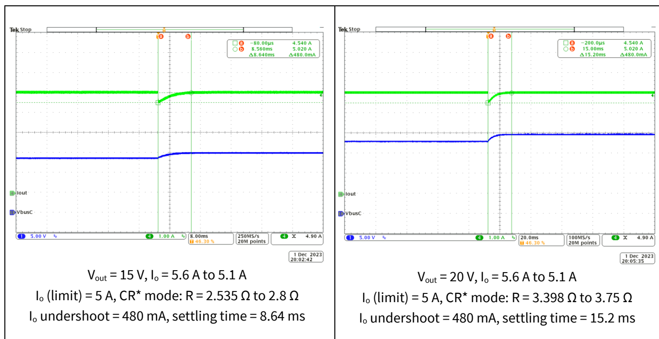
Figure 27 Output current undershoot and settling time at V ac = 230 V ac , 50 Hz (CH1: V bus_C , CH4: I out )
