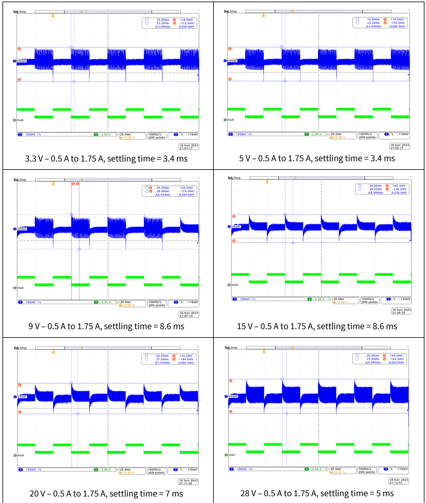
Figure 16 Output dynamic response at V_{ac} = 115 V_{ac} , 60 Hz, load transition = 10% to 35%, T_1 = 20 ms, T_2 = 20 ms, slew rate = 0.5 A/ \mu s, (CH1: V bus_C , Ch4: I out )
