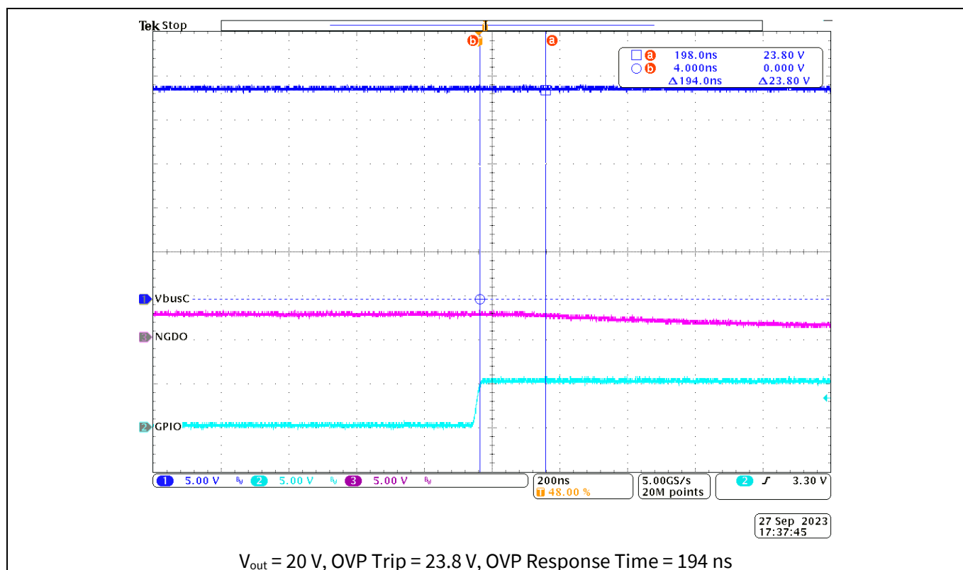
Figure 40 Overvoltage protection trip point and response time at 115 V_{ac} , 60 Hz (CH1: V_{bus\_c} , CH2: GPIO9, CH3: NDGO = Provider FET Q2 gate-source)
