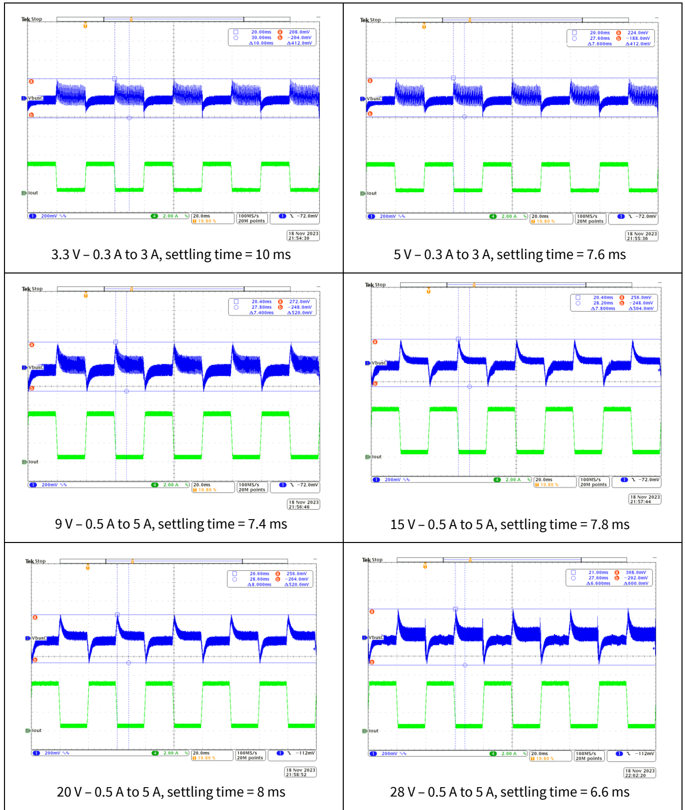
Figure 21 Output dynamic response at V_{ac} = 230 V_{ac} , 50 Hz, T_1 = 20 ms, T_2 = 20 ms, Slew Rate = 3.2 \text{ mA}/\mu\text{s} (CH1: V_{bus\_C} , Ch4: I_{out} )
