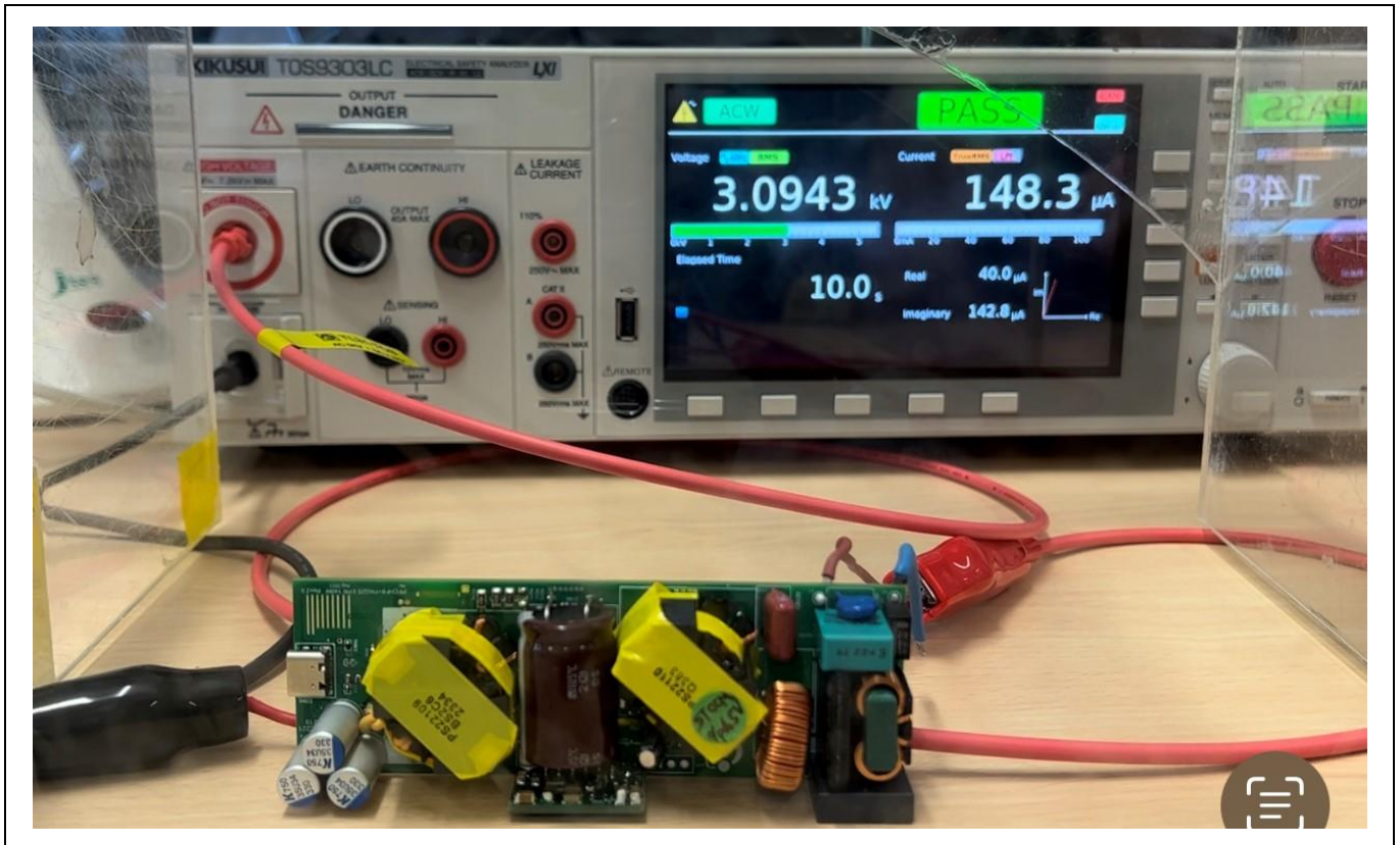
Figure 55 Hi-Pot test setup
