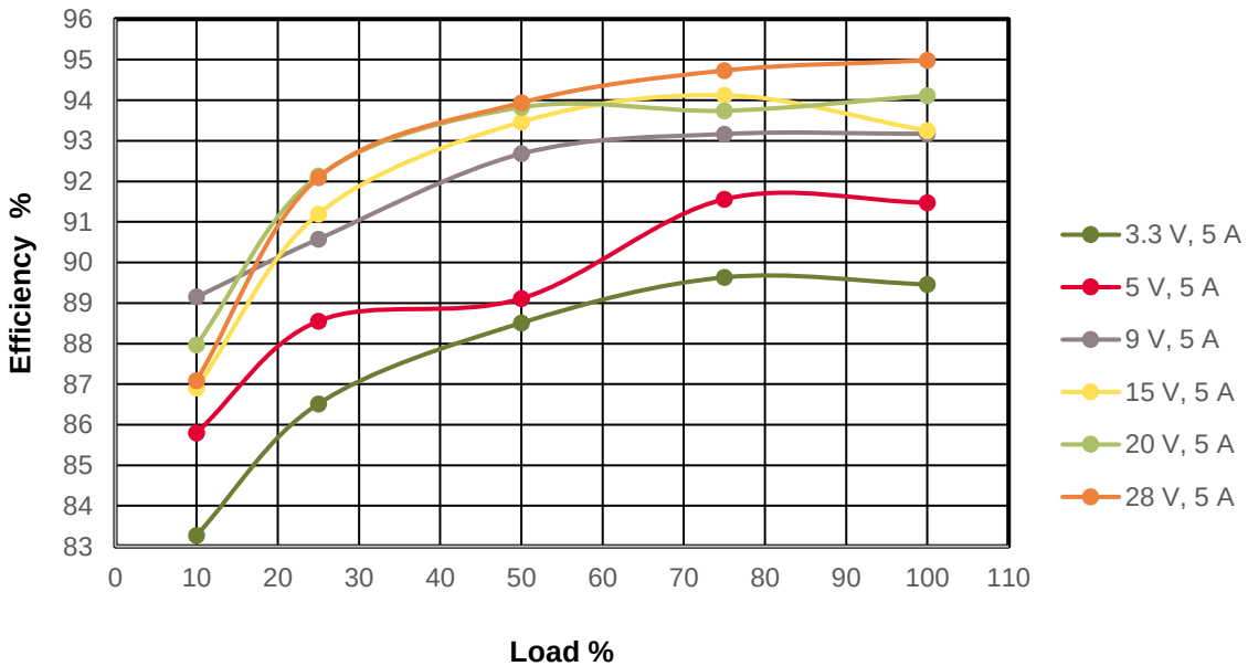
Figure 7 Efficiency at 265 V ac /63 Hz
