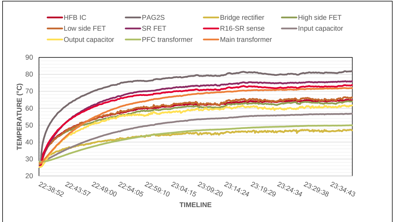
Figure 45 Thermal log with time ( V_{ac} = 265 V_{ac}/63 \text{ Hz} , V_{out} = 28 V , I_{out} = 5 A )
