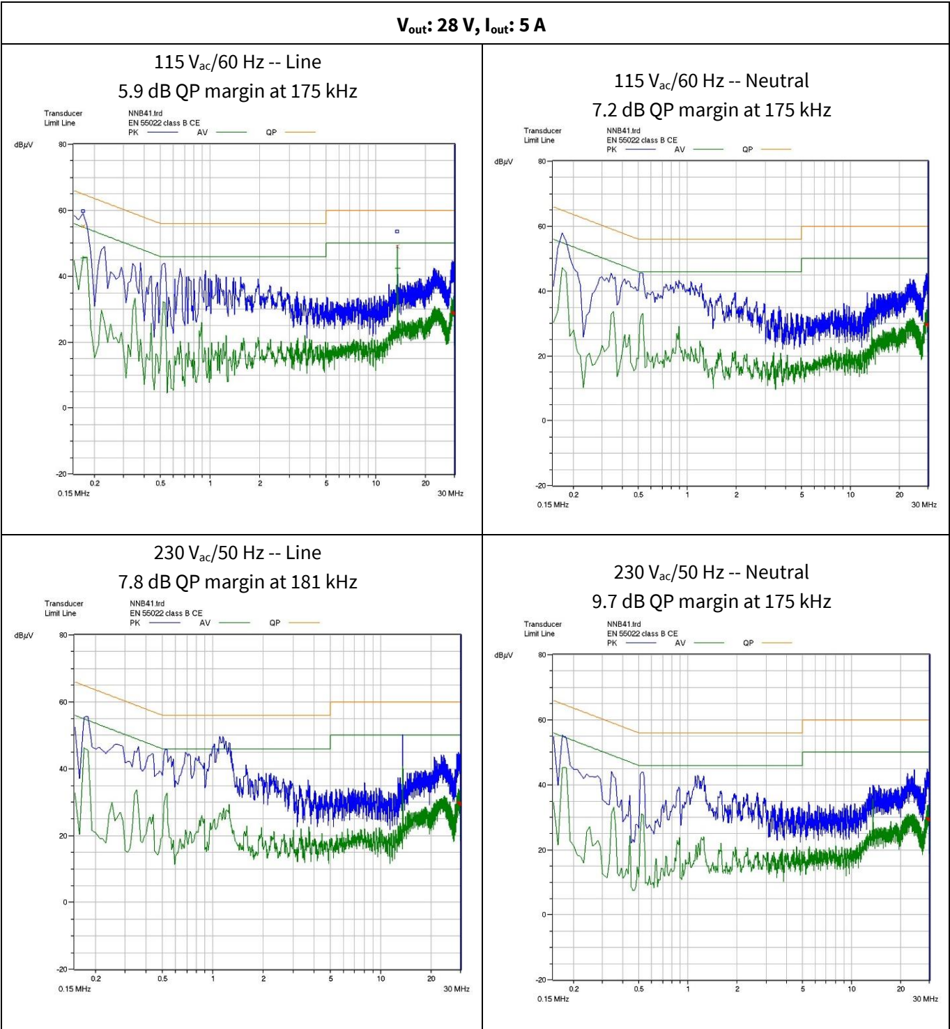
Figure 54 Conducted emissions EMI test results
