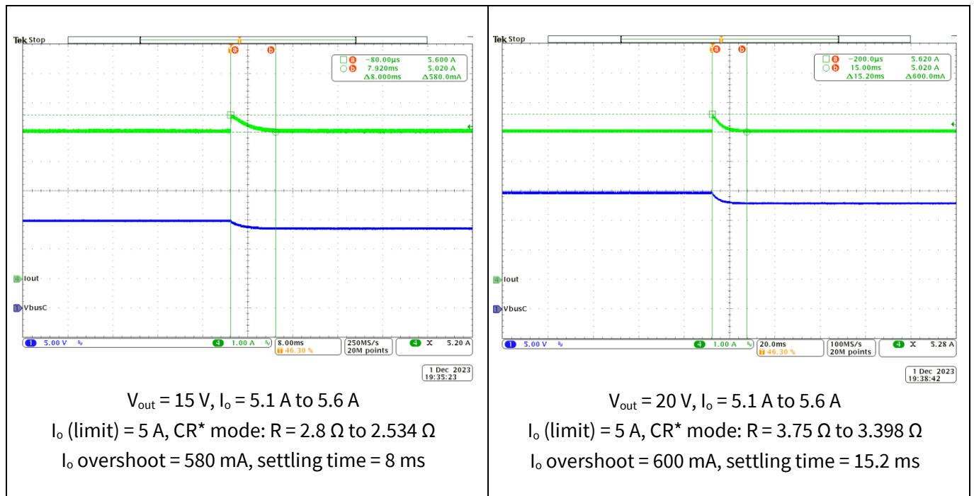
Figure 24 Output current overshoot and settling time at V_{ac} = 115 \text{ V}_{ac} , 60 Hz (CH1: V_{bus\_C} , CH4: I_{out} )
