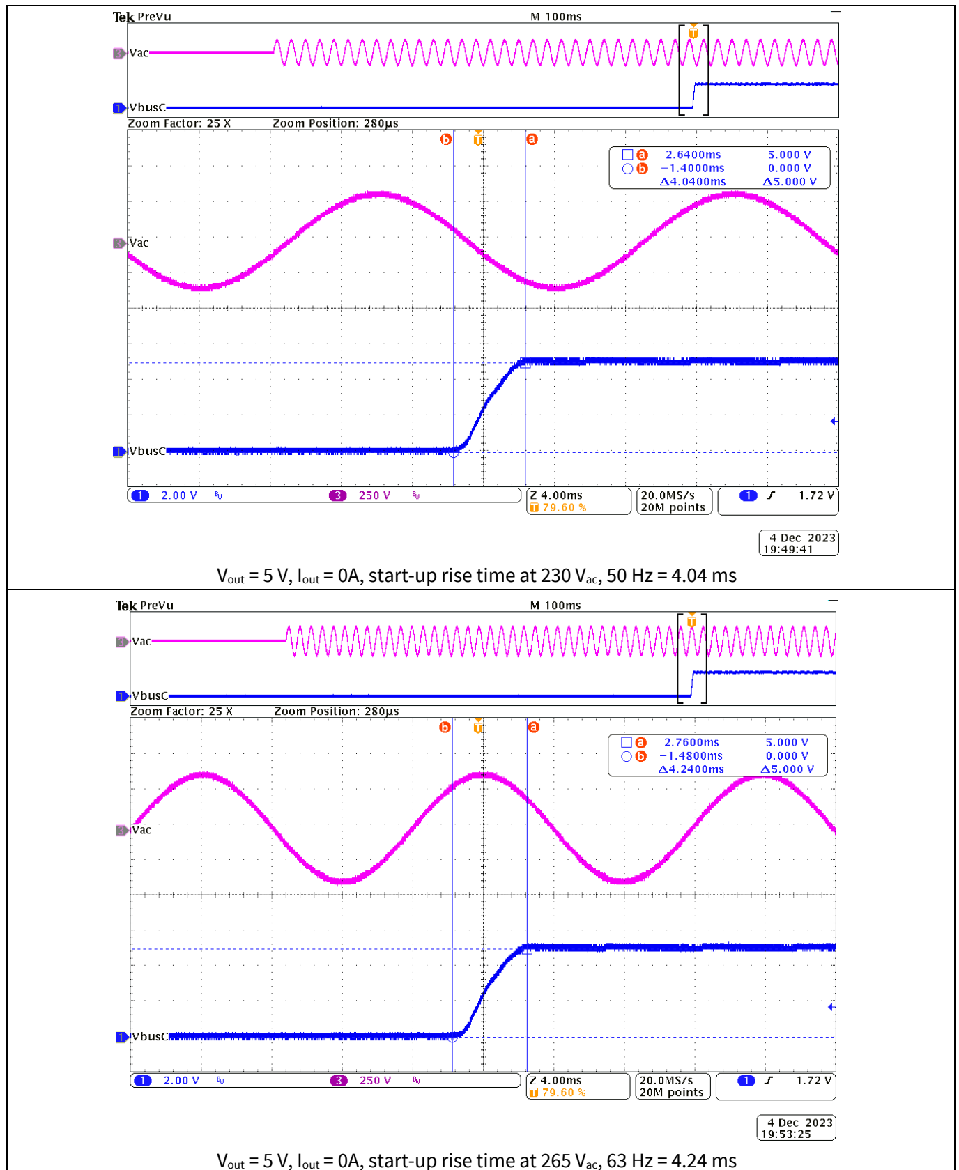
Figure 31 Start-up rise-time at various AC inputs (CH1: Vbus_C, CH3: Vin_AC)
