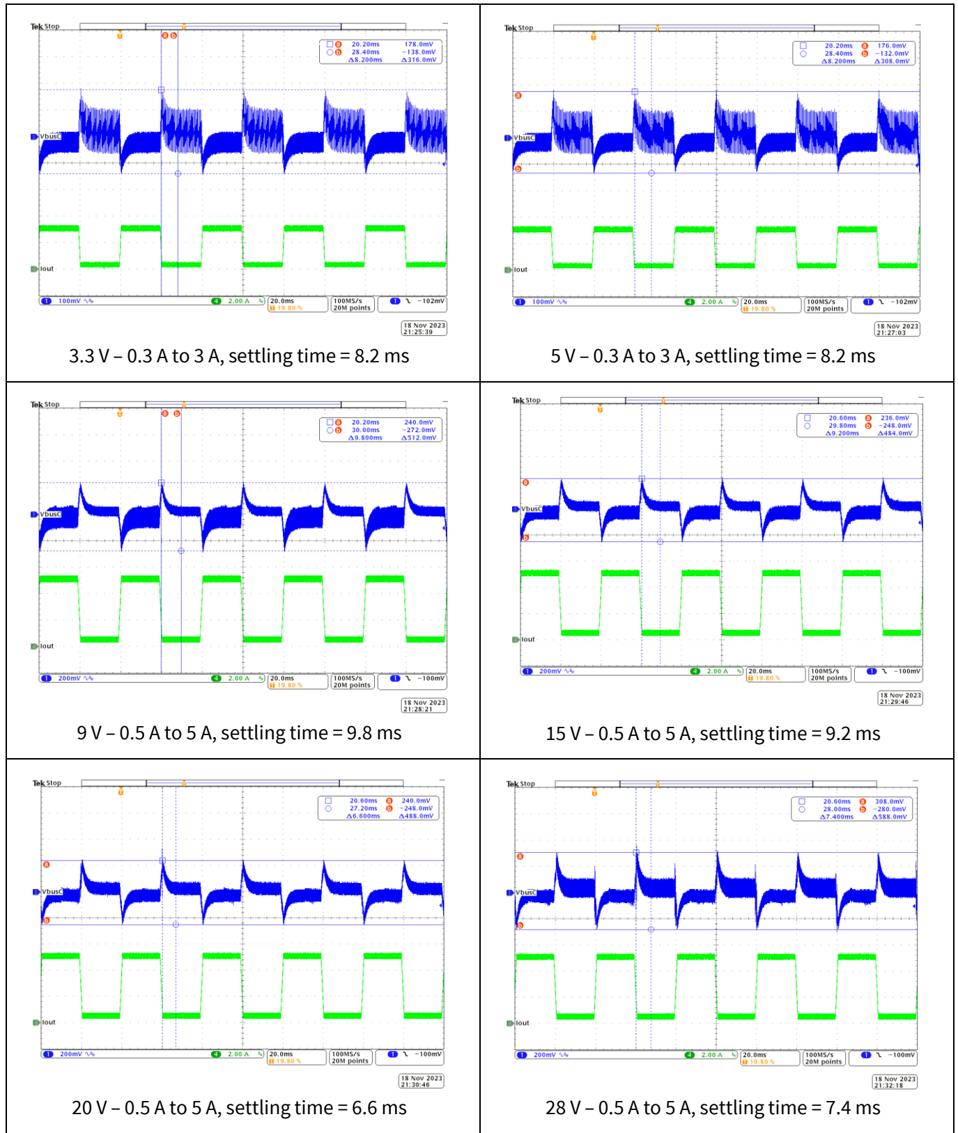
Figure 20 Output dynamic response at V_{ac} = 115 V_{ac} , 60 Hz, T_1 = 20 ms, T_2 = 20 ms, Slew Rate = 3.2 mA/ \mu s (CH1: V_{busC} , Ch4: I_{out} )
