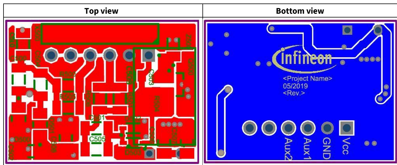
Figure 62 Daughter board
