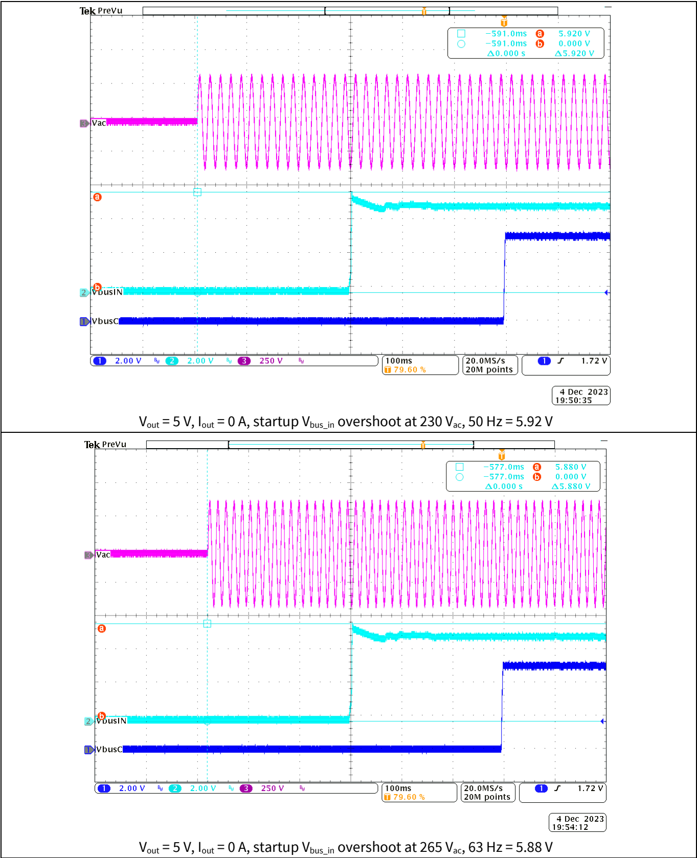
Figure 32 Start-up V_{bus\_in} overshoot at various AC inputs (CH1: V_{bus\_C} , CH2: V_{bus\_in} , CH3: V_{in\_AC} )
