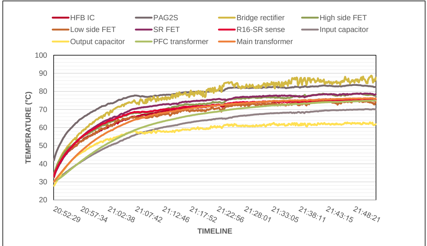
Figure 44 Thermal log with time ( V_{ac} = 90 V_{ac}/47 \text{ Hz} , V_{out} = 28 \text{ V} , I_{out} = 5 \text{ A} )
