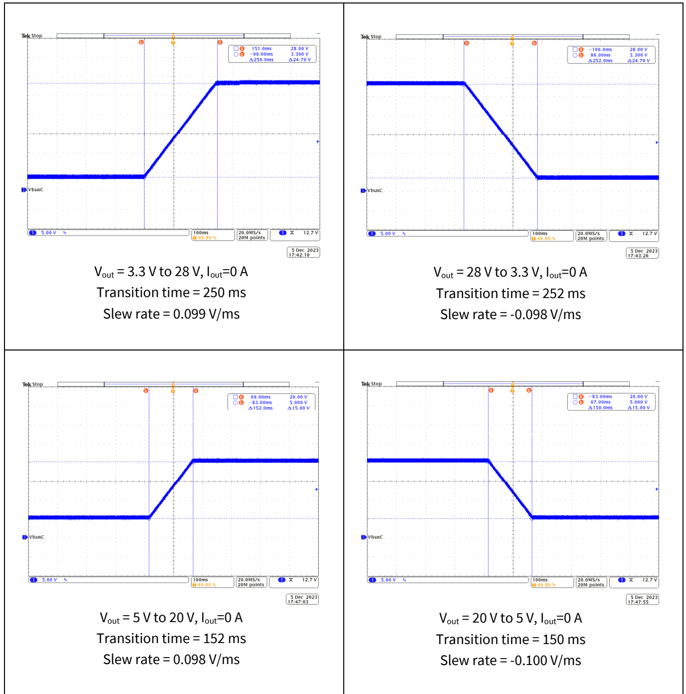
Figure 23 Output voltage transition at V_{ac} = 230 \text{ V}_{ac} , 50 Hz (CH1: V_{bus\_c} )
