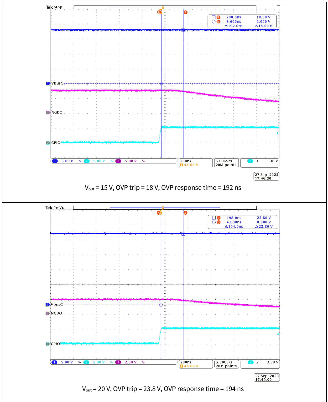
Figure 41 Overvoltage protection trip point and response time at 230 V ac , 50 Hz (CH1: V bus_c , CH2: GPIO9, CH3: NDGO = Provider FET Q2 gate-source)
