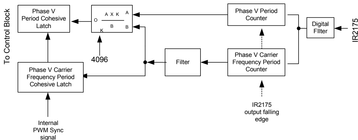
Figure 2. Current Feedback Measurement Block
