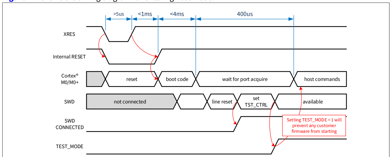
Figure 4-2. Timing diagram of entering test mode
