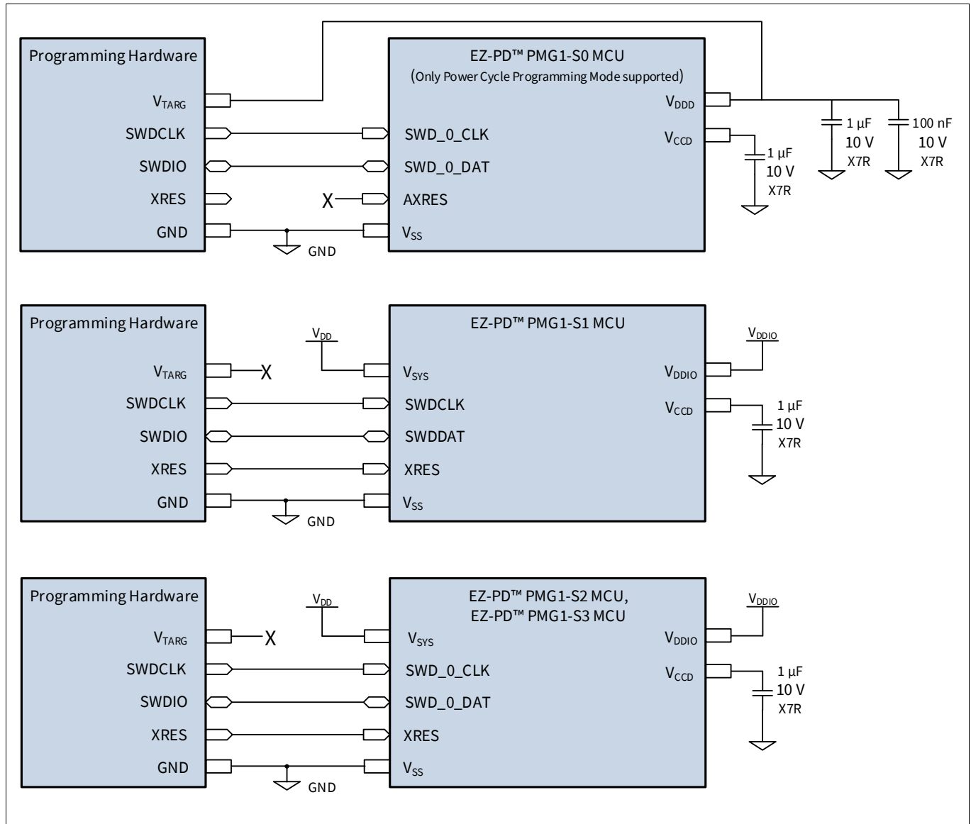
Figure 3-3. Connection schematic of programmer
