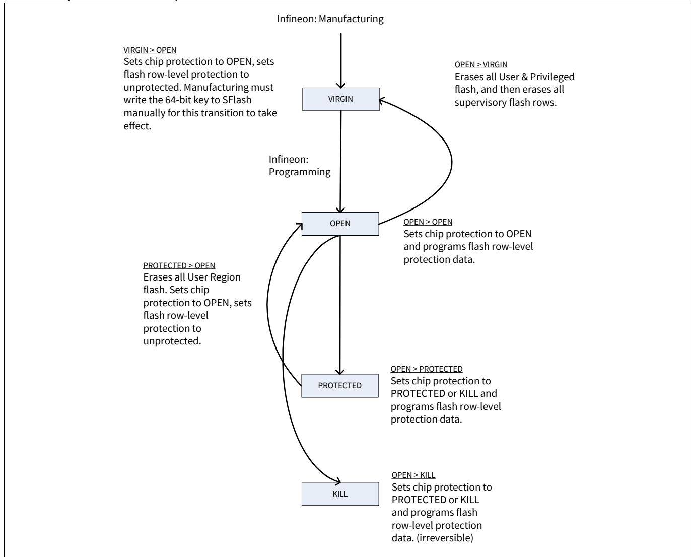
Figure A-1. Chip-level protection mode diagram
