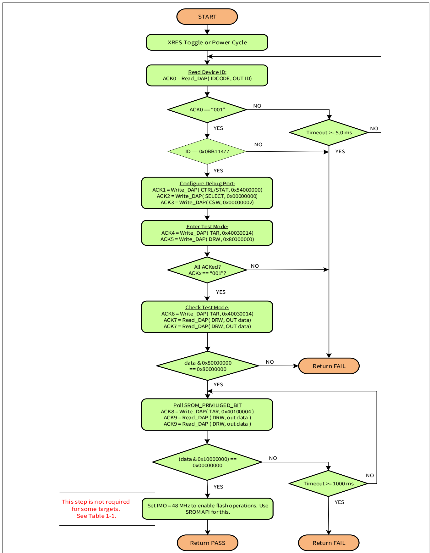
Figure 4-3. Flowchart of the “Acquire chip” step
