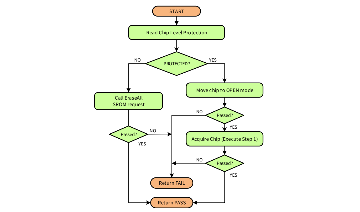
Figure 4-4. Flowchart of the “Erase all” step
