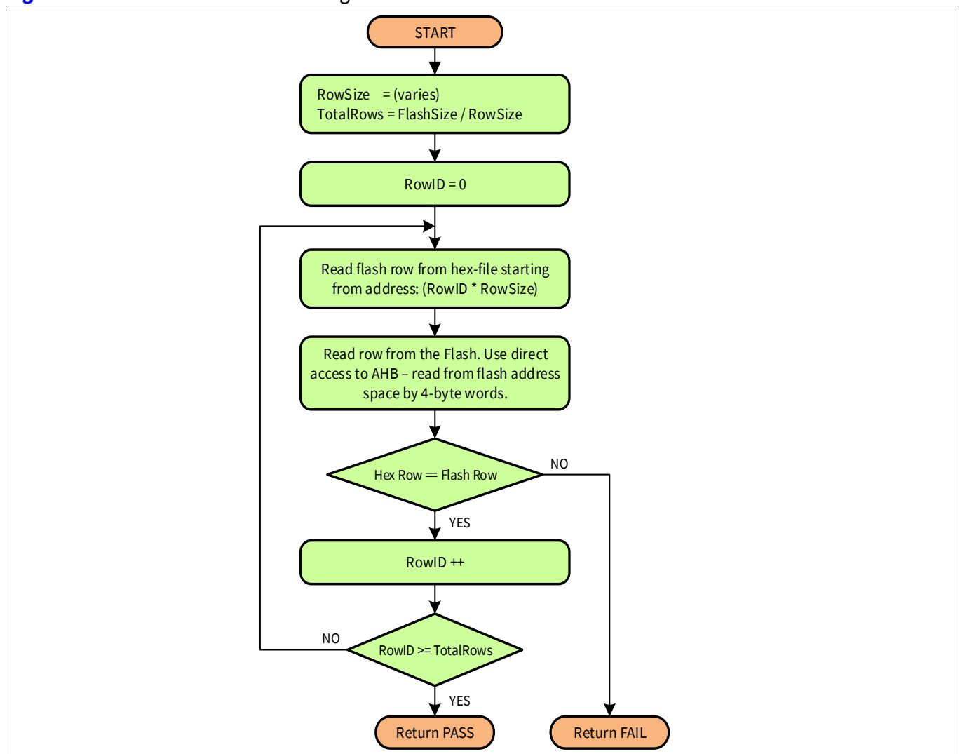
Figure 4-6. Flowchart of the “Verify flash” step
