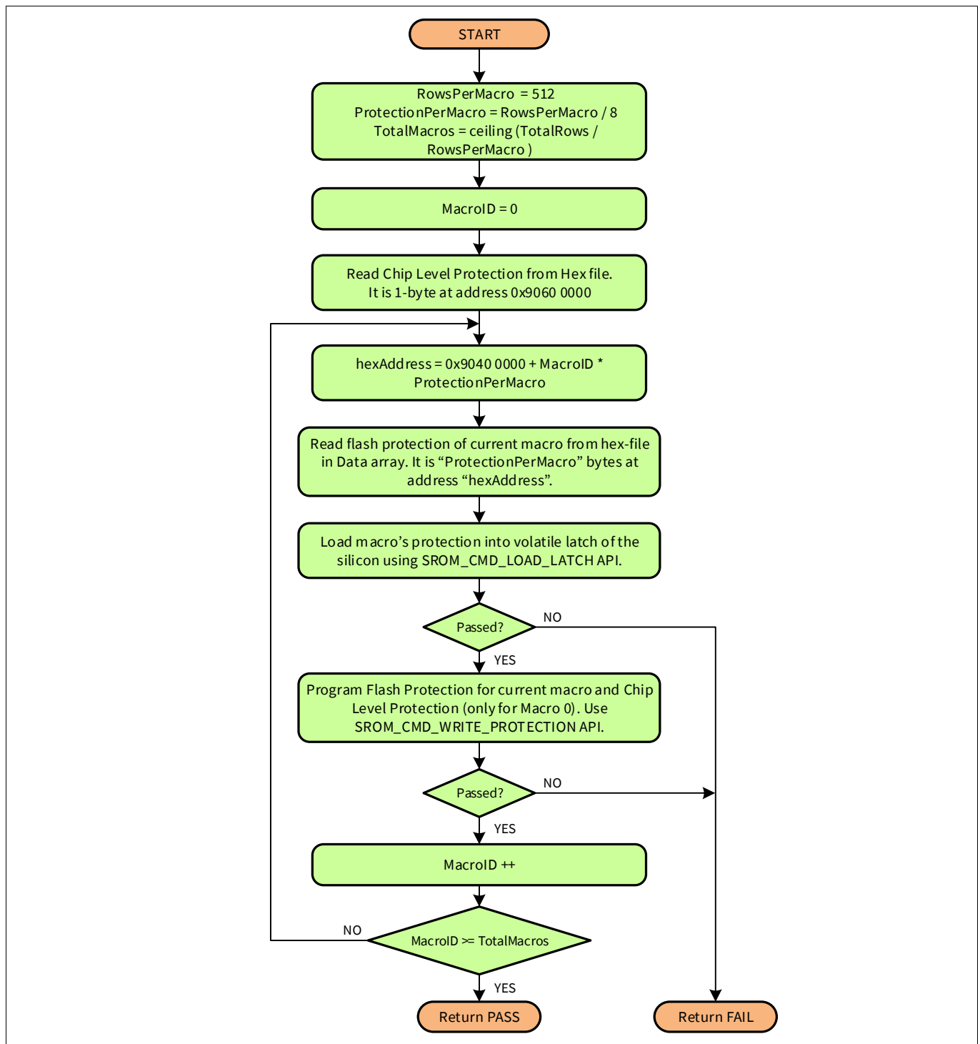
Figure 4-7. Flowchart of the “Program protection settings” step
