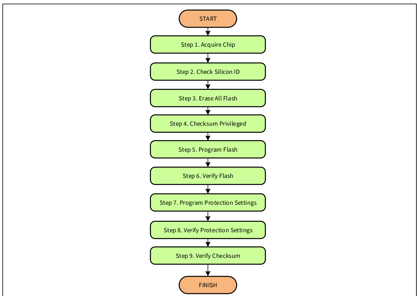
Figure 4-1. High-level programming flow of the target device
