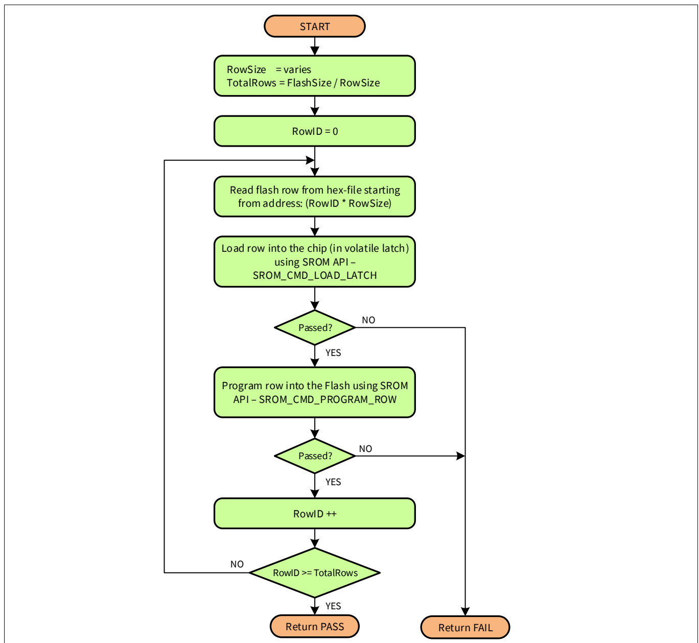
Figure 4-5. Flowchart of the “Program flash” step
