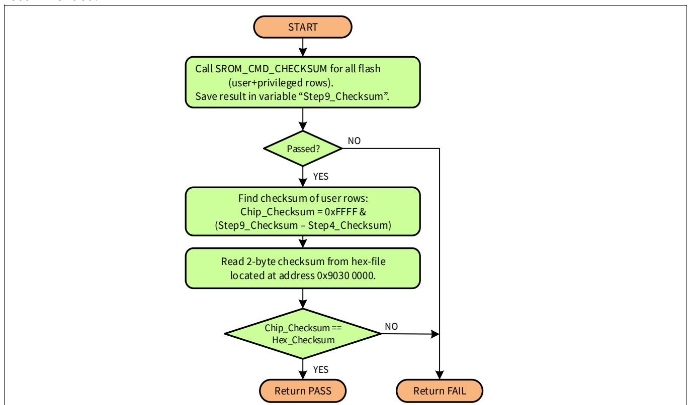
Figure 4-9. Flowchart of the “Verify checksum” step
