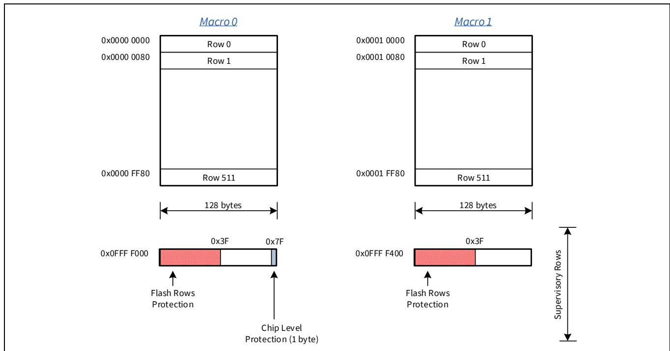
Figure 2-1. A typical nonvolatile subsystem
