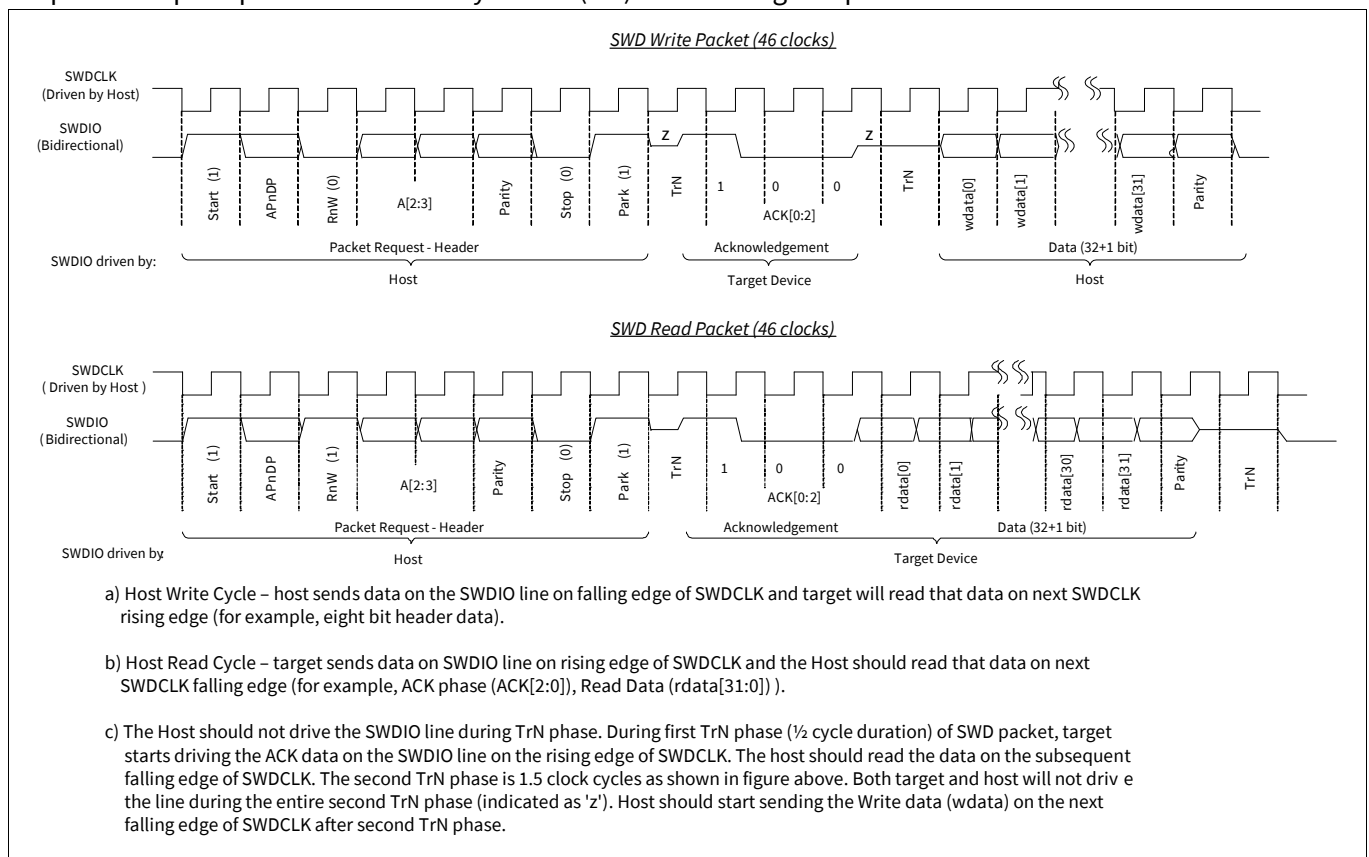
Figure C-1. Write and Read SWD packet timing diagrams
