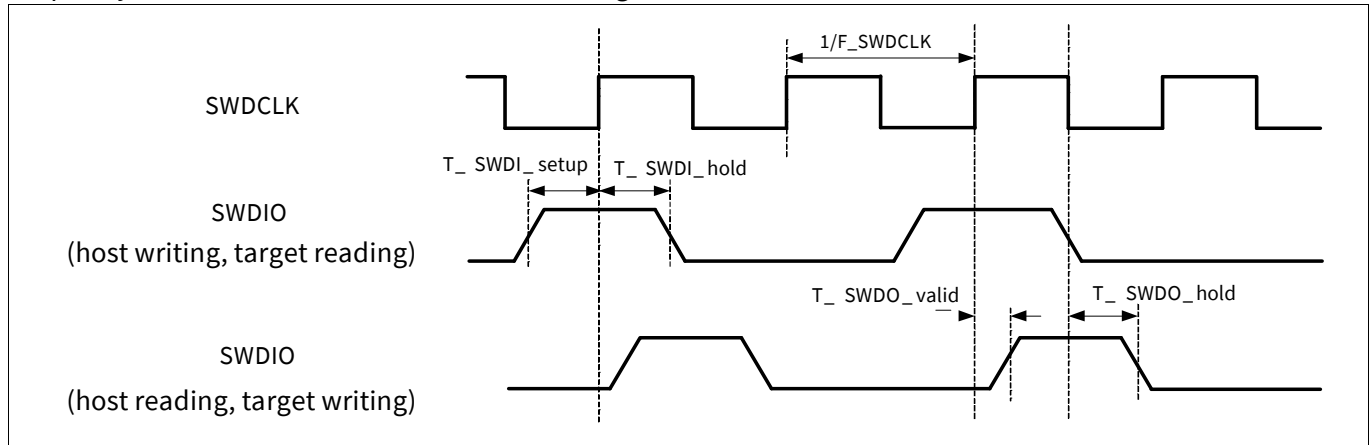
Figure D-1. SWD interface timing diagram
