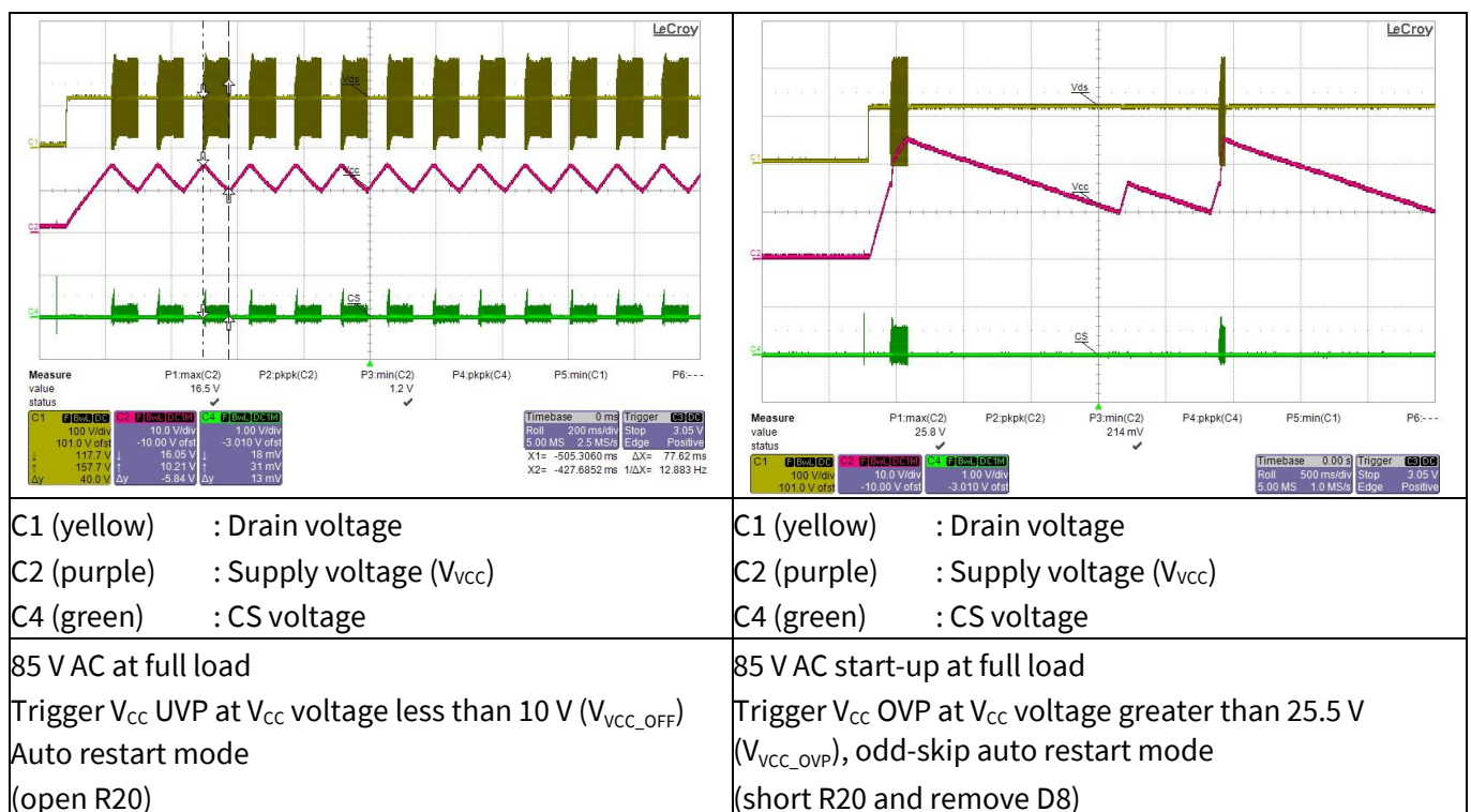
Figure 30 V_{CC} OVP/UV
