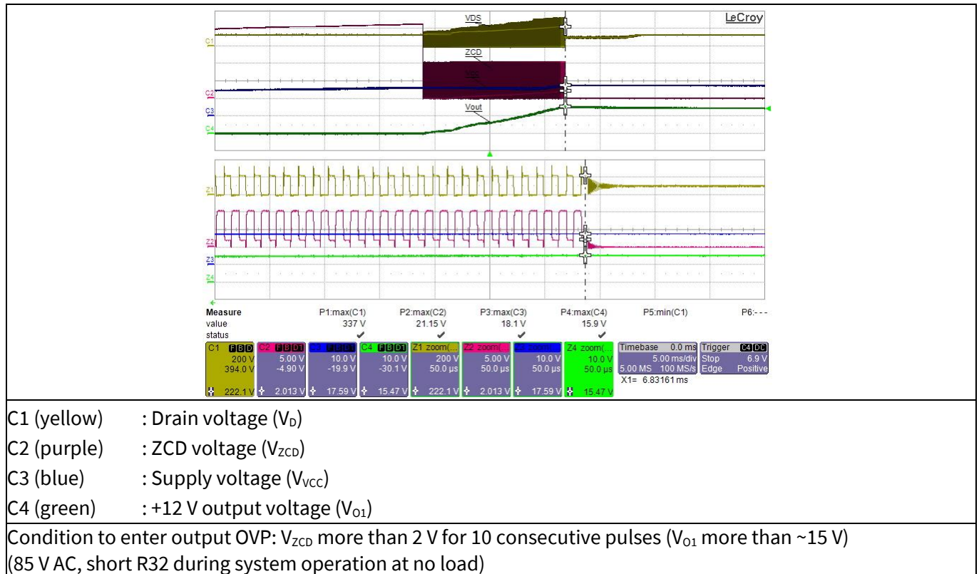
Figure 29 Output OVP
