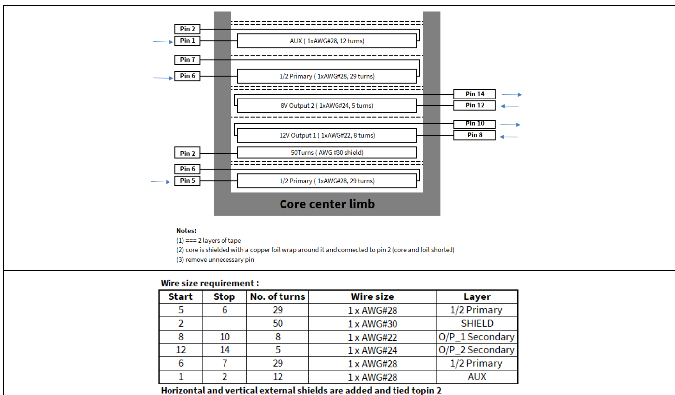
Figure 8 Transformer structure
