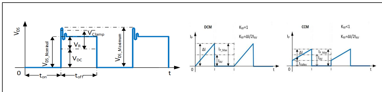
Figure 31 Drain voltage and current waveform
