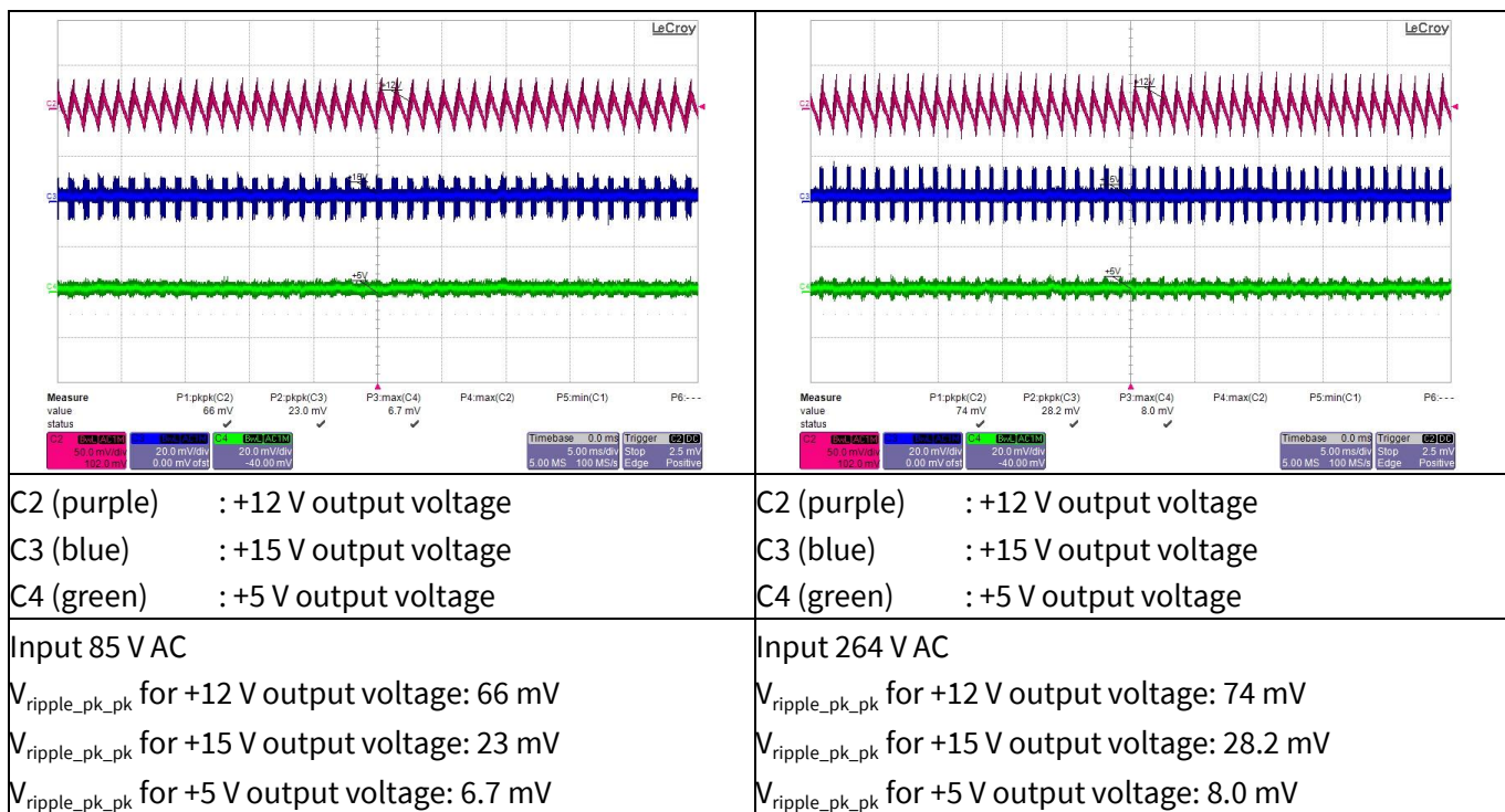
Figure 25 Output ripple voltage at minimum load. Probe terminals are decoupled with 10 \mu F electrolytic and 0.1 \mu F ceramic capacitors. Oscilloscope is bandwidth filter limited to 20 MHz
