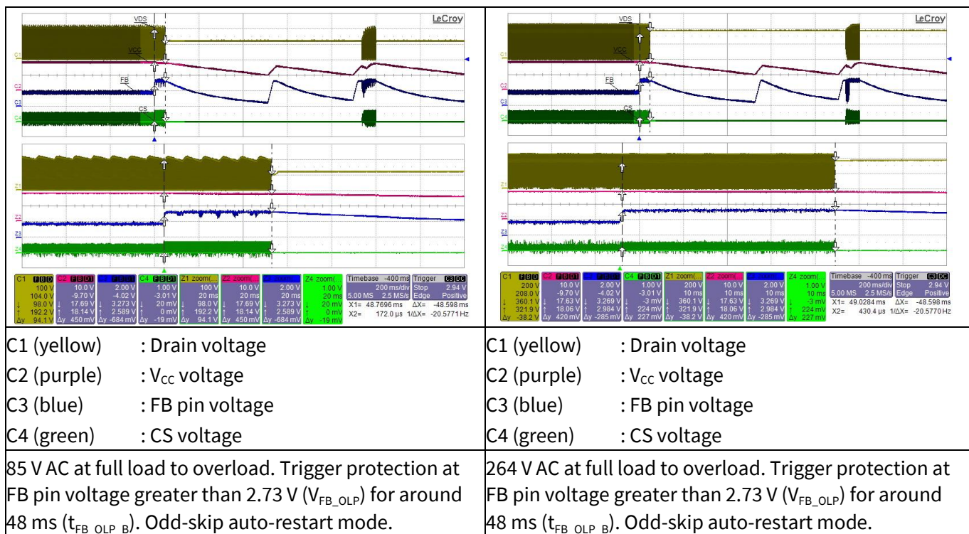
Figure 30 Overload protection
