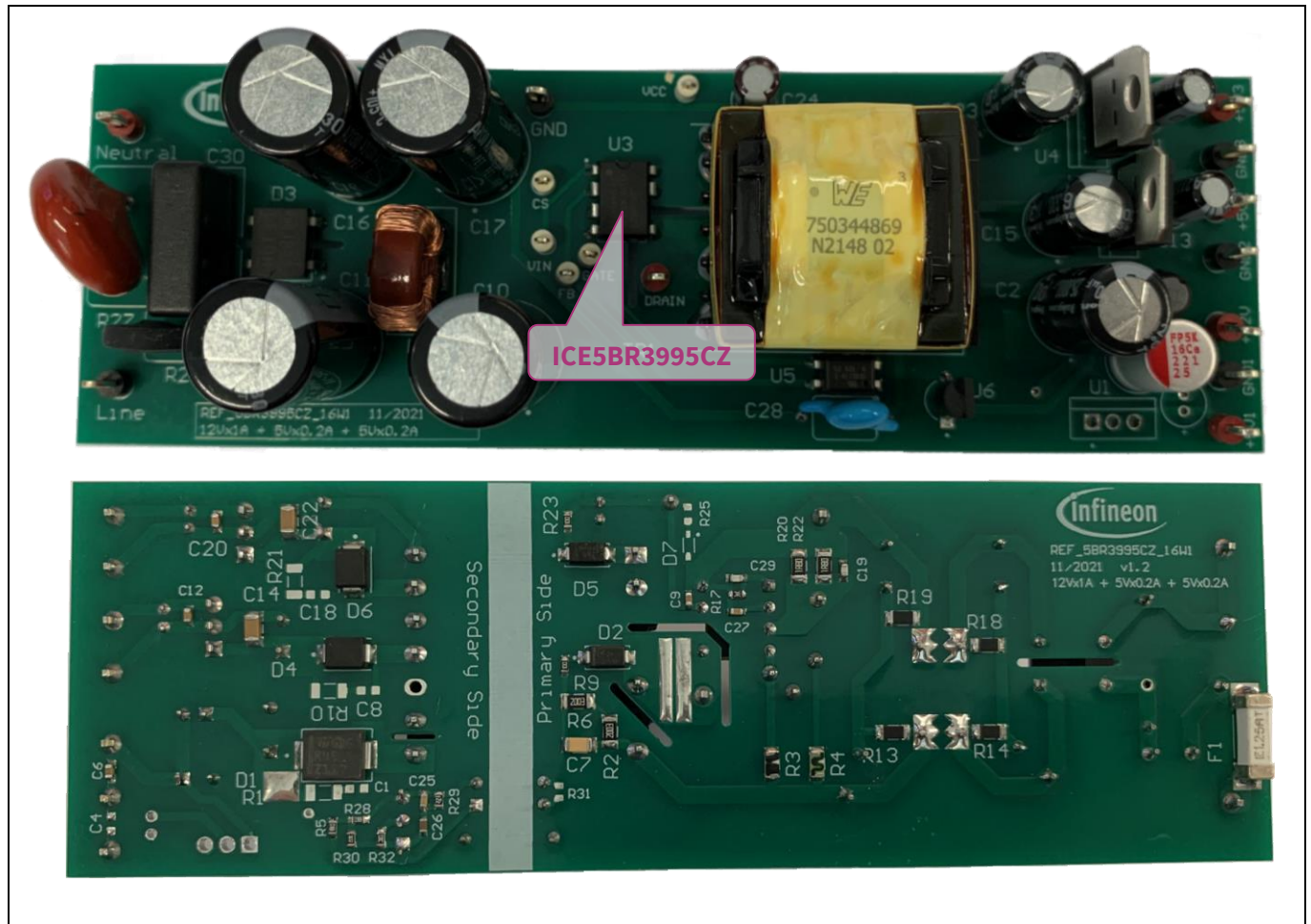
Figure 2 REF_5BR3995CZ_16W1
