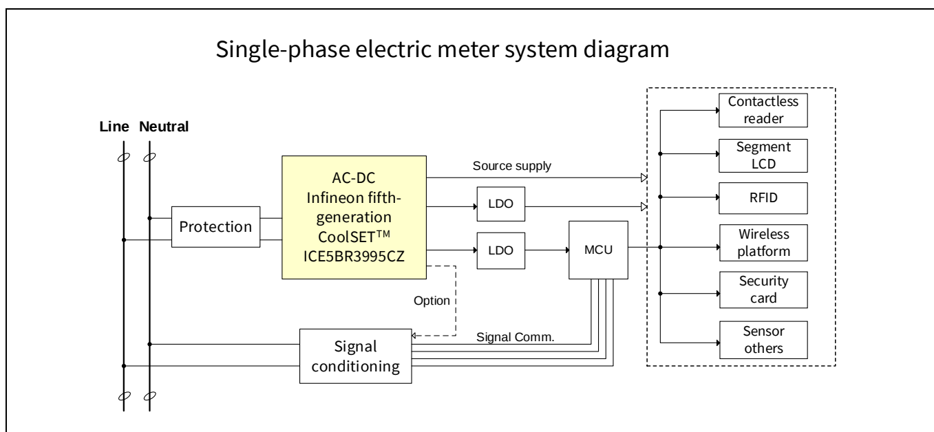
Figure 1 Simplified electric meter system diagram
