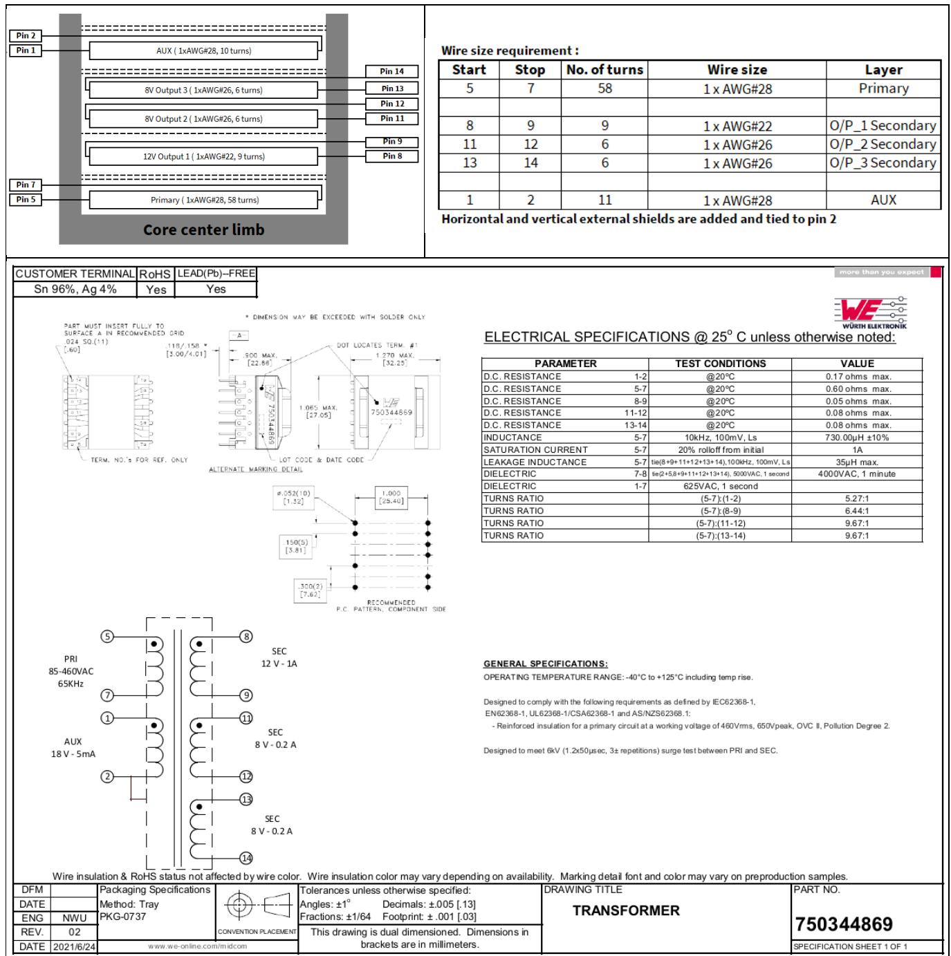
Figure 8 Transformer structure
