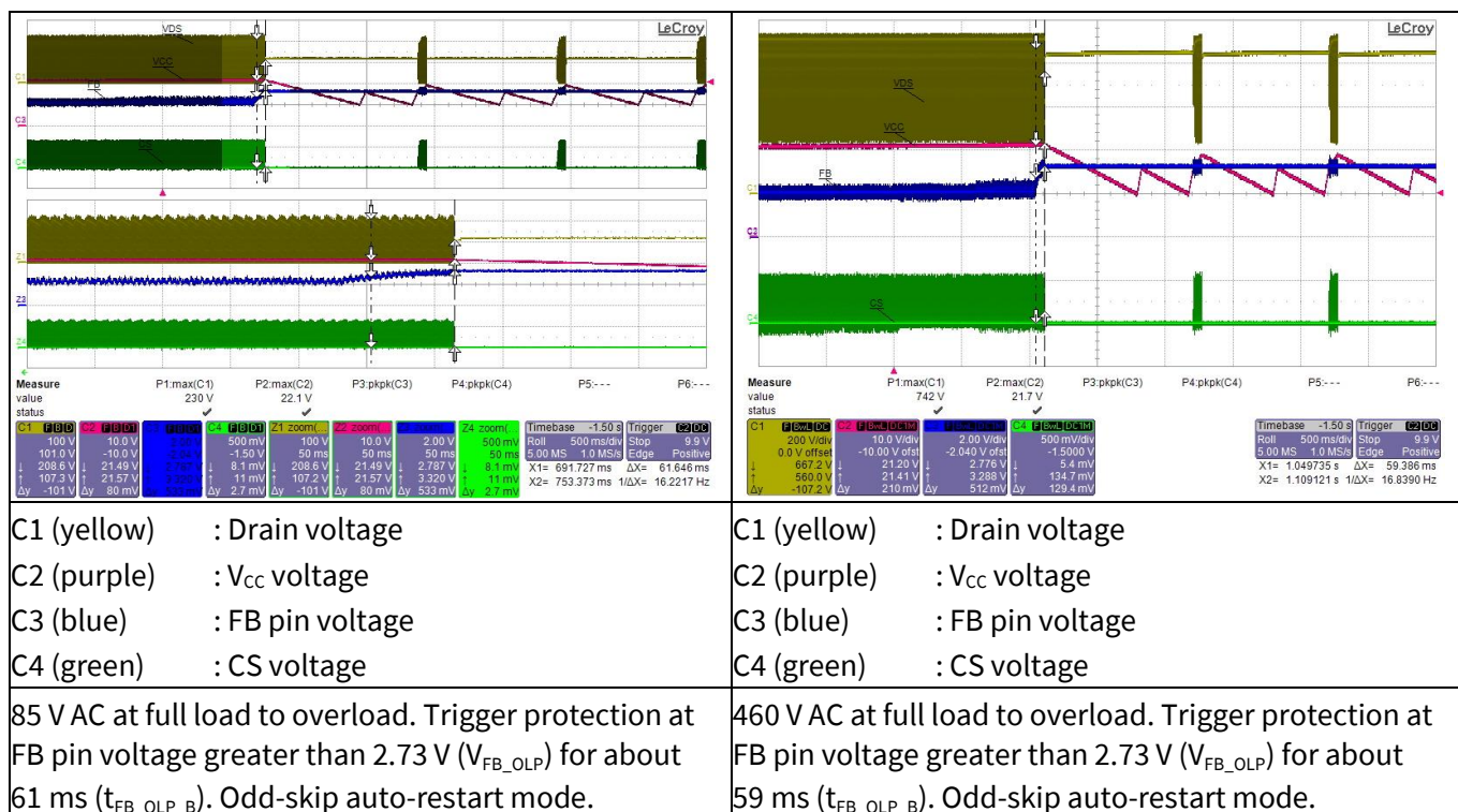
Figure 27 Overload protection
