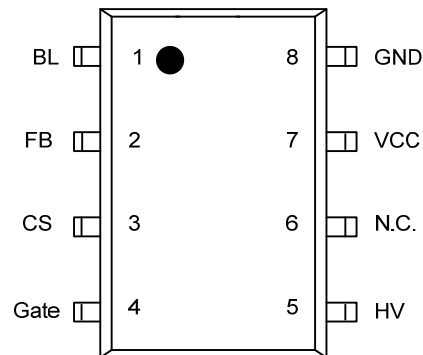
Figure 1 Pin assignment
