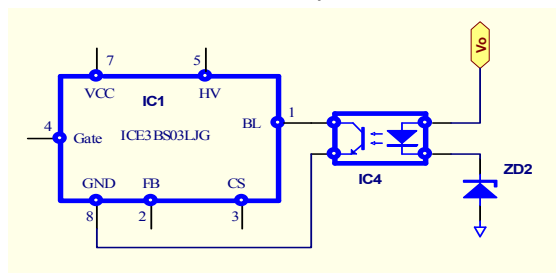
Figure 24 Output OVP circuit
