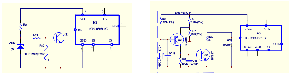
Figure 25 OTP circuit
