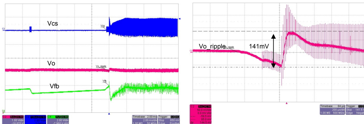
Figure 13 Leaving burst mode waveform; Vfb, Vcs and Vo (left); Vo_ripple (right)
