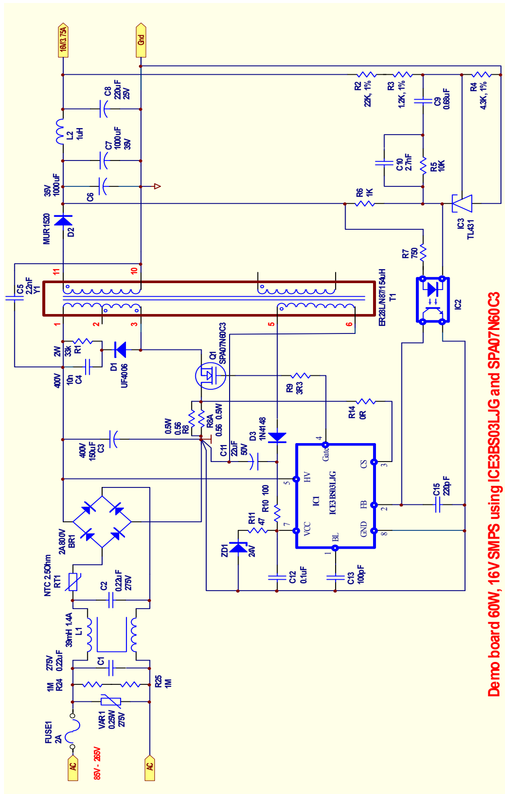
Figure 5 Typical application circuit with ICE3BS03LJG 60W 16V
