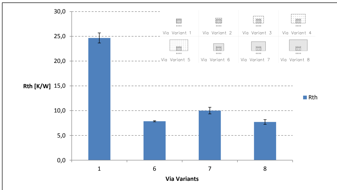
Figure 21 ThinPAK 5x6 V1, V6 to V8 results
