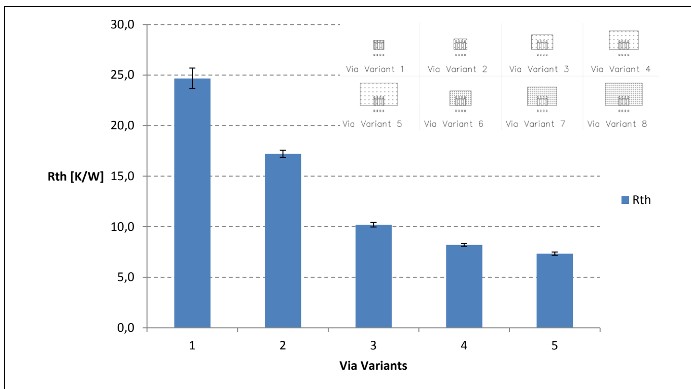
Figure 20 ThinPAK 5x6 V1 to V5 results
