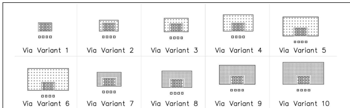
Figure 16 PCB structure ThinPAK 8x8
