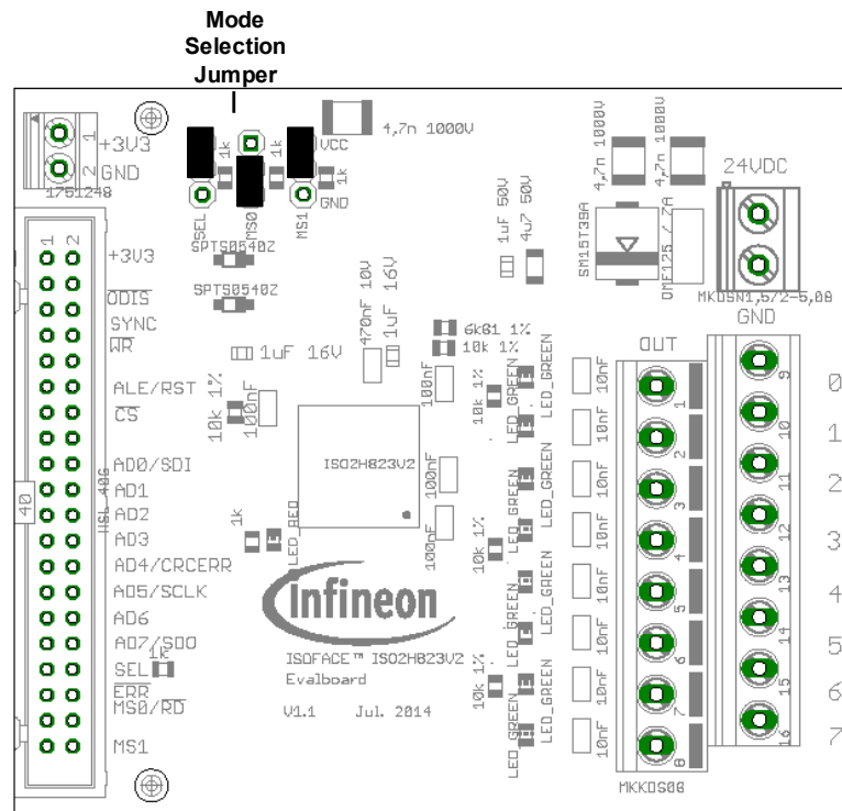
Figure 16 Jumper setting for serial mode 2
