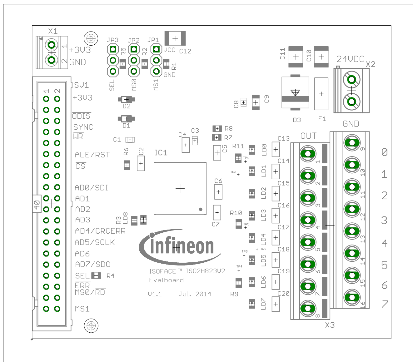
Figure 19 Component Placement
