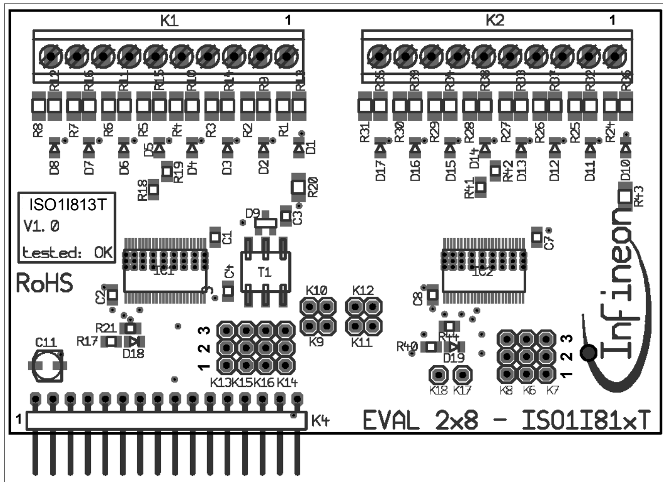
Figure 14 Board Assembly
