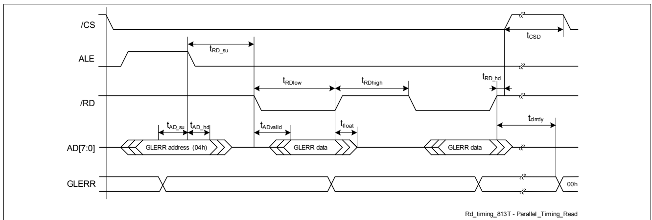
Figure 5 Timing Diagram \mu C Control Mode Read
