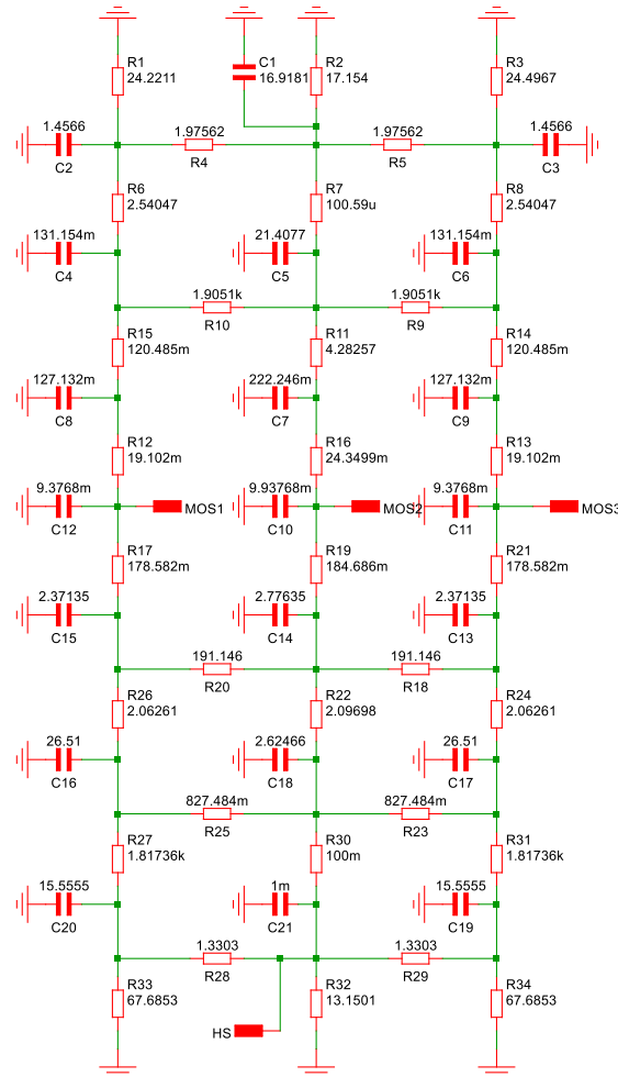
Figure 17 Cauer network of TSC with heatspreader
