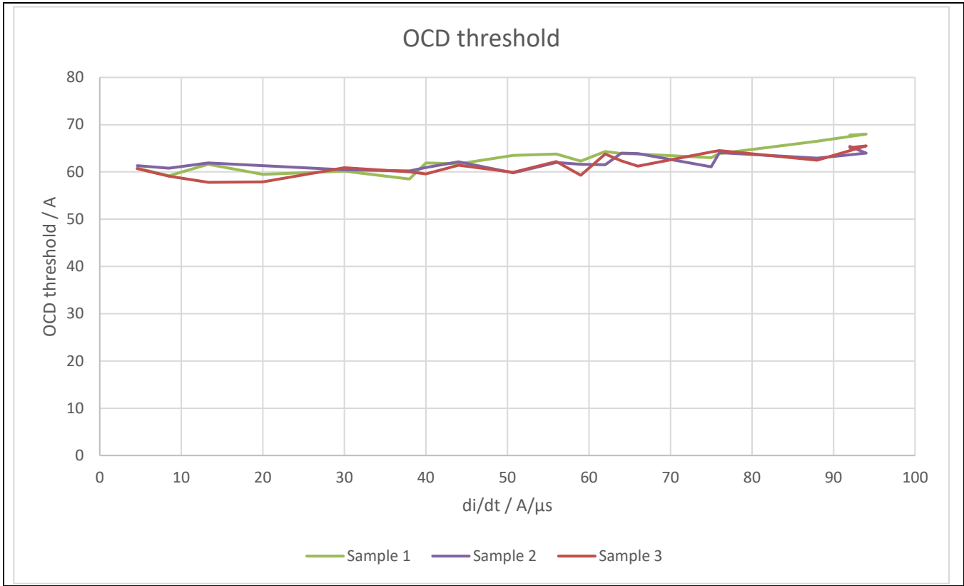
Figure 34 Measurement of optimized OCD threshold
