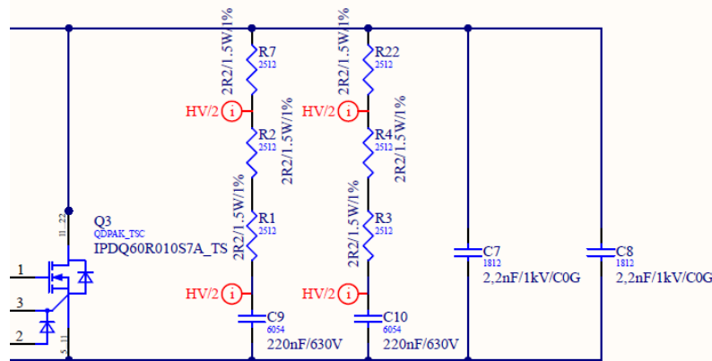
Figure 39 RC snubber design for the eFuse PoC
