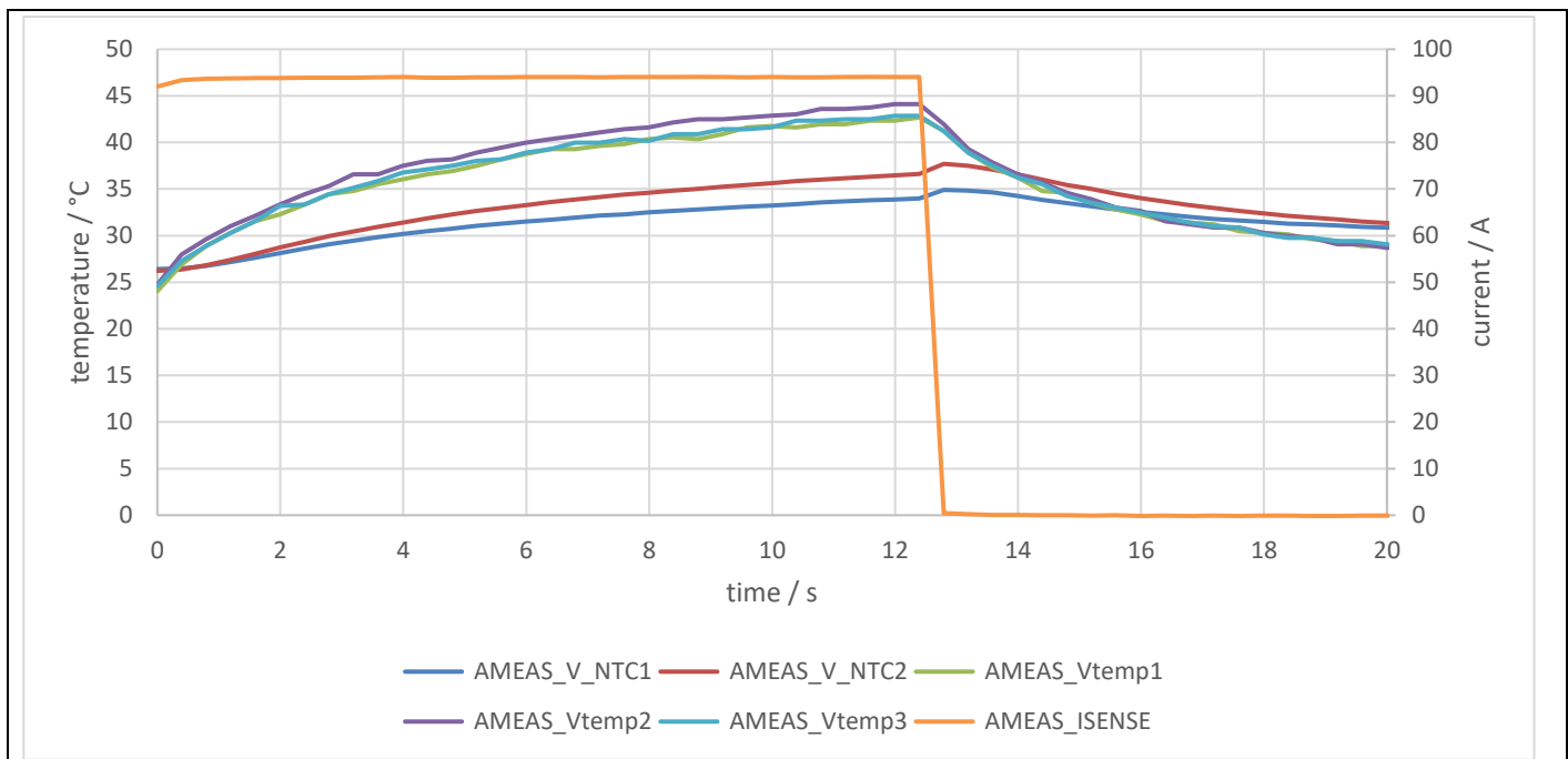
Figure 51 eFuse PoC BSC power stage - 89 A measurement result
