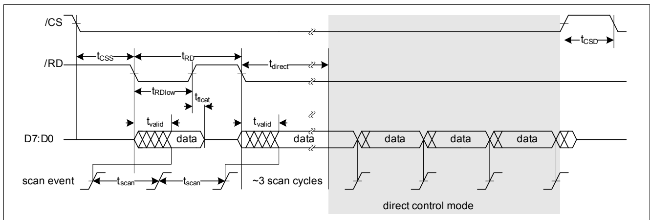
Figure 5 Timing Diagram \mu C Control Mode
