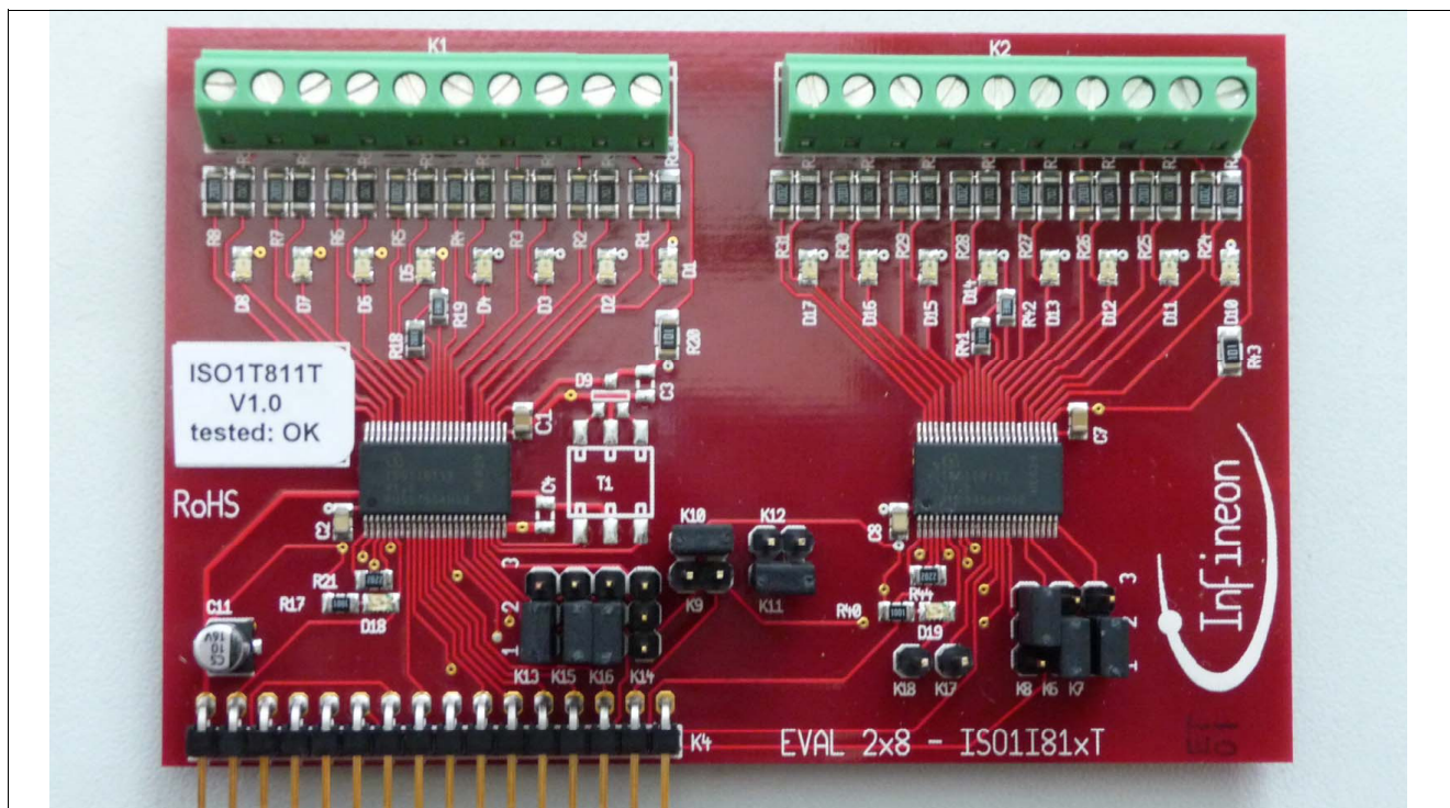
Figure 2 EVAL 2x8-ISO1I811T
