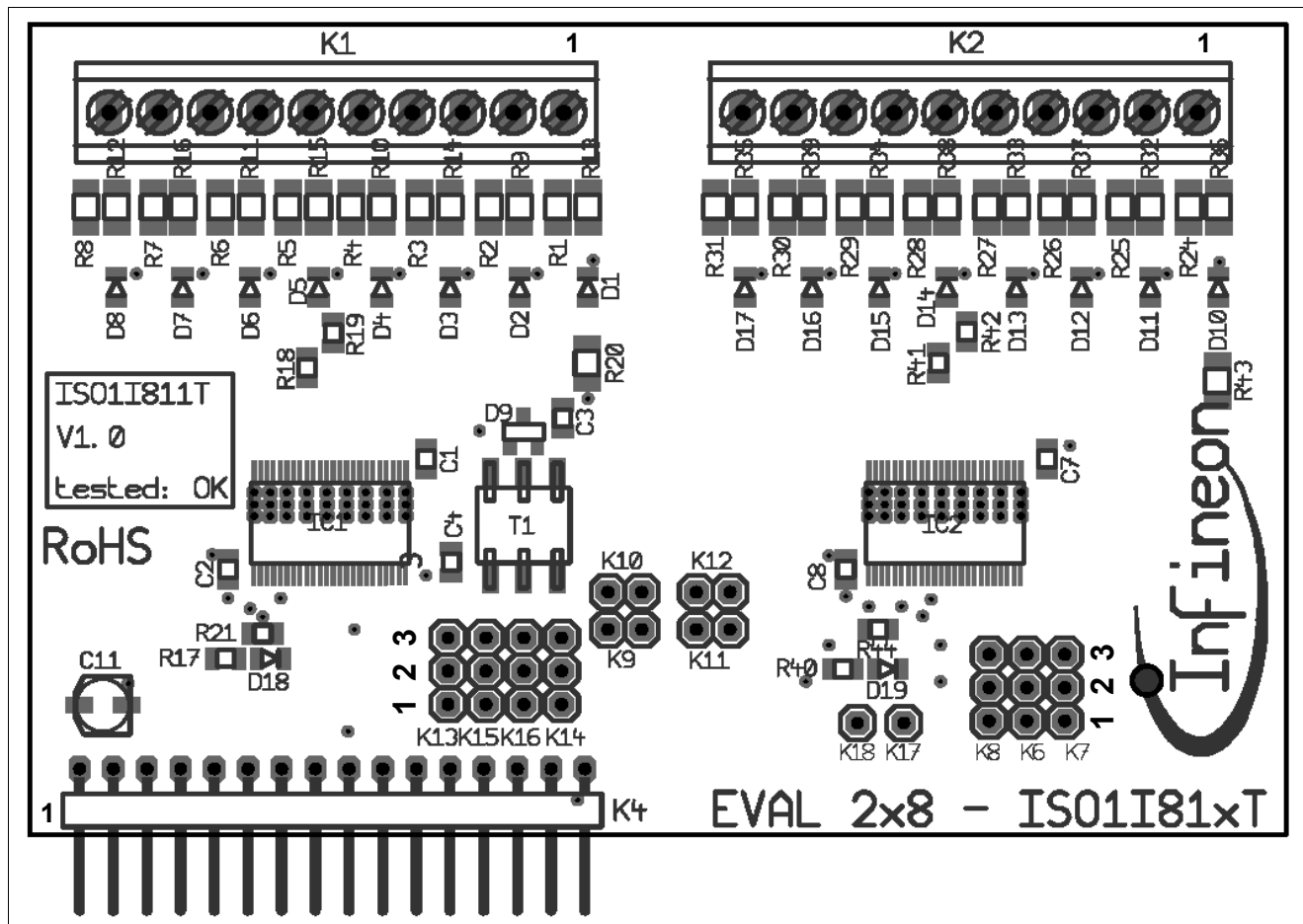
Figure 11 Board Assembly
