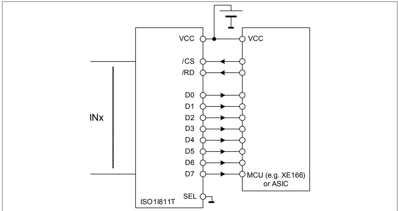
Figure 4 \mu C Control Mode
