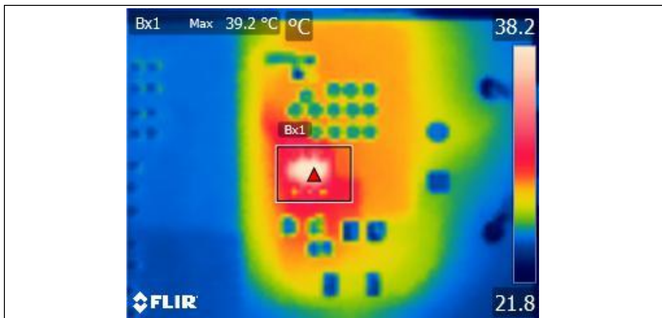
图14 热照片（V IN = 24 V, Rset = 9.1 kΩ, I LED = 68 mA, T A = 25°C）
